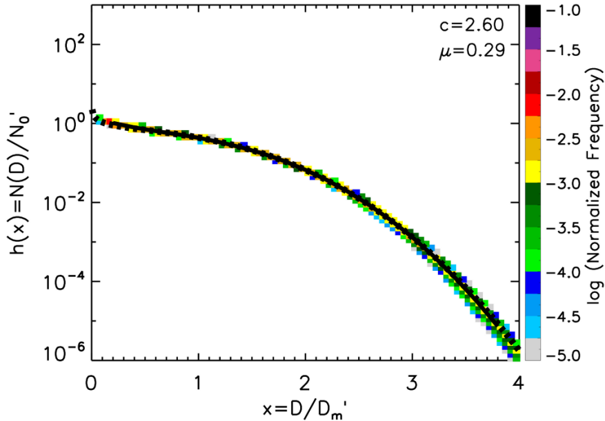
Figure 1: Normalized DSD derived from N'_0(M_0, M_3) and D'_m(M_0, M_3) , along with their h_{\text{mean}(0,3,\mu,c)}(x) from theoretical N_R(D) in Eq. (8) over the Boseong area. Colors indicate the normalized frequency of the normalized DSDs with M_0 and M_3 and the solid line represents h_{\text{mean}(0,3,\mu,c)}(x) for each channel.
