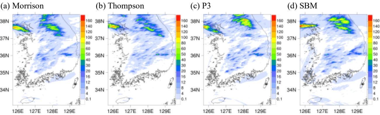
Figure 13: The accumulated surface precipitation (mm) on 6 August 2013 using (a) Morrison, (b) Thompson, (c) P3, and (d) SBM cloud microphysics schemes.
