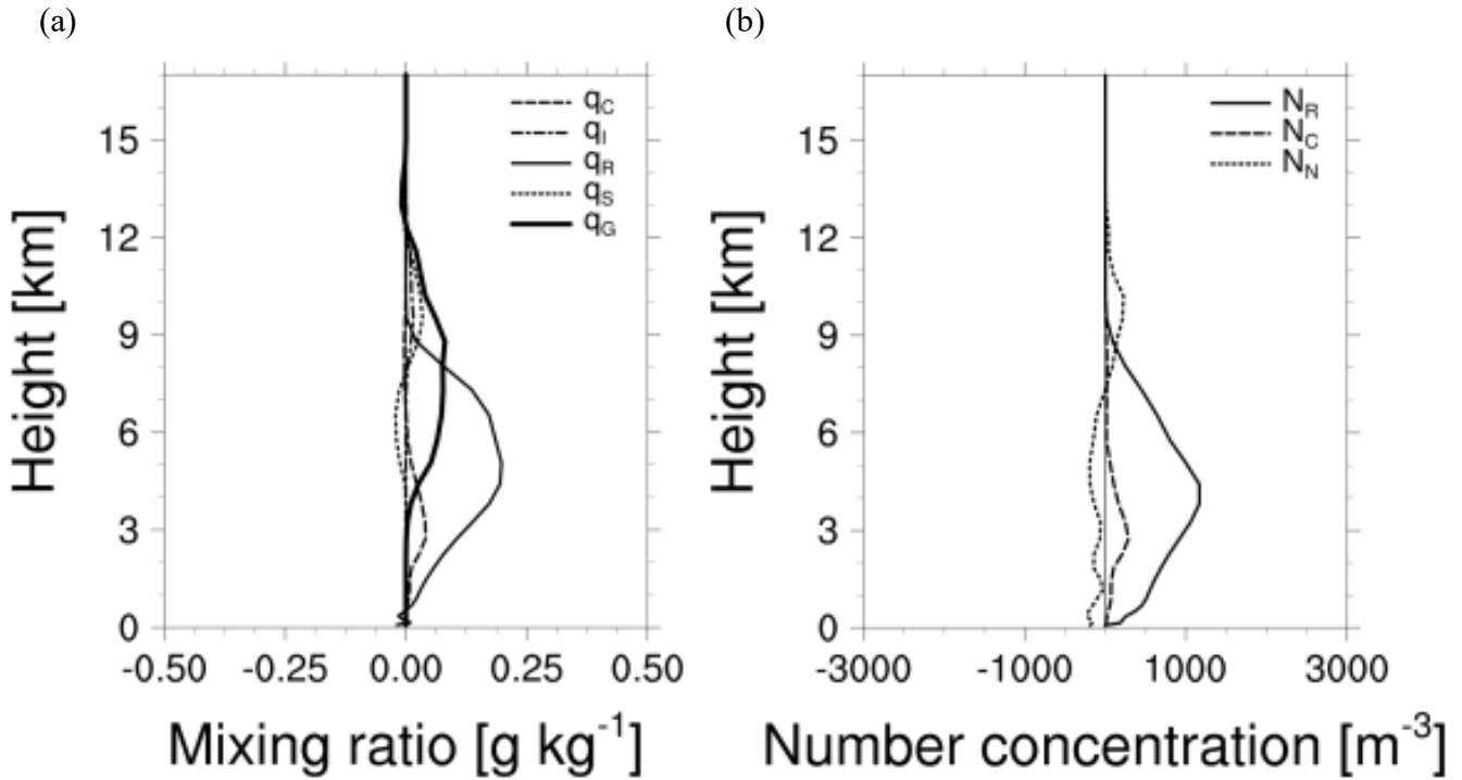
Figure 11: Differences in the time-domain averaged vertical distribution (GDMN minus WDM6) over the region denoted by the red dashed box in Fig. 3b for (a) mixing ratio ( \text{g kg}^{-1} ) and (b) number concentration ( \text{m}^{-3} ) between 06:00 and 08:00 UTC on 6 August 2013.
