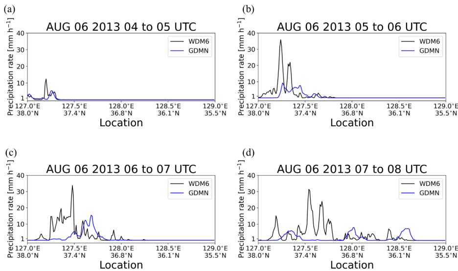
Figure 8: 1-hour accumulated surface precipitation along the cross-sectional area indicated by the red solid line in Fig. 3b for (a) 04:00 to 05:00 UTC, (b) 05:00 to 06:00 UTC, (c) 06:00 to 07:00 UTC, and (d) 07:00 to 08:00 UTC on 6 August 2013. Black and blue lines represent WDM6 and GDMN, respectively.
