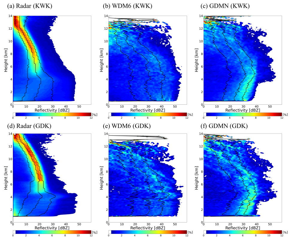
Figure 7: Contoured Frequency by Altitude Diagram percentiles at the KWK and GDK radar sites (location shown in Fig. 3b) for (a) radar observations, (b) WDM6, and (c) GDMN at the KWK site during the analysis period. Panels (d)–(f) are the same as (a)–(c) but at the GDK site. Solid lines denote the cumulative reflectivity frequencies at the 25th, 50th, and 75th percentiles.
