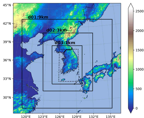
Figure 34: The model domain, consisting of three nested domains with resolutions of 9 km (d01), 3 km (d02), and 1 km (d03). Shading indicates the terrain height in meters above sea level. The analysis domain is denoted by the black dotted line within the innermost domain (d03).
