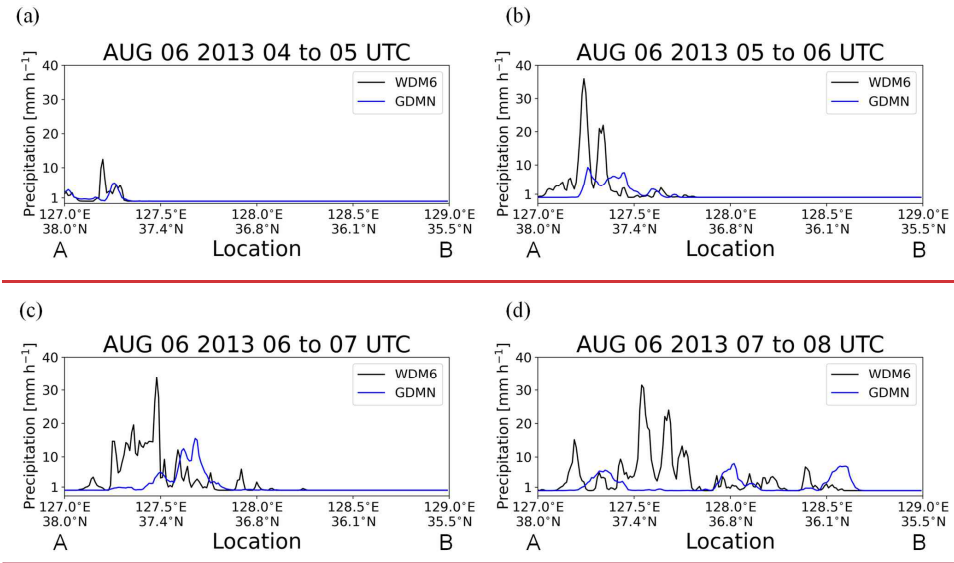
Figure 8: 1-hour accumulated surface precipitation along the cross-sectional area indicated by the red solid line in Fig. 2b3b for (a) 04:00 to 05:00 UTC, (b) 05:00 to 06:00 UTC, (c) 06:00 to 07:00 UTC, and (d) 07:00 to 08:00 UTC on 6 August 2013. Black and blue lines represent WDM6 and GDMN, respectively.
