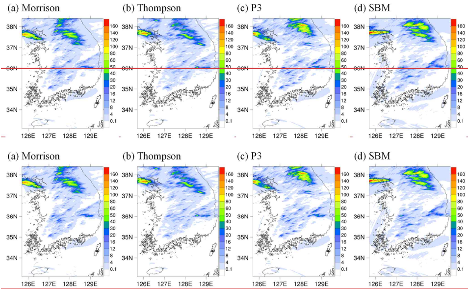
485 Figure 13: The accumulated surface precipitation (mm) on 6 August 2013 using (a) Morrison, (b) Thompson, (c) P3, and (d) SBM cloud microphysics schemes.
