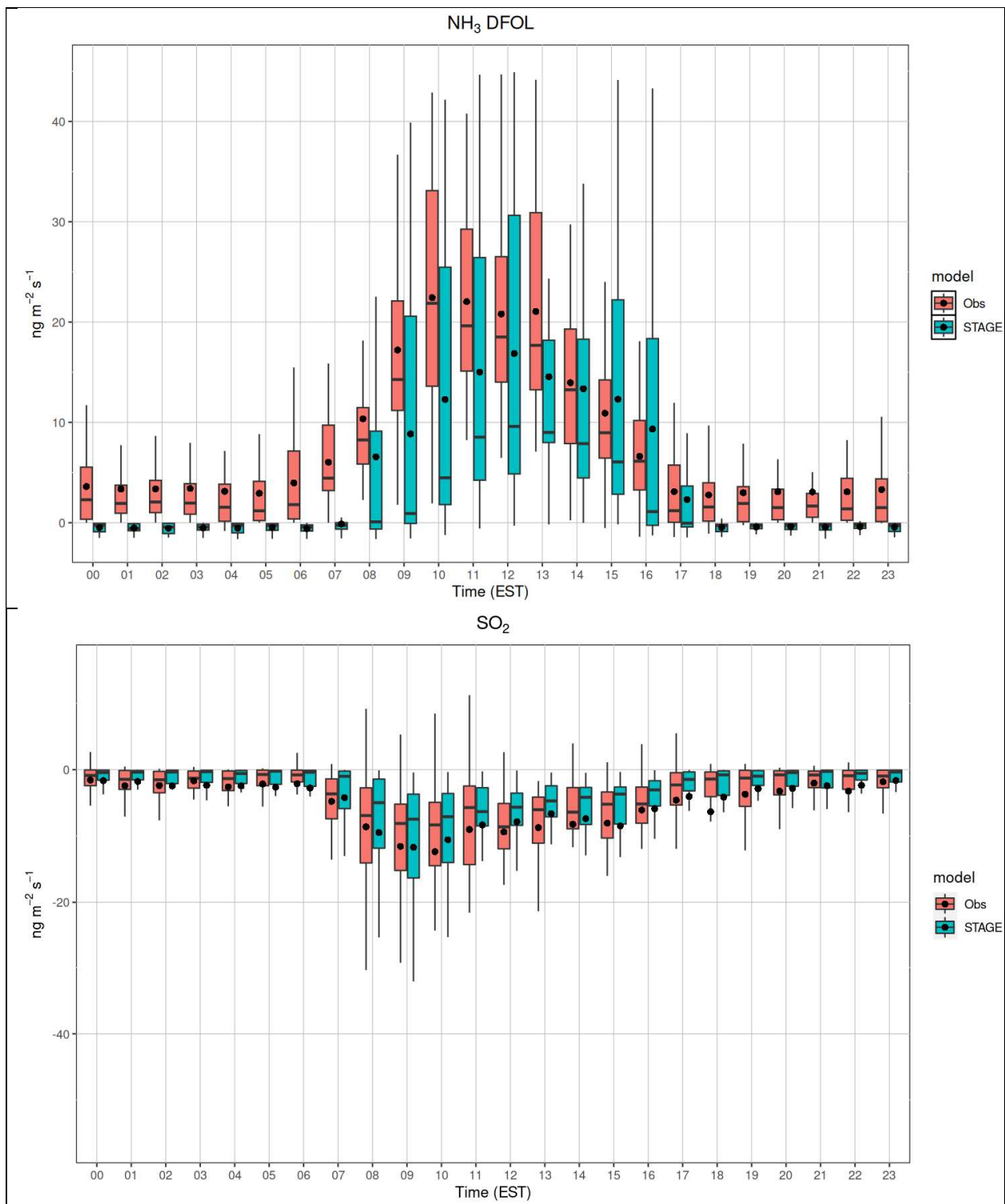
Figure 2. STAGE model estimates (blue) and observations (red) of the HNO 3 (a), NH 3 (b), and SO 2 (c) flux measurements taken at the Duke Forest grasslands flux tower. The box bounds the 25 th to 75 th percentiles, the lines extend to the 5 th and 95 th percentile, the black horizontal line is the median and the black point represents the mean of the modeled or observed hourly values. Note that negative values indicate net deposition and positive values indicate net evasion.
