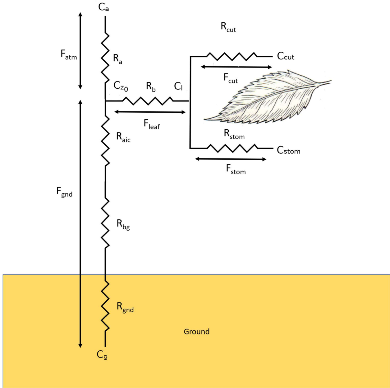
Figure 1. STAGE resistance wire diagram modified from Nemitz et al. 2001 to include non-zero compensation points for leaf cuticular surfaces. Leaf image adapted from Pearson Scott Foresman / Public domain https://commons.wikimedia.org/wiki/File:Acuminate_Leaf_(PSF).jpg
