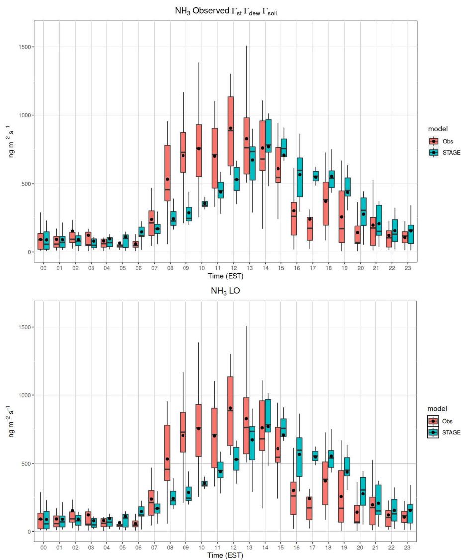
Figure 3, STAGE model estimates (blue) and observations (red) of NH 3 flux measurements taken at the Lillington, NC flux tower over a fertilized corn canopy. The box bounds the 25 th to 75 th percentiles, the lines extend to the 5 th and 95 th percentile, the black horizontal line is the median and the black point represents the mean of the modeled or observed hourly values.
