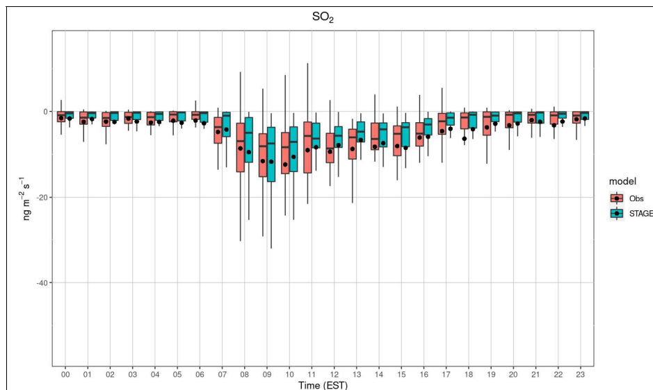
Figure 2. STAGE model estimates (blue) and observations (red) of the HNO 3 (a), NH 3 (b), and SO 2 (c) flux measurements taken at the Duke Forest grasslands flux tower. The box bounds the 25 th to 75 th percentiles, the lines extend to the 5 th and 95 th percentile, the black horizontal line is the median and the black point represents the mean of the modeled or observed hourly values. Note that negative values indicate net deposition and positive values indicate net evasion.
