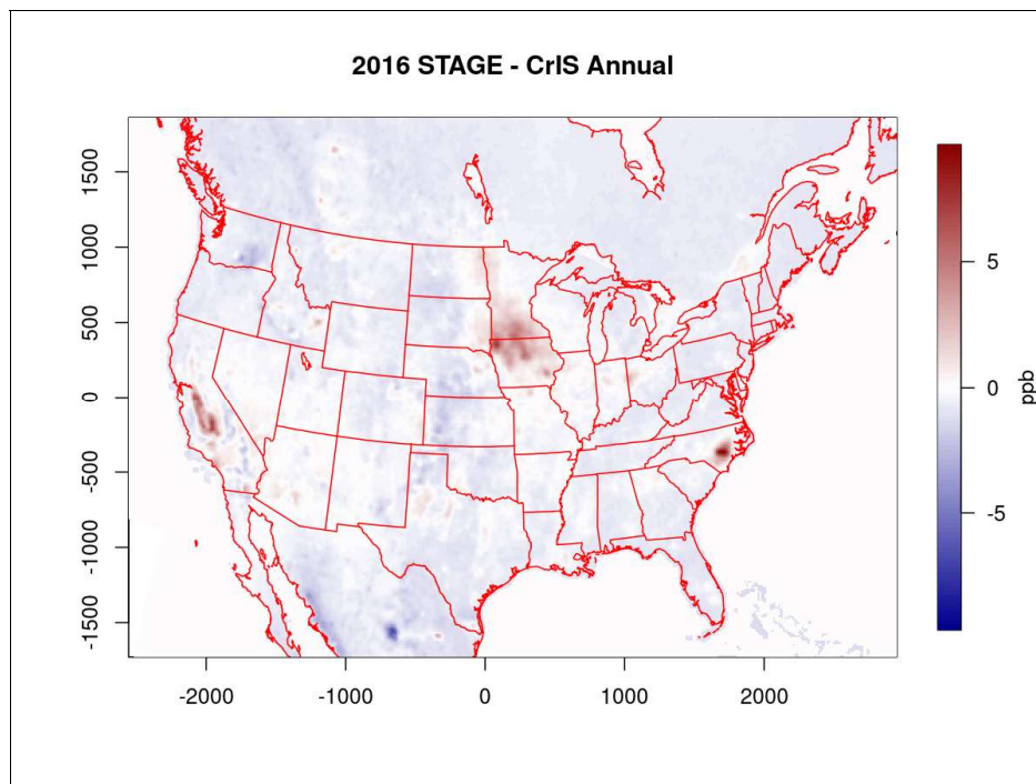
Figure 4, Annual mean Cross Infrared Sounder (CrIS) satellite surface \text{NH}_3 observations binned to CMAQ grid cells for 2016 (Top), mean CMAQ surface \text{NH}_3 estimates paired in space and time with CrIS observations for 2016 (Middle), the mean difference between CMAQ estimates and CrIS observations of \text{NH}_3 paired in space and time for 2016 (Bottom).
