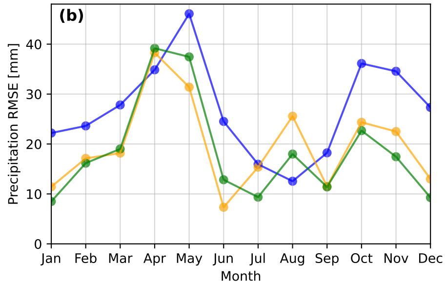
Spatial RMSE of mean monthly near-surface air temperature Spatial RMSE of mean monthly total precipitation
