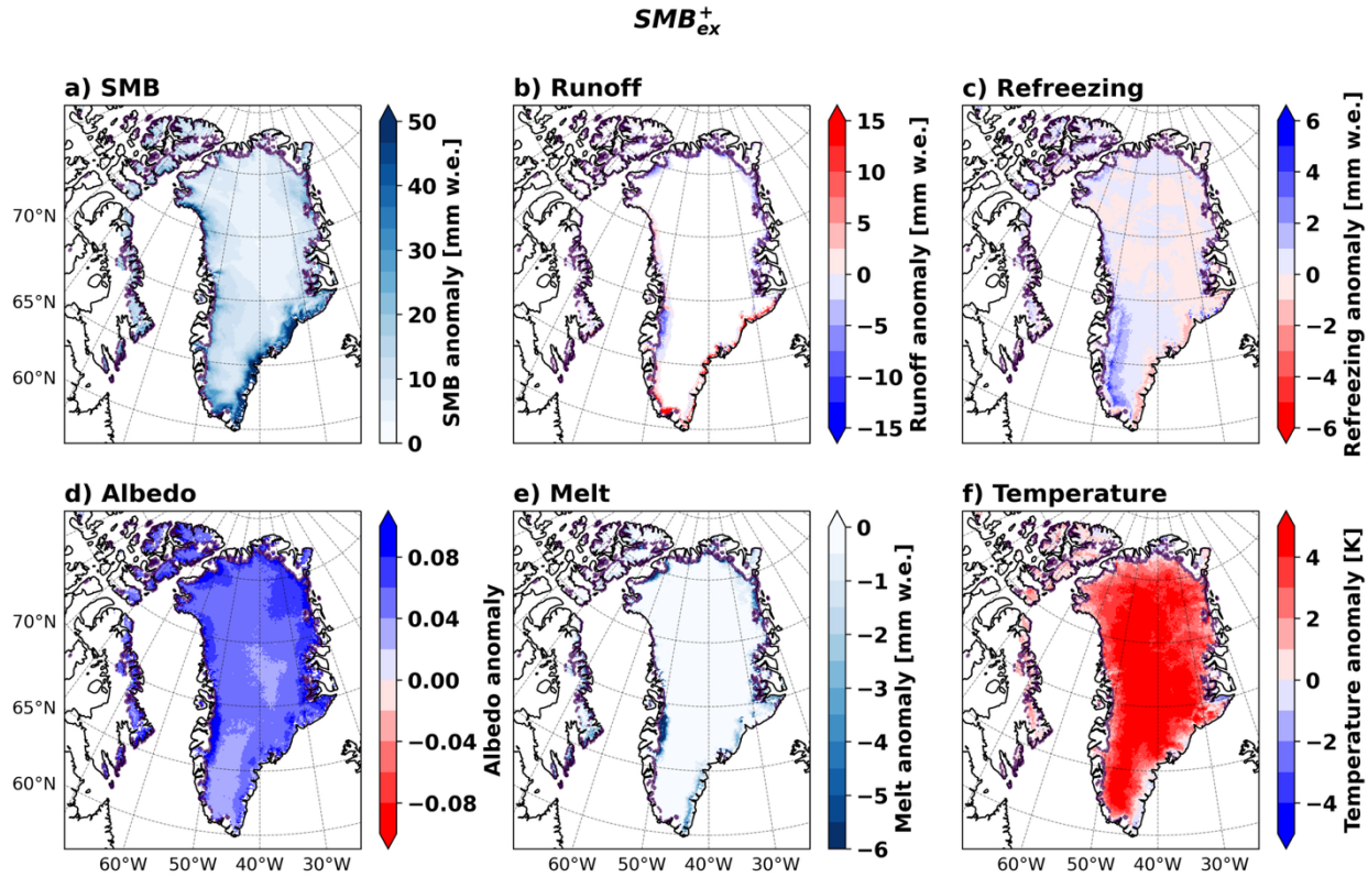
375 Figure 9. Mean anomalies on positive SMB JJAS extreme precipitation days in the historical period (1980-1998) from RACMO. Anomalies are calculated for the extreme precipitation day relative to \pm 15 days surrounding the extreme precipitation day. The solid purple line denotes the top of the ablation zone for the full simulation period. Blue colours in each panel indicate anomalies that act to increase SMB.
