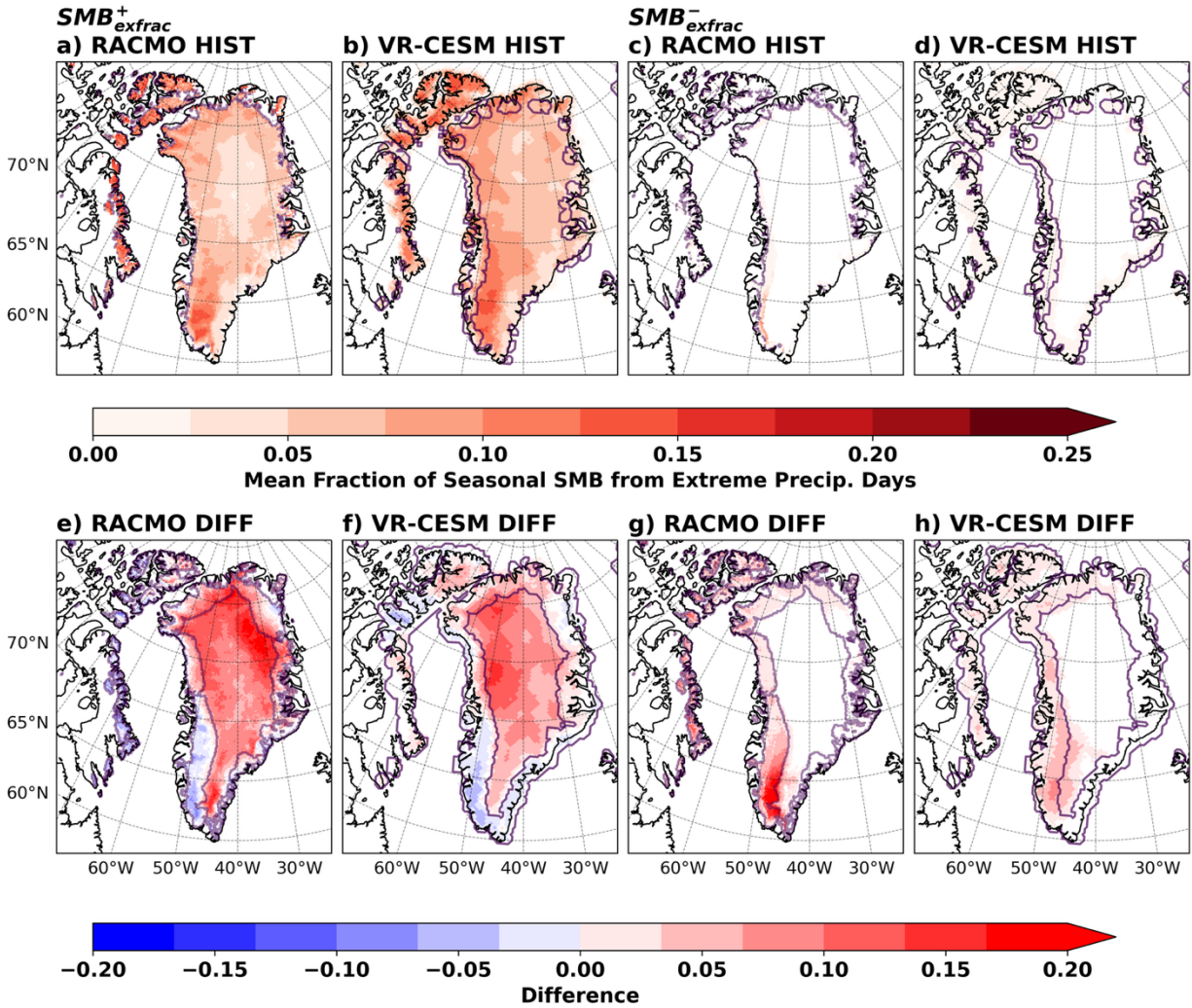
Figure 8. Mean JJAS SMB_{exfrac}^+ (a-b, e-f) and SMB_{exfrac}^- (c-d, g-h) for HIST (1980-1998; a-d) and projected changes (FUT (2080-2098) - HIST; e-h) from RACMO (a, c, e, g) and VR-CESM (b, d, f, h). The solid purple line denotes the top of the ablation zone for the full simulation period, with the future ablation zone being shown on the DIFF panels (e-h).
