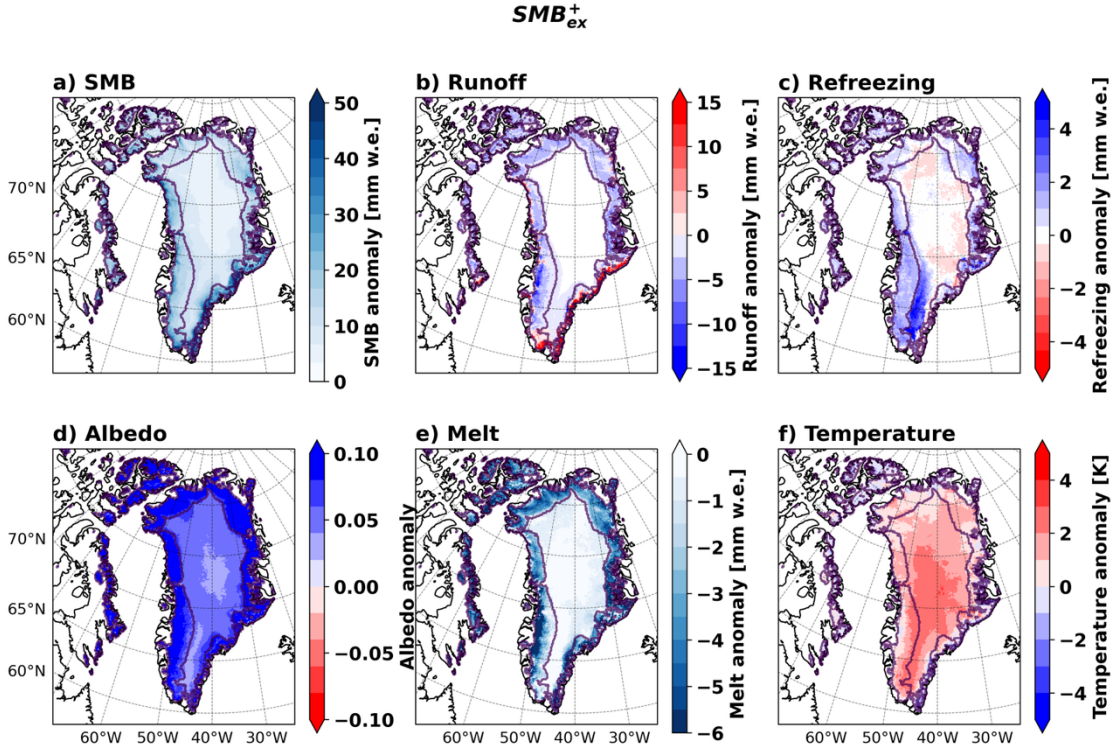
Figure 10. As in Fig. 9, but for future (2080-2098) positive SMB JJAS extreme precipitation days from RACMO.
