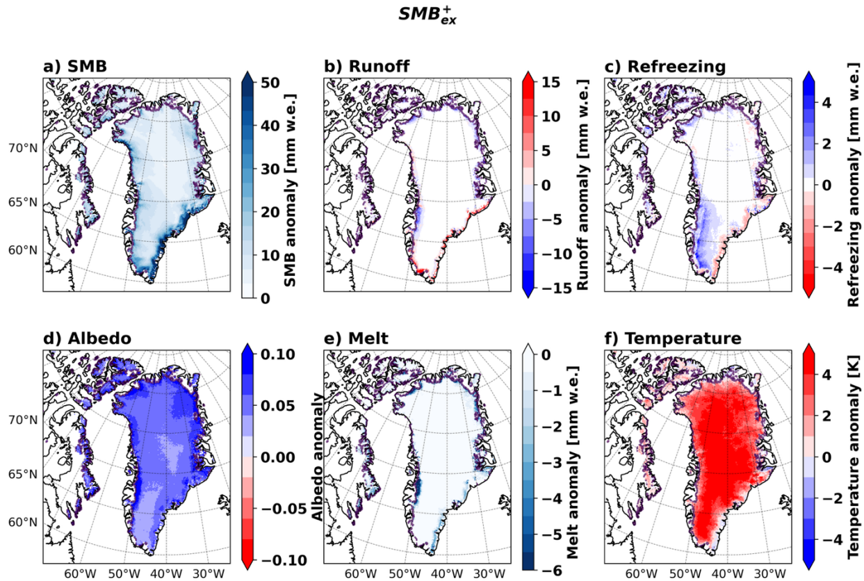
375 Figure 9. Mean anomalies on positive SMB JJAS extreme precipitation days in the historical period (1980-1998) from RACMO. Anomalies are calculated for the extreme precipitation day relative to \pm 15 days surrounding the extreme precipitation day. The solid purple line denotes the top of the ablation zone for the full simulation period. Blue colours in each panel indicate anomalies that act to increase SMB.
