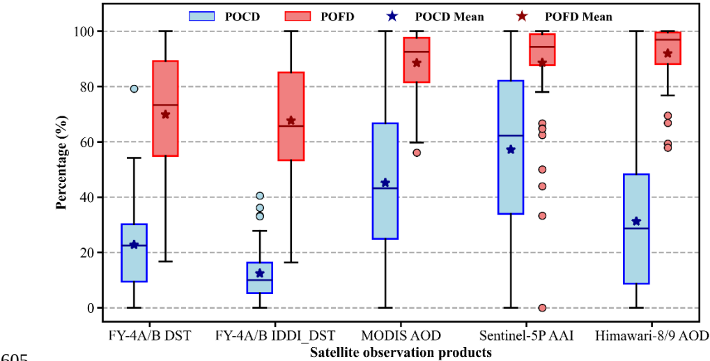
Figure 12. The POCD and POFD of different satellite products for atmospheric dust for every dust events.
