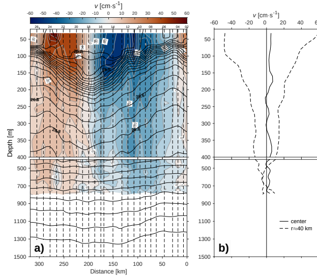
Figure 4. a) Vertical section of cross-transect velocities ( v ) from VMADCP measurements along the OcéT transect. Grey contours represent velocity levels at 5 \text{ cm} \cdot \text{s}^{-1} intervals, while black contours show isopycnals ( \sigma_\theta ) ranging from 25.2 to 27.7 \text{ kg m}^{-3} with 0.1 \text{ kg m}^{-3} intervals. Vertical dashed lines indicate the positions of oceanographic stations, with only even station numbers labeled for clarity. b) Vertical profiles of cross-transect velocities at the eddy's center (station 18), and at approximately the radial distance of maximum velocity ( r \approx 40 \text{ km} , refer to text for further details). Different vertical scales are applied for the 0 – 400 \text{ m} and 400 – 1500 \text{ m} depth ranges in both panels.
