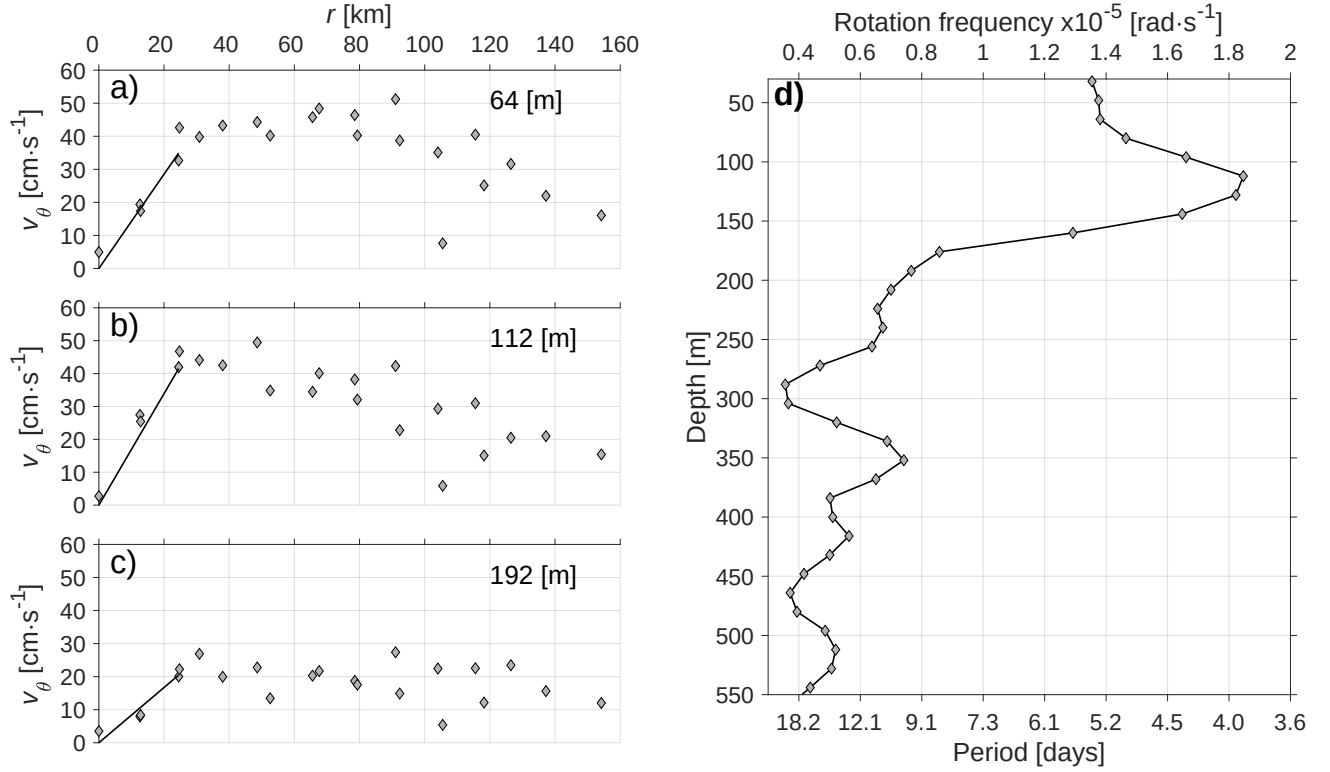
Figure 11. Radial profiles of azimuthal velocity ( v_\theta ) for the OceT transect at selected depths: a) 64 m, b) 112 m, and c) 192 m, derived from the OceT. Grey diamonds represent the observed data, while solid black lines correspond to the linear regression fit using v_\theta = \omega_\theta r , with v_\theta = 0 at r = 0 . The slope of the regression ( \omega_\theta ) is proportional to the angular velocity of the eddy. d) Depth-wise variation of the solid-body core's rotation frequency ( \omega_\theta ) and its corresponding period.
