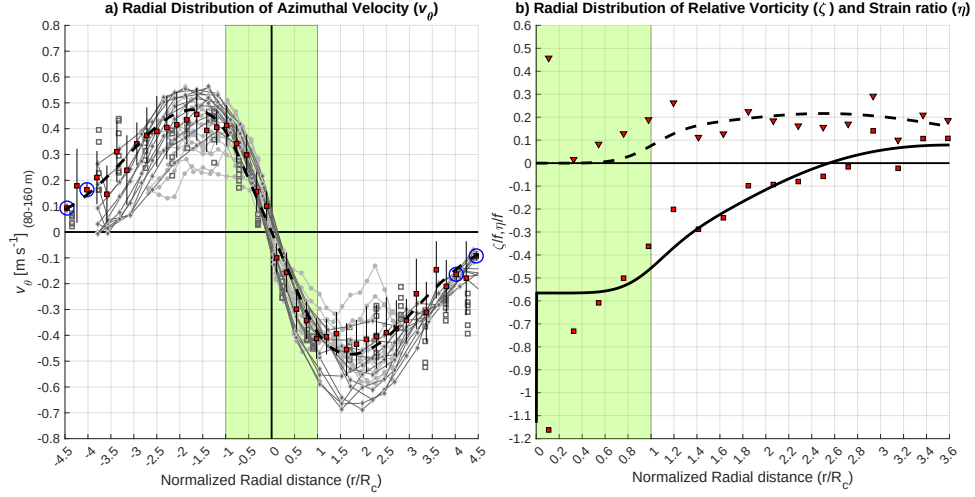
Figure 12. a) Radial distribution of azimuthal velocity ( v_\theta ) between 80 and 160 m depth, relative to the center of the Bentayga eddy normalized by R_c . Gray markers represent individual measurements from different survey phases: SeaSoar (T3 and T4; dark gray diamonds), Orthotransects (ZT and MT; light gray circles), and OcéT (dark gray open squares) (see Supplementary Note 3 for further details). The binned mean profile is shown as red-filled black squares, calculated over 5-km radial intervals; vertical bars indicate \pm 1 standard deviation. Blue-circled markers highlight bins with fewer than 10 observations. An hybrid model-derived velocity profile is overlaid (black dashed). b) Normalized relative vorticity ( \zeta/f , squares and solid lines) and strain rate ( \eta/f , triangles and dashed lines) as a function of normalized radial distance. Symbols denote observed values, and curves follow the same color scheme as in panel a). The green-shaded region in both panels marks the extent of the well-mixed eddy core ( |r| \leq R_c = 23 km).
