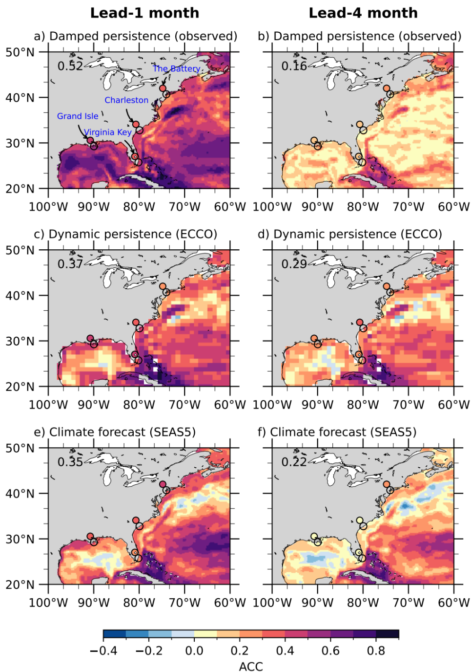
150 Figure 1. Retrospective forecast skill (ACC) at lead-1 and 4 months for the damped-persistence (observed; a and b), dynamic-persistence (ECCO; c and d), and climate-forecast (SEAS5; e and f) models. Forecasts of monthly sea level anomalies are compared to observations by altimetry (shading) and water level gauges (colored circles on land) at four example locations (indicated by unfilled circles on the coastline). The domain-averaged ACC is shown in the upper left of each panel.
