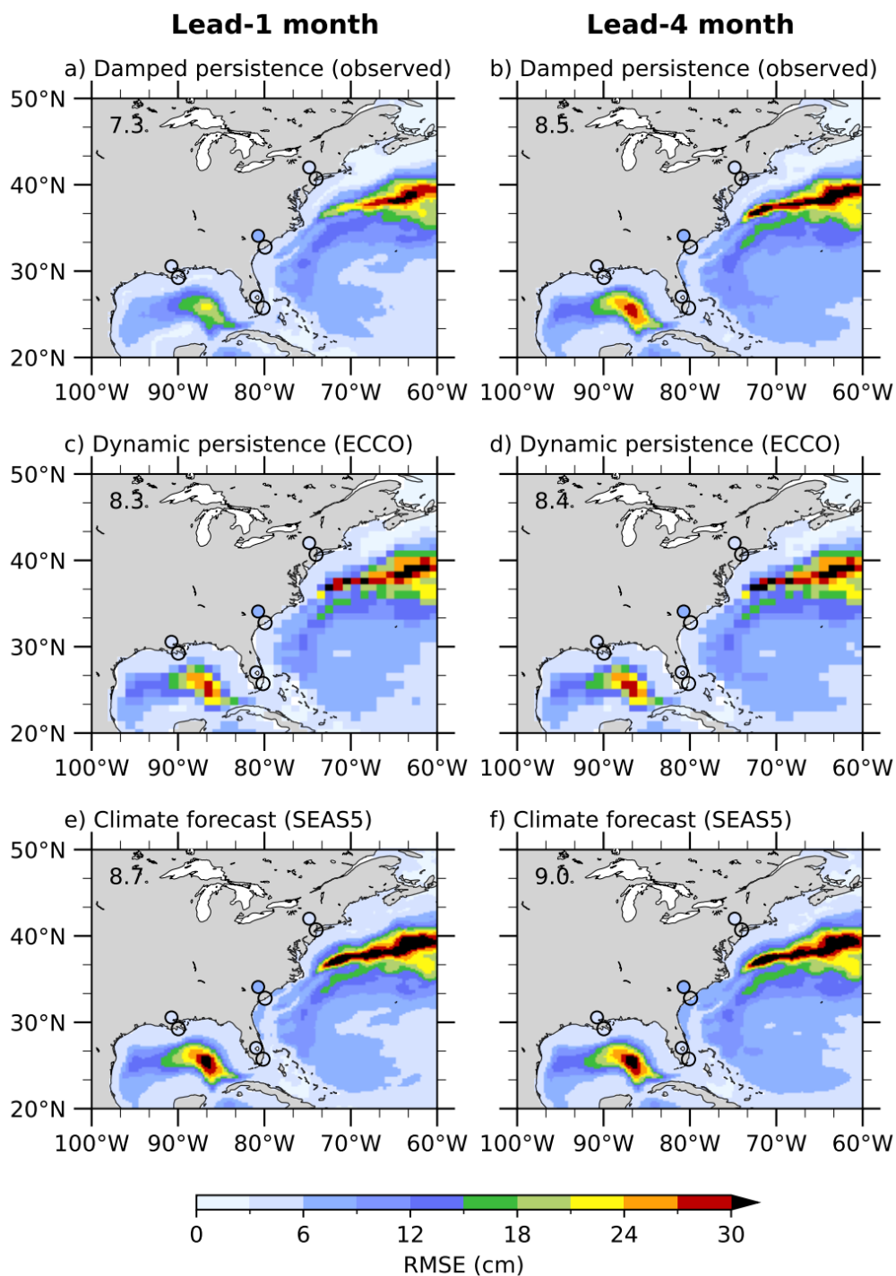
Figure 2. Same as Figure 1, but for RMSE.
