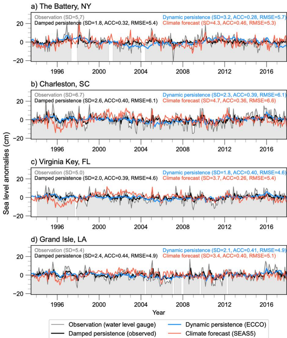
285 Figure 7. Time series of monthly sea level anomalies according to observations from water level gauges and the lead-1 month retrospective forecasts from the damped-persistence (observed), dynamic-persistence (ECCO), and climate-forecast (SEAS5) models. For each example location (labeled in Figure 1a), the SD (cm), ACC, and RMSE (cm) metrics are indicated for the models and observations (SD only).
