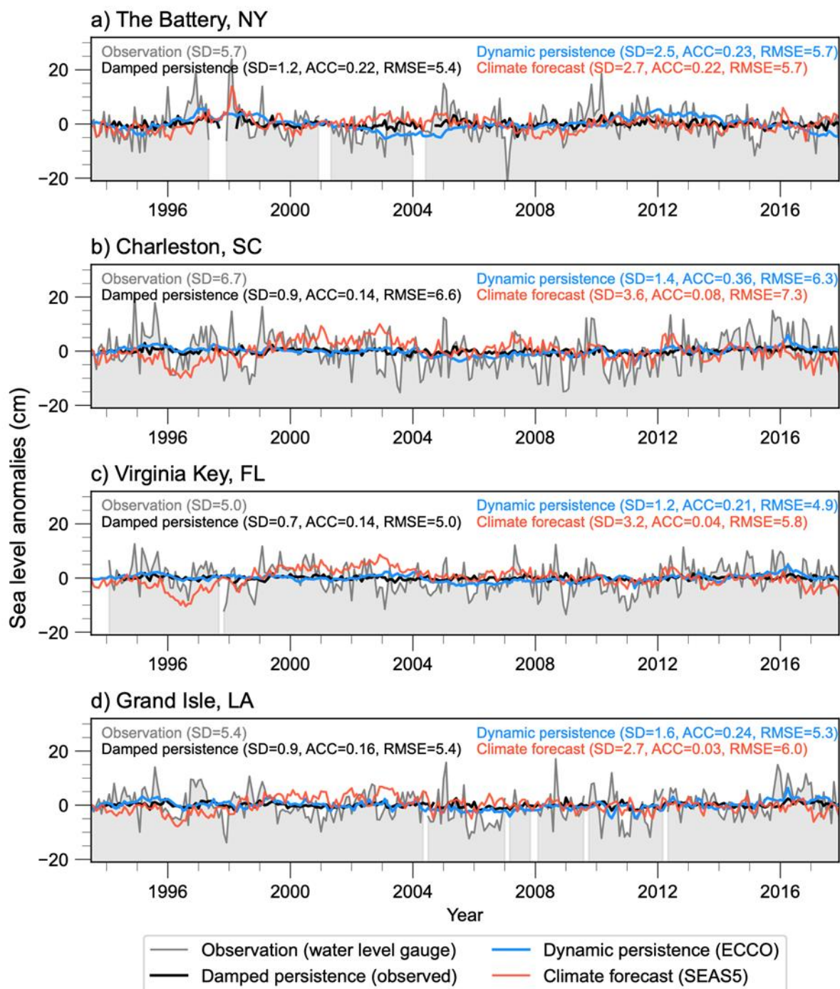
290 Figure 8. Same as Figure 7, but for the lead-4 month.
