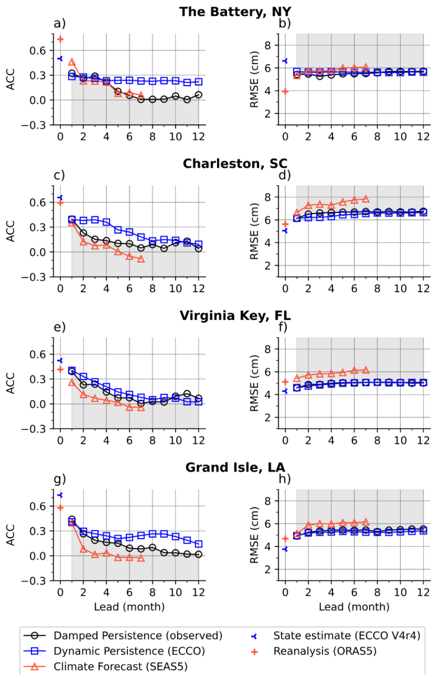
Figure 5. Retrospective forecast skill (ACC and RMSE) as a function of lead time at four example locations (labeled in Figure 1a). Markers (see legend) correspond to the damped-persistence (observed), dynamic-persistence (ECCO), and climate-forecast (SEAS5) models. Also shown are the state estimate (ECCO V4r4) and reanalysis (ORAS5), which are the initial conditions corresponding to the latter two forecasts. Monthly sea level anomalies from each product are compared to observations by water level gauges. Gray shading designates less skill than the damped-persistence model at a particular lead month (lower ACC and higher RMSE).
