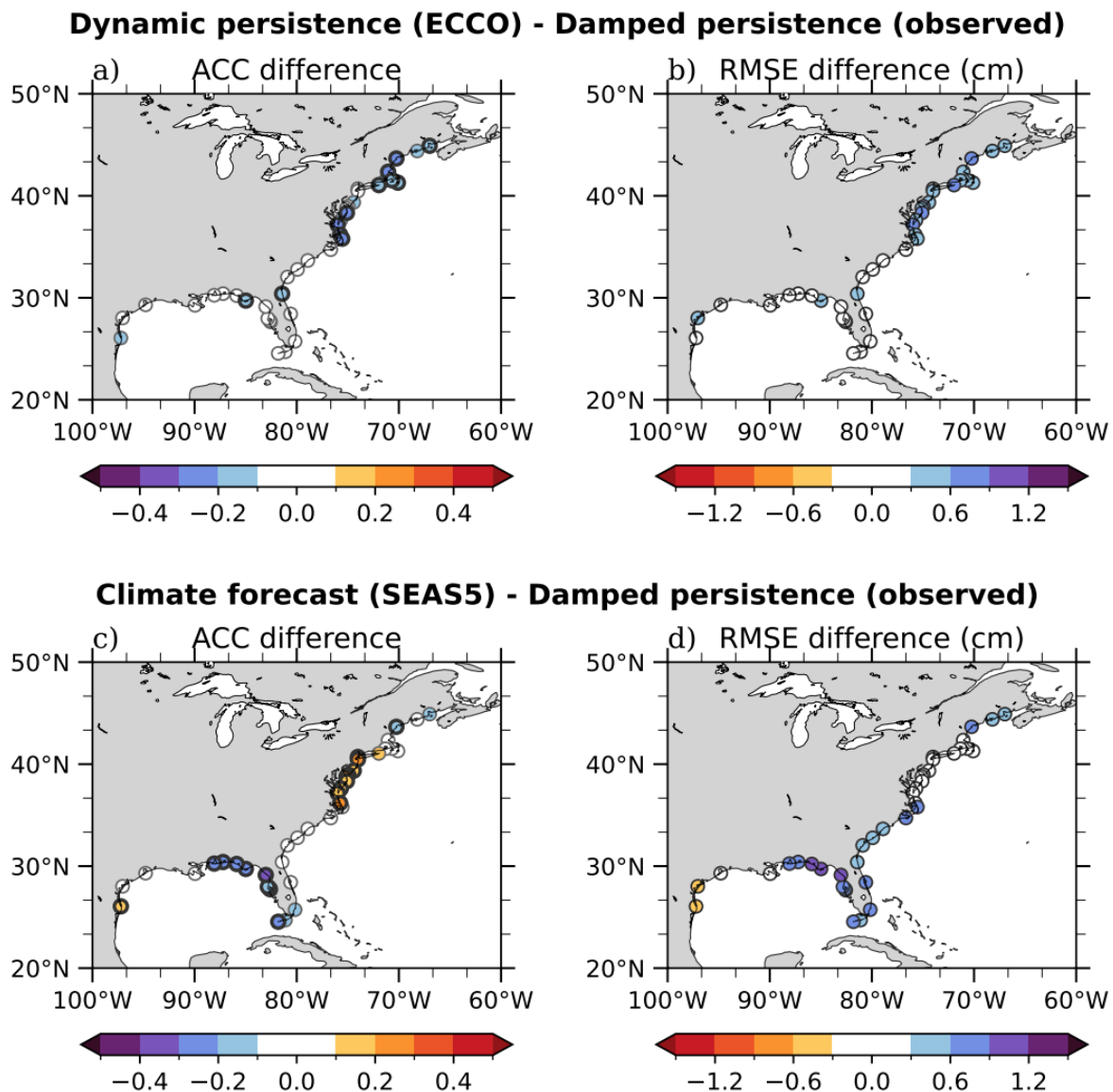
Figure 3. Differences of retrospective forecast skill (ACC and RMSE) at the lead-1 month for the dynamic-persistence (ECCO; a and b) and climate-forecast (SEAS5; c and d) models compared to damped persistence of monthly sea level anomaly observations by water level gauges (colored circles). Skill of the damped-persistence model is subtracted from that of the other models at each location. Orange shading indicates more skill (higher ACC and lower RMSE) compared to the damped-persistence model. Circles with thick black outlines denote statistically significant ACC differences at the 0.05 significance level.
