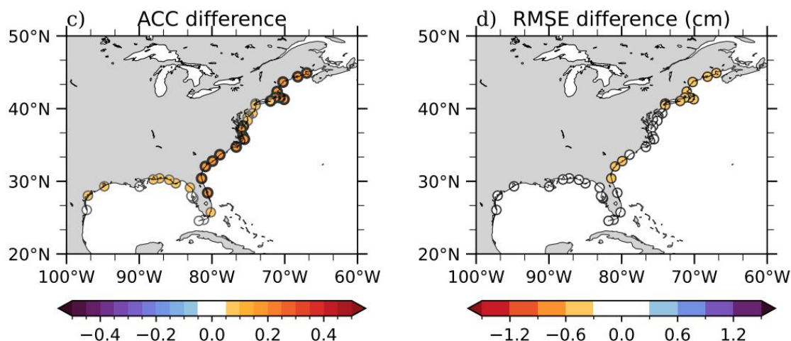
265 Figure 6. Difference of skill (ACC and RMSE) for the dynamic persistence (ECCO) and damped persistence (ECCO), with each product being compared to monthly sea level anomalies derived from the ECCO state estimate. Orange shadings indicate more skill (higher ACC and lower RMSE) for dynamic persistence (ECCO) compared to damped persistence (ECCO). Circles with thick black outlines denote statistically significant ACC differences at the 0.05 significance level. Note that smaller ACC differences are more likely to pass the significance test in (a) because the respective ACC values of both models are typically closer to one at the shorter lead time (e.g., at Virginia Key).
