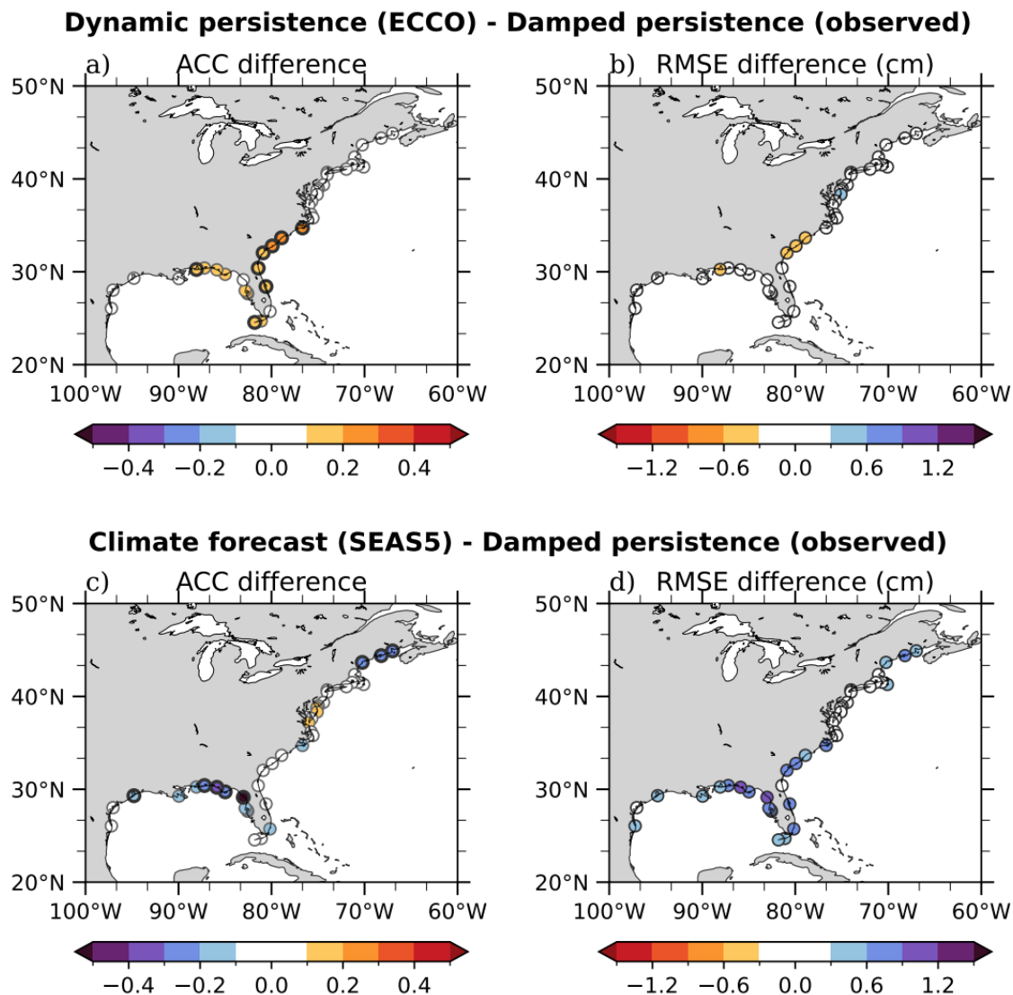
Figure 4. Same as Figure 3, but for the lead-4 month.
