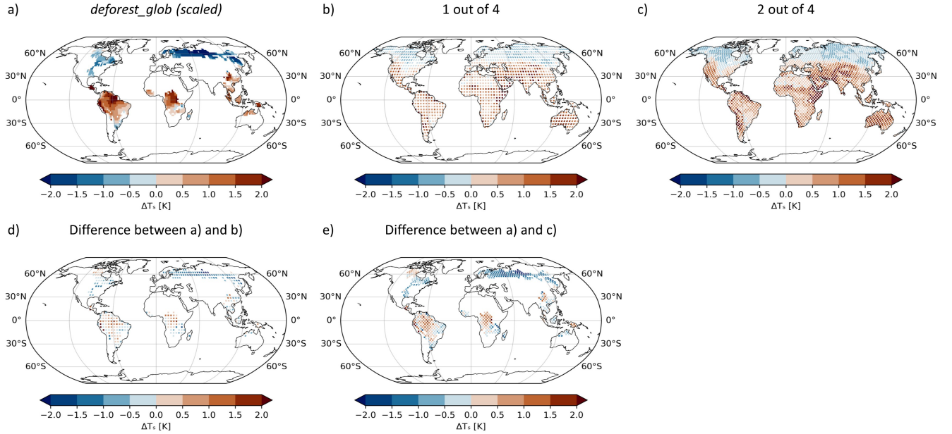
Figure A6. Comparison between the local effects in the deforest-glob simulation with scaling to 100% applied from this study (a) and the chessboard pattern simulations of Winckler et al. (2019a), where one out of four grid cells (b) or two out of four grid cells (c) are deforested. Here, all simulations are performed with MPI-ESM.
