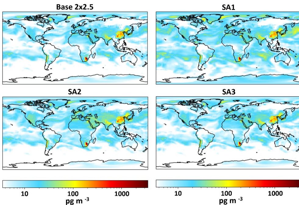
Figure 8. Average \text{Hg}^{\text{II}} concentrations at the surface on 9 June 2021 for four of the model simulations.
