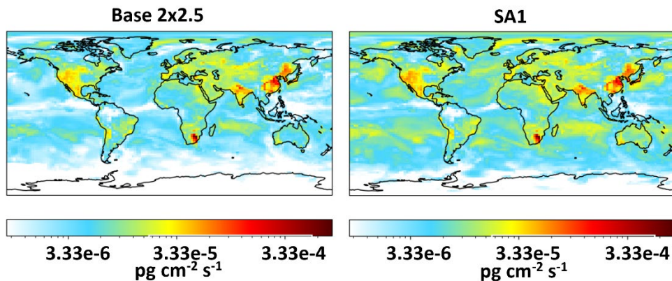
300 Figure 9. Average dry deposition for the Base 2x25 and SA1 simulations on 9 June 2021.
