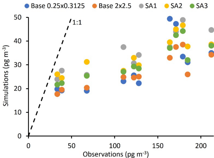
Figure 5. Observed versus simulated daily average Hg II . A 1:1 slope is shown as a black dashed line.
