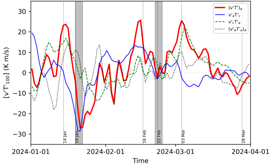
Figure 5. Time series of the anomalous 100 hPa meridional eddy heat flux (Eq. 3), v'T' - v'_c T'_c , area-averaged poleward of 45^\circ\text{N} (thick red) and its components v'_a T'_c (solid blue), v'_c T'_a (dashed green), and v'_a T'_a - (v'_a T'_a)_a (dotted black). The sub-indices c and a denote the climatological mean and anomalies. Vertical gray stripes indicate the window of 5-8 days after the onset same as in Fig. 4.
