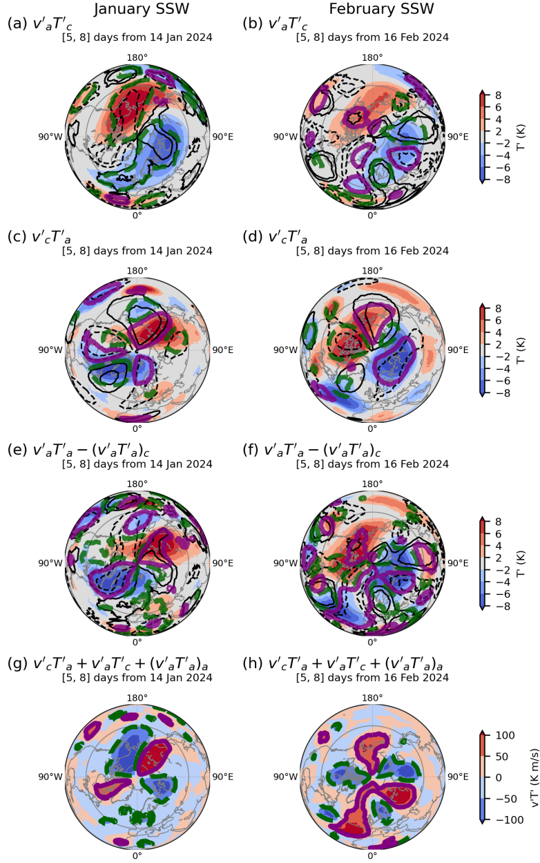
Figure 4. Details on the interference and nonlinear terms components of the anomalous meridional eddy heat flux in Eq. 1-3 around the SSW termination in January and February 2024. The thick solid purple (dashed green) contours of \pm 20 K m/s indicate positive (negative) values of 100 hPa meridional eddy heat flux components: (a-b) v'_a T'_c , (c-d) v'_c T'_a , (e-f) v'_a T'_a - (v'_a T'_a)_c . The eddy temperature, T' (K), either climatological in (a,b) or anomalous in (c-f), is shaded and the eddy meridional wind, v' (m/s), either climatological in (c-d) or anomalous in (a-b, e-f) is shown as black contours ( \pm 5, 10 m/s). (g-h) The anomalous 100 hPa meridional eddy heat flux ( sum of the interference and nonlinear terms in Eq. 1 ) is shaded, and positive (negative) contours of \pm 50 K m/s from Fig. 3 are highlighted as solid purple (dashed green) lines. Here, prime denotes the deviation from the zonal mean (or eddy component), while the sub-indexes c and a denote the climatological mean and anomalies.
