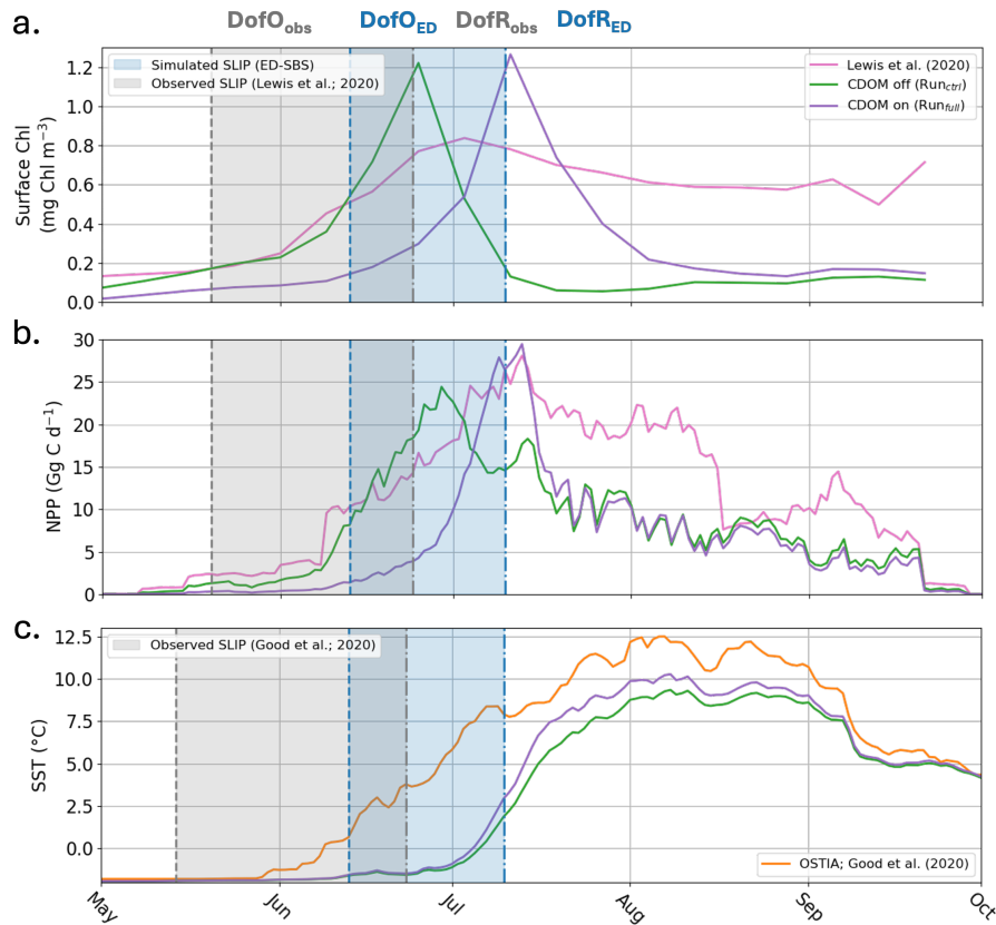
Figure 9. 2012 (a) averaged Surface Chl-a ( \text{mg Chl-a } m^{-3} ), (b) integrated NPP ( \text{Gg C } d^{-1} ), and (c) averaged SST ( ^{\circ}\text{C} ) over the Mackenzie River plume region for Run ctrl (green line), Run full (purple line), satellite observations (pink line Lewis et al., 2020), and in-situ/satellite observations (orange line Good et al., 2020). The blue (grey) area indicates the simulated (observed) seasonal loss of ice period.
