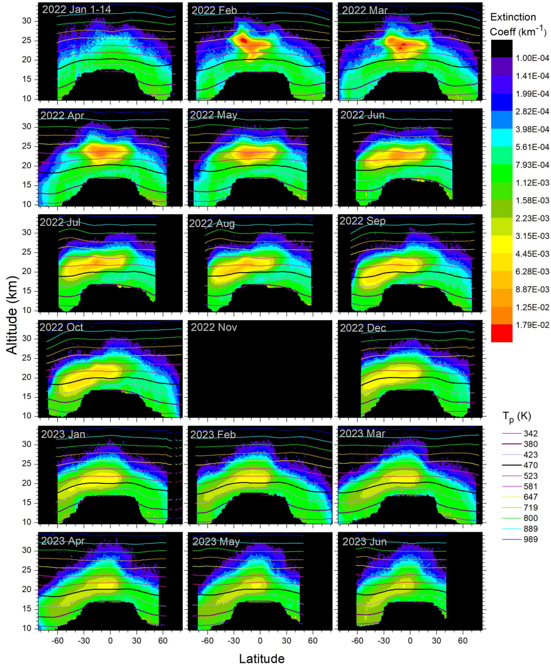
Figure 3. Monthly average extinction coefficients dependent on latitude and altitude with overlaid potential temperature levels. Note that “2022 Jan 1 – 14” covers only the pre-eruption period 1 – 14 January.
