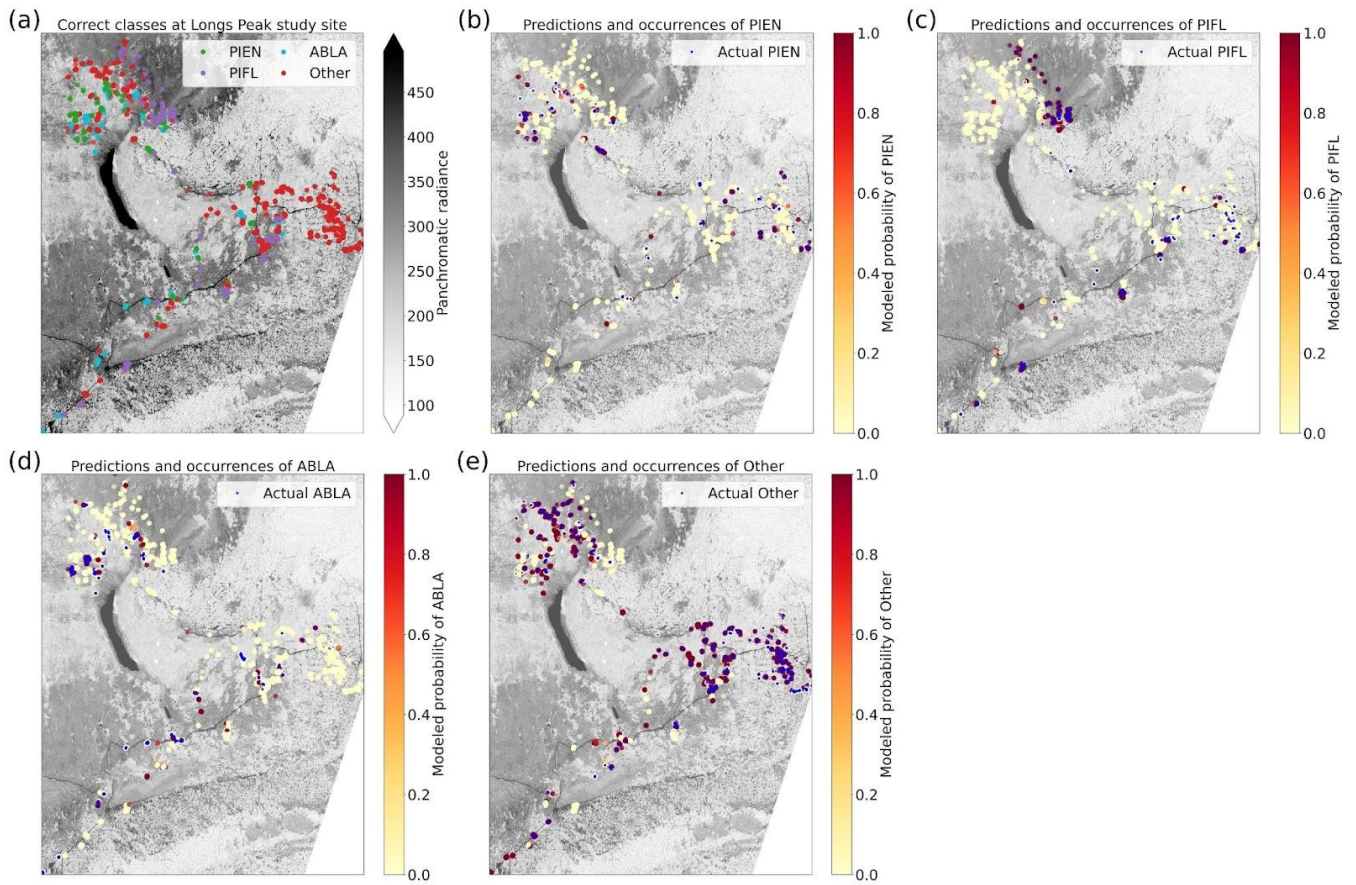
Figure D3. Targets and out-of-bag predictions for the 4-class model at the Longs Peak study site. Formatting is explained in the caption of Figure D1.
