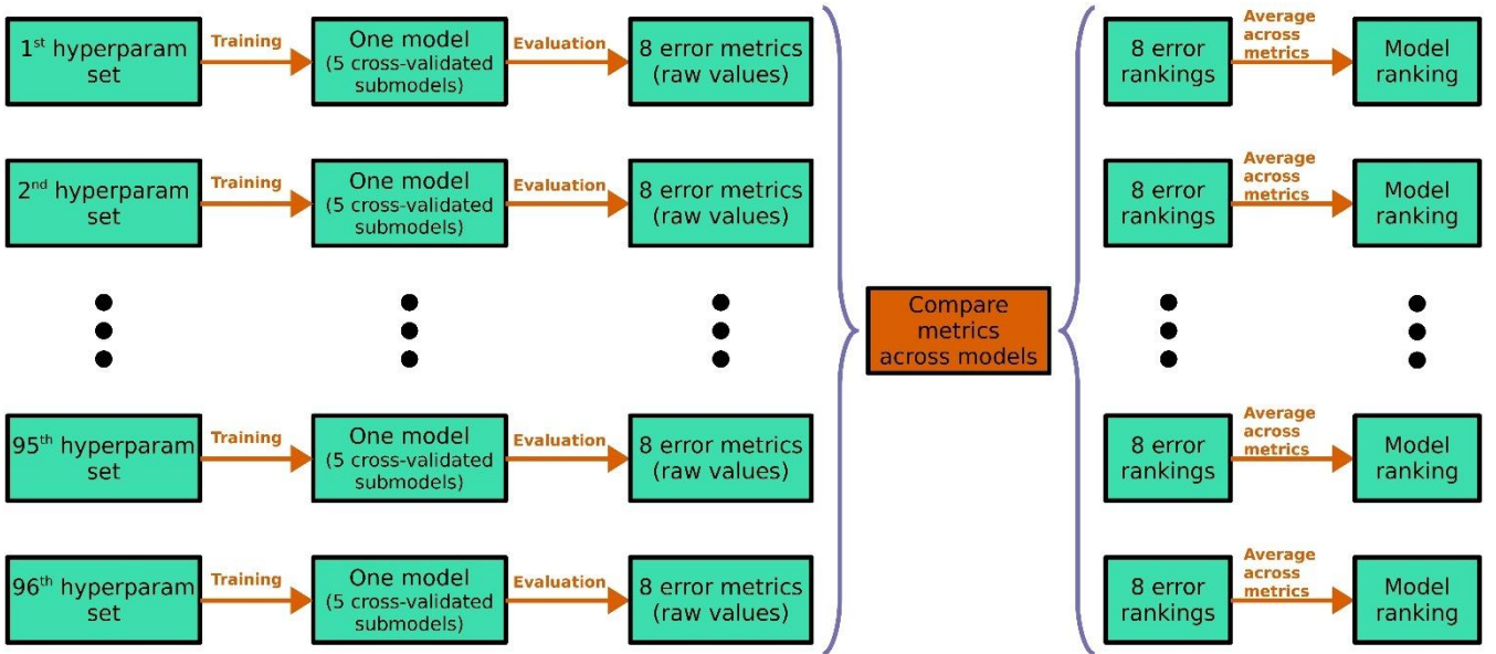
420 Figure 4. Schematic for the six-class hyperparameter experiment. The two- and four-class experiments follow the same methodology, except with 24 hyperparameter sets (hence, 24 models) instead of 96. Each row corresponds to one model; the black ellipsis (dots) represent the 3rd through 95th models; each green box represents an object (hyperparameter set, model, set of error metrics or rankings); and each orange arrow/box represents a procedure. The purple braces indicate that models are being compared with each other— i.e. , they indicate a procedure that cannot be done independently for each model. The last 425 procedure—implied but not shown—is choosing the model with the best "Model ranking," averaged over all eight error metrics.
