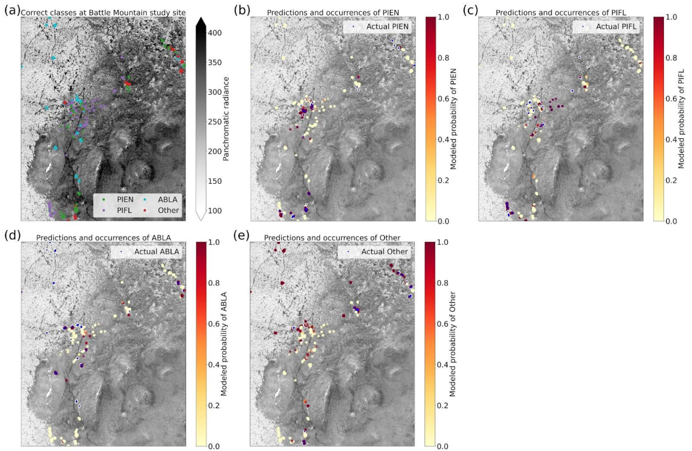
855 Figure D4: Targets and out-of-bag predictions for the 4-class model at the Battle Mountain study site. Formatting is explained in the caption of Figure D1.
