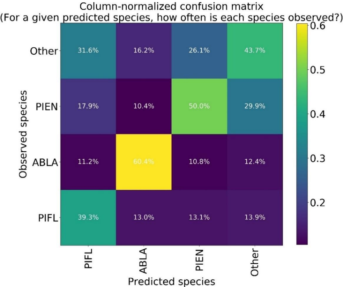
570 Figure 10: Column-normalized confusion matrix for the four-class model. Classes include subalpine fir (ABLA), Engelmann spruce (PIEN), limber pine (PIFL), and other classes pooled as “Other”.
