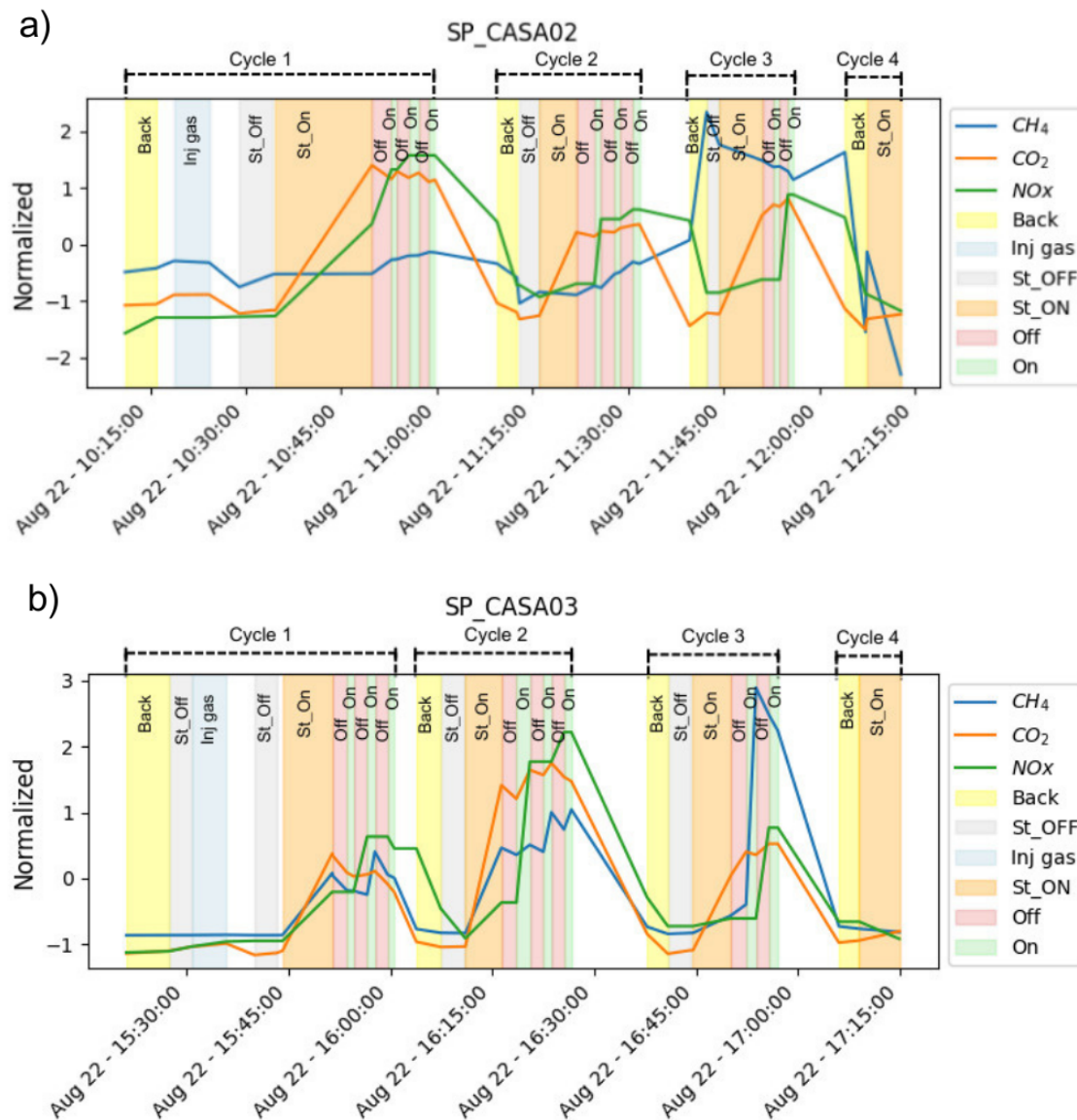
Figure 5. Temporal variability of the normalized concentrations of CH 4 , CO 2 and NO x . (a) House-Residence using Liquefied Petroleum Gas (SP_CASA02). (b) House-Residence using Natural Gas (SP_CASA03).
