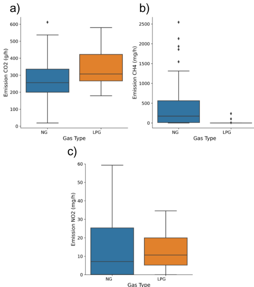
Figure 8. Emission rate-rates measured in the monitored households using natural gas (NG) and liquefied petroleum gas (LPG): (a) For carbon dioxide in grams per hour (g/h). (b) For methane in milligrams per hour (mg/h). (c) For nitrogen dioxide in milligrams per hour (mg/h).
