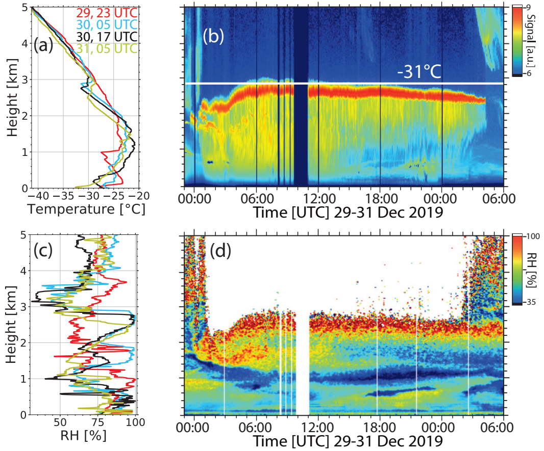
Figure 3. Temporal evolution of a long-lasting MPC event observed with Raman lidar aboard Polarstern at 86.6°N, 116–118°E, on 29–31 December 2019 (panel b). The height-time display of the 1064 nm range-corrected signal in panel b shows the droplet-dominated cloud layer (in red) between 2 and 3 km height and virgae (in yellow) of falling ice crystals. Profiles of temperature (panel a) and relative humidity (over water, panel c) were measured with MOSAiC radiosondes launched at 23 UTC (29 December), 5 and 17 UTC (30 December) and 5 UTC (31 December 2019). Thin black vertical lines in panel b indicate times of radiosonde observations. Cloud top temperature was between -28 and -32^{\circ}\text{C} . In panel d, the relative-humidity field derived from the water vapor Raman lidar measurements is shown. Several dark bars in panel b and white bars in panel d indicate times with non-useful lidar observations (partly caused by automated calibration and adjustment events). In panel d, the large white area above the MPCs indicates missing lidar data. In panels b and d, the lidar observations are biased in the near range ( <250 m).
