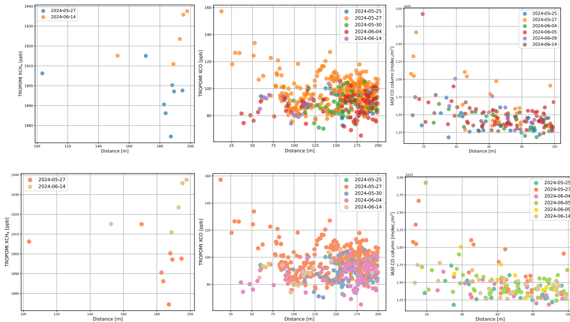
Figure A 3: Correlation between TROPOMI XCH 4 (a) and XCO (b) with the distance from each TROPOMI observation to the EM27/SUN location. Panel (c) shows the correlation between IASI CO and the distance from each IASI observation to the EM27/SUN location.
