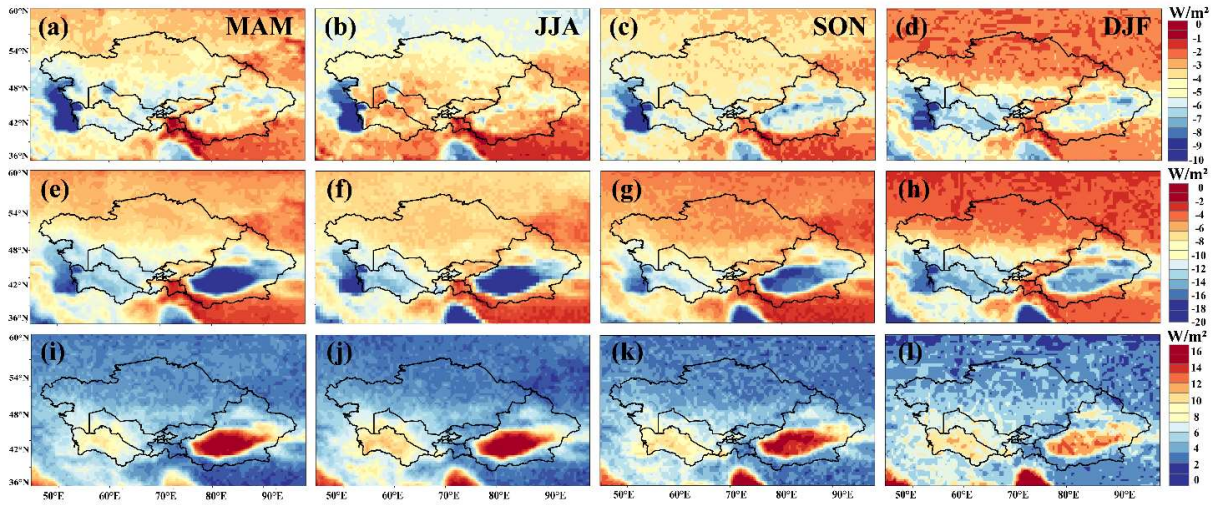
423 Figure. 7 Seasonal spatial distribution of clear-sky shortwave aerosol direct radiative forcing 424 (ADRF) due to dust aerosols in Central Asia (1980–2023): at the top of the atmosphere (panels a– 425 d), at the surface (e–h), and in the atmosphere (i–l).
