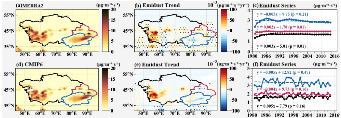
Figure 2 Spatial distribution, linear trends, and time series of dust emissions from MERRA-2 and the CMIP6 multi-model ensemble (MME) in Central Asia from 1980 to 2014. The red outline delineates Northern Xinjiang, the blue outline delineate Southern Xinjiang, and the black outlines denote the five Central Asian countries. Black dots in panels (b) and (e) mark regions significant at the 95% confidence level.
