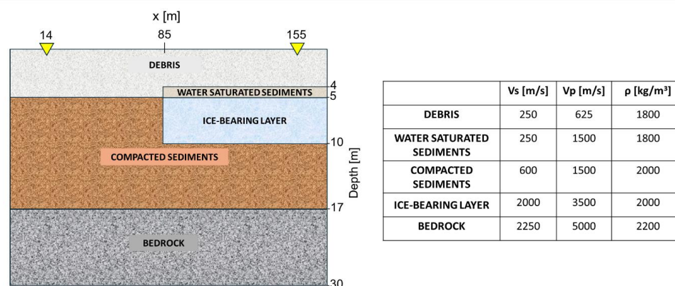
Figure 4: Conceptual model used for the synthetic seismic modelling with the SW4 software (Pettersson and Sjögreen, 2023). The two yellow triangles denote the first and the last geophones in the array. Abbreviations as in Tab. 1.
