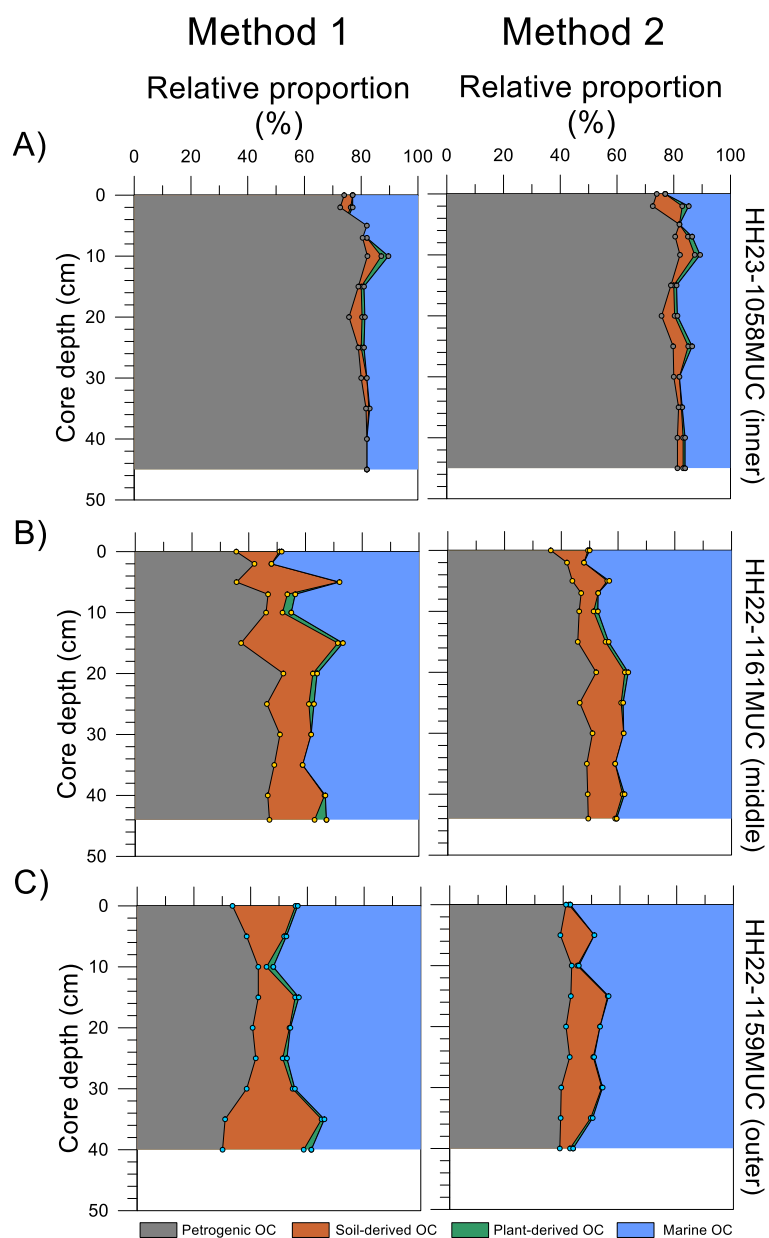
Fig. 9. Depth profiles showing the relative proportions of petrogenic, soil-derived, plant-derived, and marine OC, as determined using Method 1 (based on \delta^{13}\text{C}_{\text{org}} (‰ VPDB), \Delta^{14}\text{C}_{\text{org}} (‰), and (Ad/Al) v ratio) and Method 2 (based on \delta^{13}\text{C}_{\text{org}} (‰ VPDB), \Delta^{14}\text{C}_{\text{org}} (‰), and lignin phenols (mg/gOC)), for the cores (A) HH23-1058MUC, (B) HH22-1161MUC, and (C) HH22-1159MUC.
