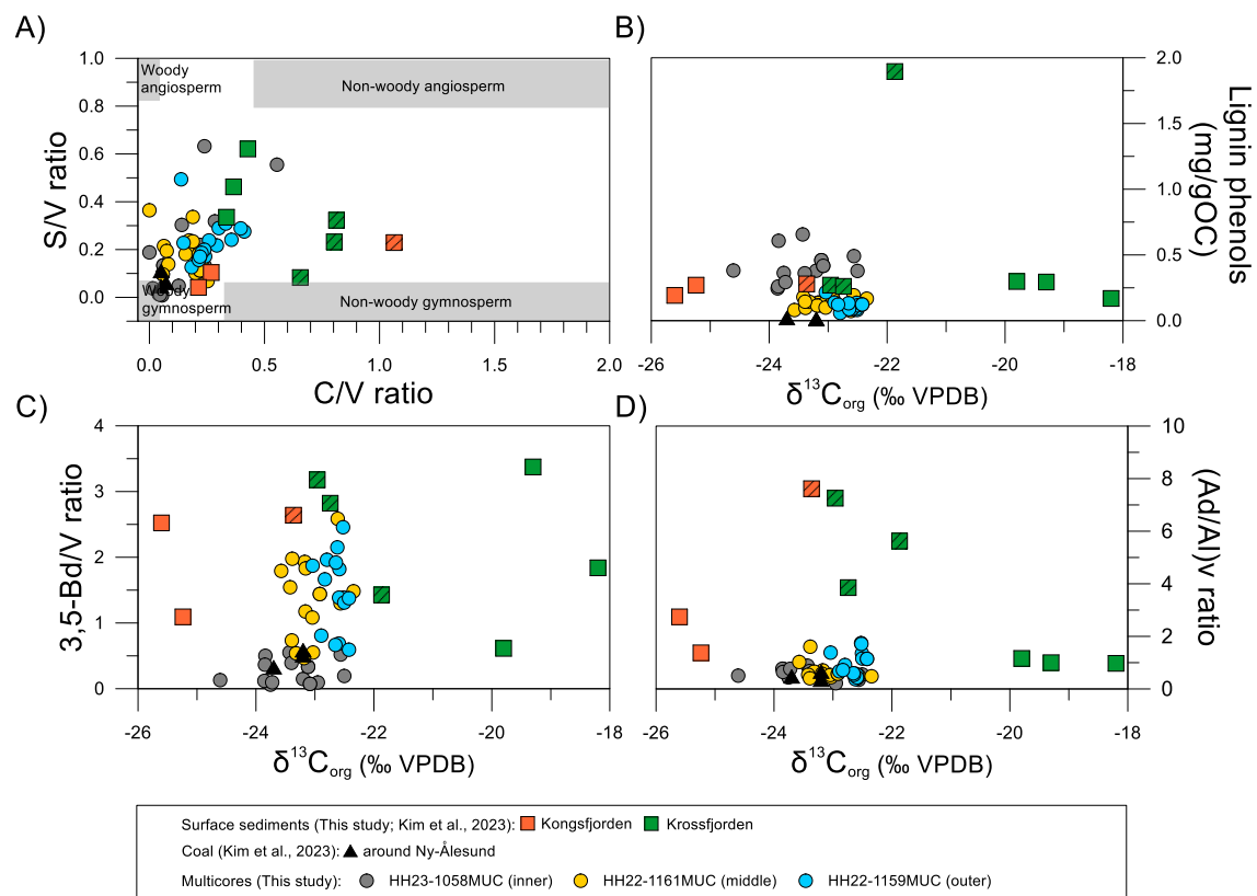
1010 Fig. 8. Scatter plots of (A) C/V ratio versus S/V ratio, including the end-members for 1011 different vascular plant tissues (cf. Goñi et al., 2000), (B) \delta^{13}C_{org} (‰ VPDB) versus lignin 1012 phenols (mg/gOC), (C) \delta^{13}C_{org} (‰ VPDB) versus 3,5-Bd/V ratio, and (D) \delta^{13}C_{org} (‰ 1013 VPDB) versus (Ad/Al)v ratio for the three cores, compared with data from coals (Kim et 1014 al., 2023) and surface sediments (Kim et al., 2023 and this study). Note that the surface 1015 sediment samples newly analyzed in this study are indicated by hashed square symbols.
