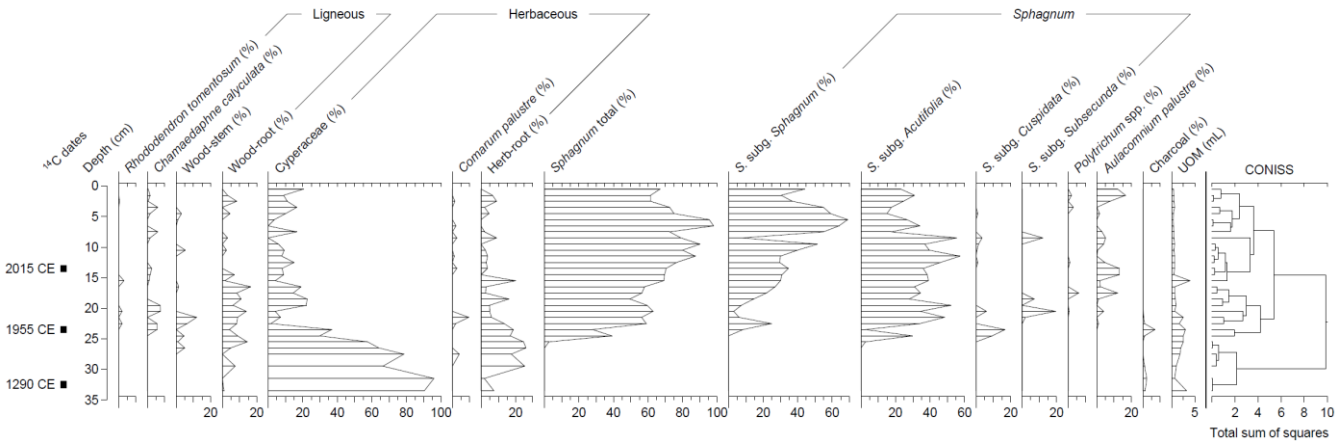
600 Figure A2. Macrofossil diagram of core TQ22-C2.
