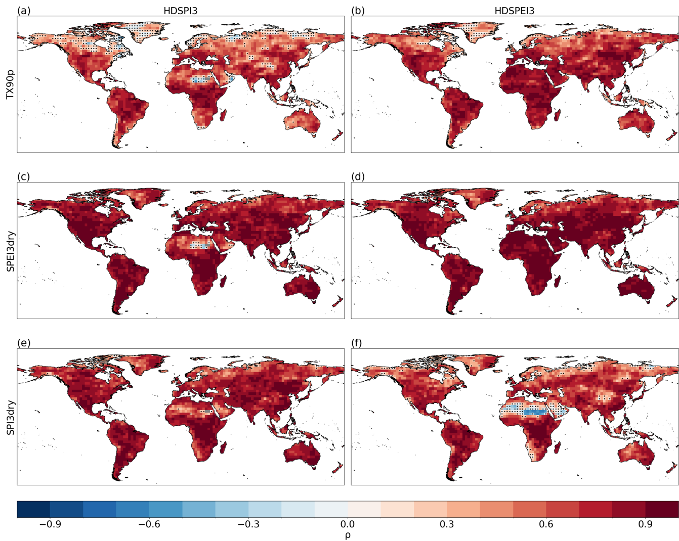
Figure A6. Spearman rank correlation between the annual sum of HD SPI3 (a,c,e) and HD SPEI3 (b,d,f) and TX90p, SPEI3dry and SPI3dry respectively, in the ERA5 dataset. Hatching indicates correlations not statistically significant at the 95% confidence level ( p -value < 0.05) using a two-tailed test.
