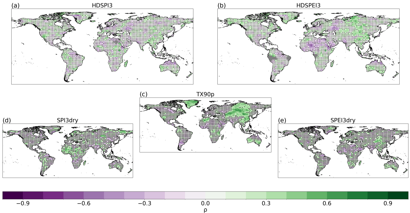
Figure 2. Spearman’s rank residual correlation for HDSPI3 (a), HDSPEI3 (b), TX90p (c), SPI3dry (d) and SPEI3dry (e) for the average forecast years 2-5. Dots indicate areas where the residual correlation is not statistically significant at the 95% confidence level. Grey areas indicate missing data.
