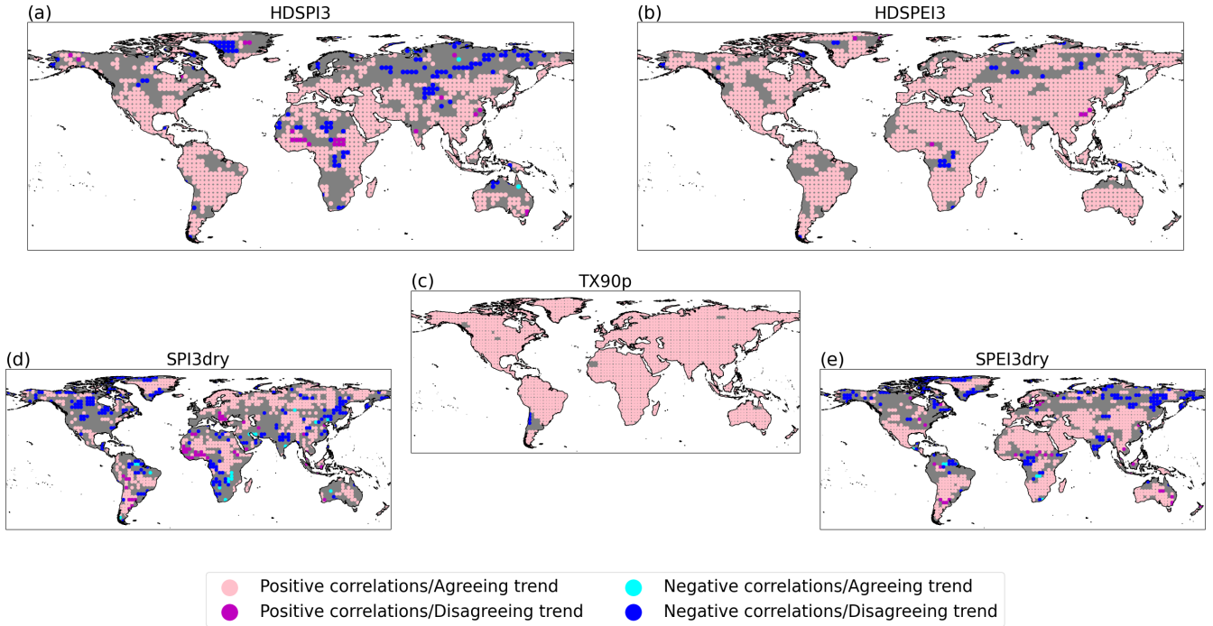
Figure 3. Statistically significant Spearman's rank correlation against the trend sign for HD SPI3 (a), HDSPEI3 (b), TX90p (c), SPI3dry (d) and SPEI3dry (e) for the average forecast years 2-5 (as in Figure 1). Pink (magenta) dots indicate areas where the correlation is positive and statistically significant, and where the trends of GPCC-BEST and DCP MME show the same (opposite) sign. Light blue (Dark blue) dots indicate areas where the correlation is negative and statistically significant, and where the trends of GPCC-BEST and DCP MME show the same (opposite) sign. Grey areas indicate grid points where the correlation is non-significant.
