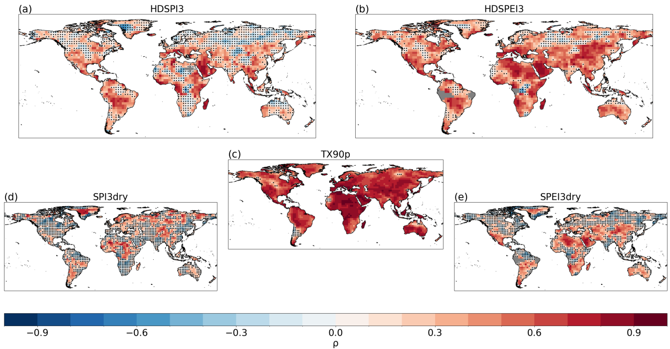
Figure 1. Spearman’s rank correlation for HDSPI3 (a), HDSPEI3 (b), TX90p (c), SPI3dry (d) and SPEI3dry (e) for the average forecast years 2-5 (1962-2014). Dots indicate regions where the correlation is not statistically significant at the 95% confidence level. Grey areas indicate missing data.
