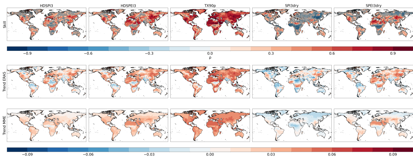
Figure A5. First row: Spearman rank correlation between the ERA5 dataset and the DCPP MME ensemble mean for HDSPI3, HDSPEI3, TX90p, SPI3dry and SPEI3dry respectively. Hatchings indicate correlations not statistically significant at the 95% confidence level ( p -value < 0.05) using a one-tailed test. Second row: Normalized trends in the ERA5 dataset for HDSPI3, HDSPEI3, TX90p, SPI3dry and SPEI3dry respectively. Third row: Median normalized trends, calculated ensemble-wise, in the DCPP MME ensemble for HDSPI3, HDSPEI3, TX90p, SPI3dry and SPEI3dry respectively.
