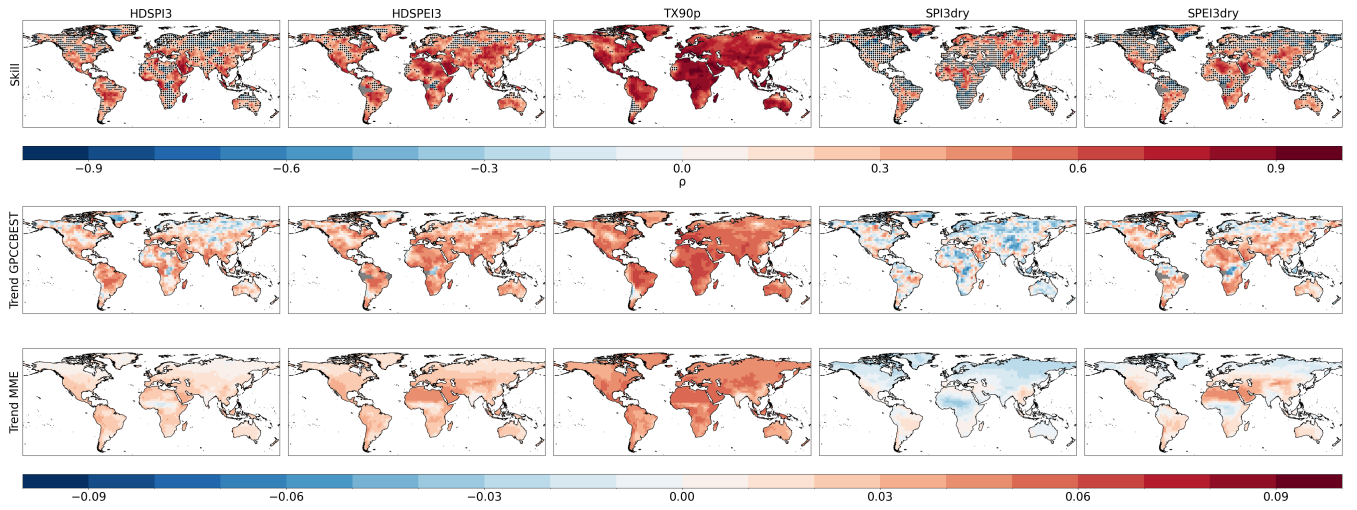
Figure A4. First row: Spearman rank correlation between the GPCC-BEST dataset and the DCPP MME ensemble mean for HDSPi3, HDSPEi3, TX90p, SPI3dry and SPEi3dry respectively. Hatchings indicate correlations not statistically significant at the 95% confidence level ( p -value < 0.05 ) using a one-tailed test. Second row: Normalized trends in the GPCC-BEST dataset for HDSPi3, HDSPEi3, TX90p, SPI3dry and SPEi3dry respectively. Third row: Median normalized trends, calculated ensemble-wise, in the DCPP MME ensemble for HDSPi3, HDSPEi3, TX90p, SPI3dry and SPEi3dry respectively. Grey areas indicate missing data.
