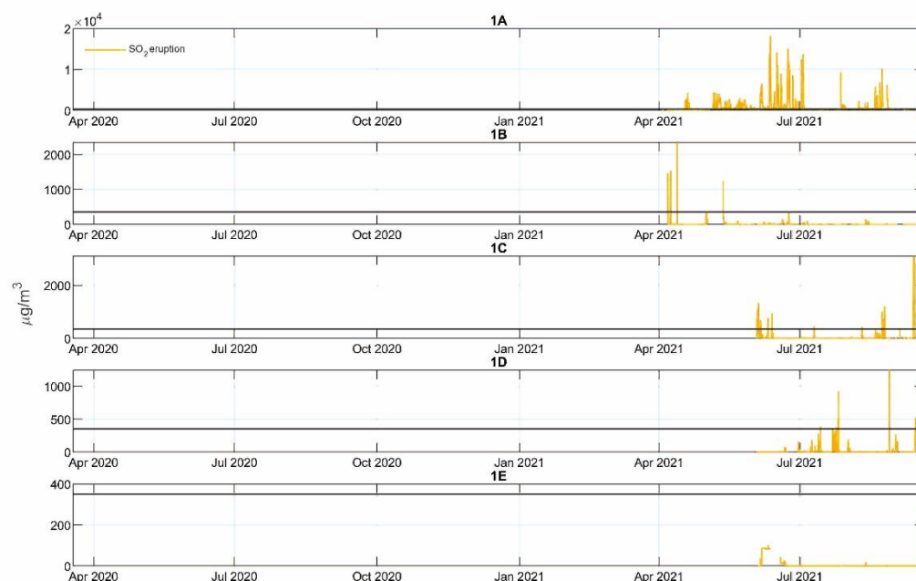
Figure B1 Time series of hourly-mean concentrations \text{SO}_2 ( \mu\text{g}/\text{m}^3 ), measured by the eruption site stations (G1 A-E) during the 2021 eruption. The stations were not in operation before the eruption and therefore there are no data on pre-eruptive background. The ID air quality threshold of 350 \mu\text{g}/\text{m}^3 hourly-mean is shown on all panels with a black horizontal line. Note that the eruption-site sensors have low accuracy and were only used in this study to indicate time periods that were over the ID threshold, the absolute concentration values were not included in the analysis.
