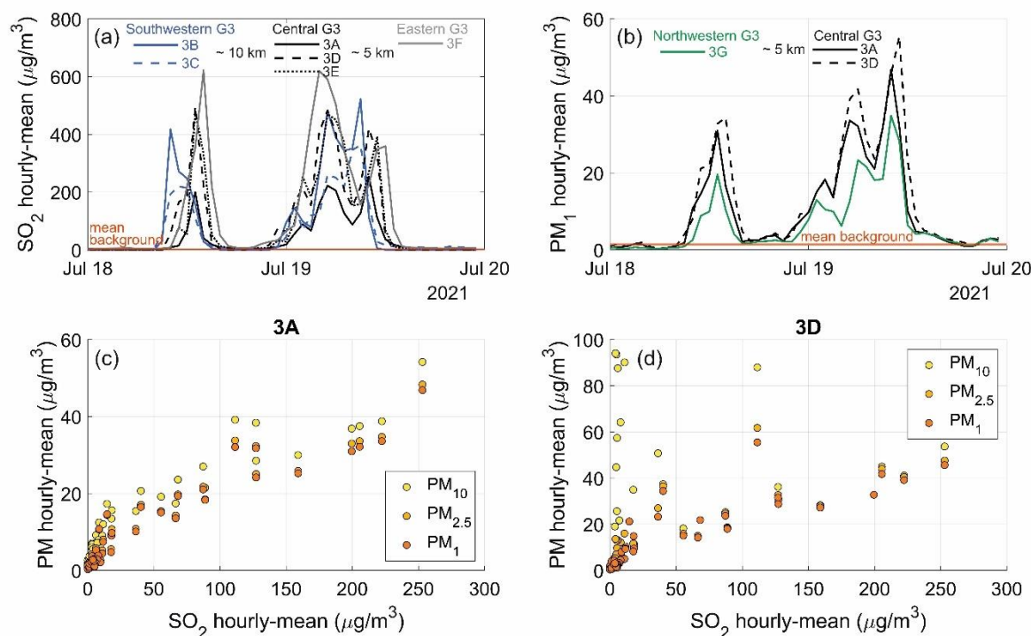
Figure 7: SO 2 and PM concentrations ( \mu\text{g}/\text{m}^3 ) during a 'fresh' volcanic plume advection episode in Reykjavik capital area (G3) 18-19 July 2021. 3A to 3F are names of reference-grade stations and the figure indicates their respective locations within Reykjavik (southwestern, central, eastern, and northwestern) and the approximate distance between them. Panel (a): SO 2 hourly-means timeseries. Panel (b): PM 1 hourly-means timeseries. Panel (c): Scatter plot between concentrations of SO 2 and PM 10 , PM 2.5 and PM 1 at station 3A, which measured all of these pollutants. Panel (d): Scatter plot between concentrations of SO 2 and PM 10 , PM 2.5 and PM 1 at station 3D, which measured all of these pollutants.
