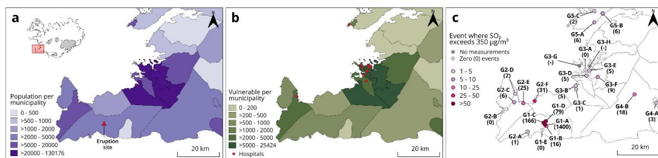
Figure 9: Potential exposure of the general population of Iceland to above-threshold \text{SO}_2 concentrations ( 350 \mu\text{g}/\text{m}^3 hourly-mean). Panel (a): Population map at the municipality level of the densely populated southwestern part of Iceland, including the Reykjavík capital area (area G3). Population data in this figure for 2020 from Statistics Iceland. Panel (b): Map of potentially vulnerable sub-populations ( \leq 4 years and \geq 65 years of age) in each municipality. Location of hospitals is shown. Panel (c): Number of events when \text{SO}_2 concentrations exceeded the ID air quality threshold of 350 \mu\text{g}/\text{m}^3 hourly-mean during the eruption period as measured by the monitoring stations (areas G1, G2 and G3). Source and copyright of basemap and cartographic elements: Icelandic Met Office & Icelandic Institute of Natural History.
