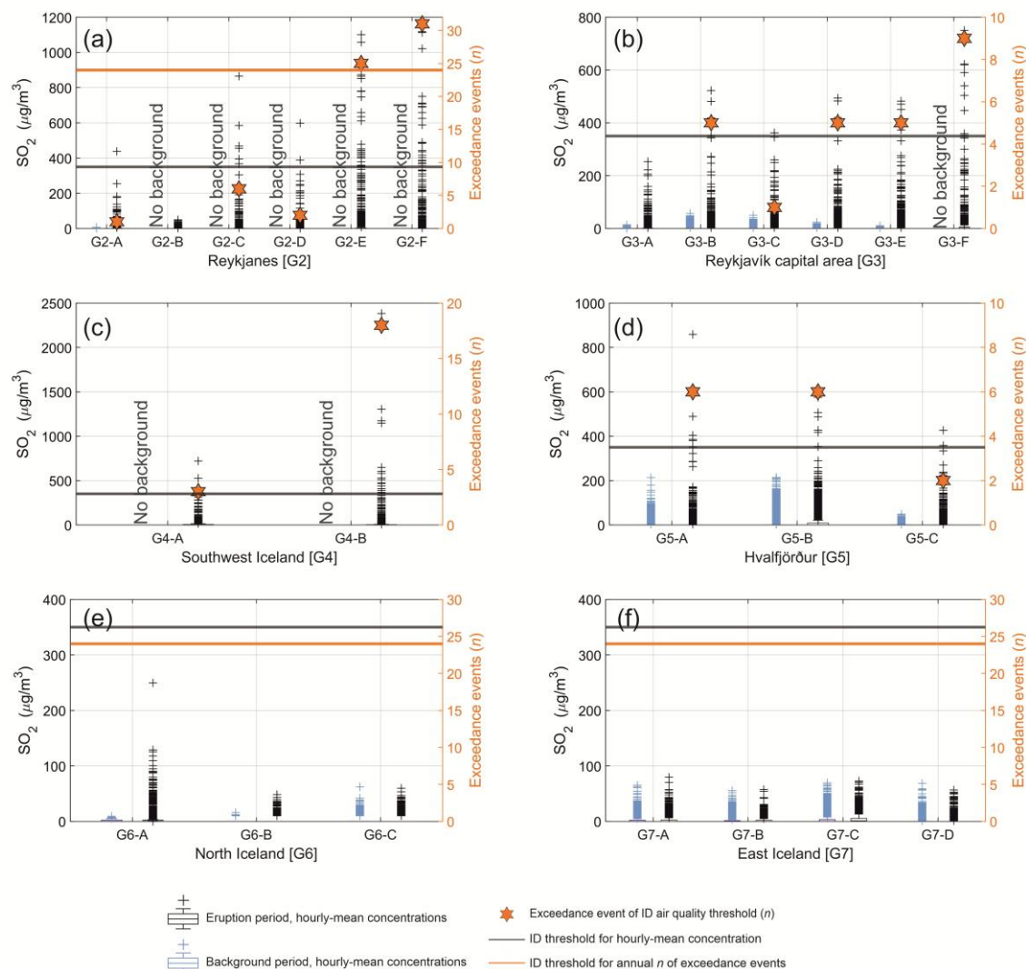
Figure 3: SO 2 hourly-mean concentrations (μg/m 3 ) and number of Icelandic Directive (ID) threshold exceedance events, measured by 24 regulatory-grade stations in populated areas in Iceland shown as six geographic clusters G2-G7 (panels a-f). Pre-eruptive background data are shown for stations that were operational before the eruption began. The data are presented as box-and-whisker plots: boxes represent the interquartile range (IQR), the whiskers extend to \pm 2.7\sigma from the mean, and crosses represent very high values (statistical outliers beyond \pm 2.7\sigma from the mean). Note that the IQR is very low in most cases due to the negligible SO 2 concentrations in the local background; as a result, most of the SO 2 pollution episodes are statistical outliers. The ID air quality threshold of 350 μg/m 3 hourly-mean is indicated by a black horizontal line in all panels. Orange stars represent the number of times this threshold was exceeded at each station ('Exceedance events'). The annual limit for cumulative hourly exceedance events is 24, shown by an orange horizontal line. Stations with orange stars above the orange line exceeded the annual threshold. Time series plots for each station are available in Appendix A.
