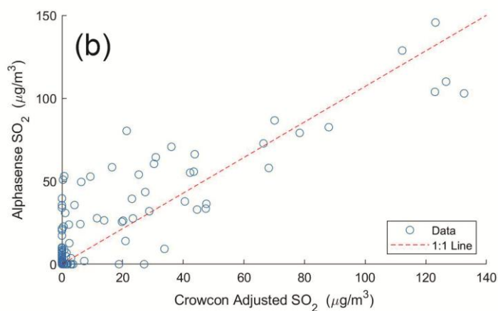
Figure A2: SO 2 concentrations measured by two types of lower-cost sensors (LCS) used in this study—Alphasense SO 2 -B4 and Crowcon XGuard—during a field colocation at the eruption site (6–22 June 2021). Measurements from the two sensors showed a strong linear correlation ( r^2 = 0.70 ), but Alphasense reported lower values relative to Crowcon, with a correlation coefficient of 0.38. Panel (a) Correlation of raw data points from the two sensors. Panel (b) Correlation after Crowcon data were adjusted using the correlation coefficient
