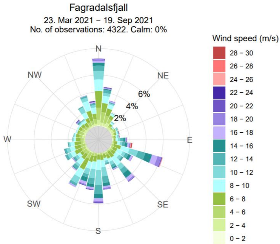
Figure A13: Wind rose shows wind direction (wind coming from) and wind speed measured by Icelandic Meteorological Office weather station at the Fagradalsfjall eruption site 23 March – 19 September 2021.
