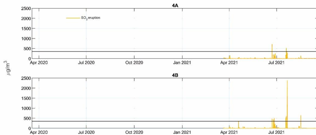
835 Figure A6: Time series of hourly-mean concentrations SO 2 (µg/m 3 ), measured in Southwest Iceland by regulatory air quality stations (G4 A-B) during the 2021 eruption. The stations were not in operation before the eruption and therefore there are no data on pre-eruptive background. The ID air quality threshold of 350 µg/m 3 hourly-mean is shown on all panels with a black horizontal line.
