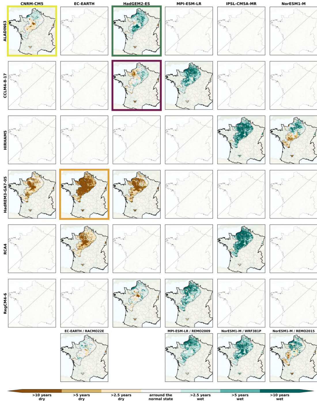
Figure 3. Spatial distribution of the SPLI median over the AquifR domain under the RCP8.5 on the long-term horizon (2071-2099) , following the different GCM (in column) / RCM (in line) combination. The last line corresponds to couples where RCMs are used only once. The coloured rectangles indicates the GCM/RCM couples corresponding to the storylines (see section 2.1). The missing panels indicate the GCM/RCM couples not included in the EXPLORE2 climate projection dataset.
