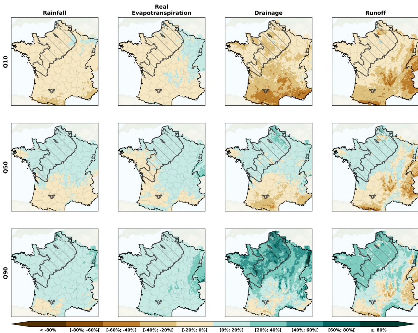
Figure D3. Spatial distribution of the total rainfall (1 st column) from the CPs for the RCP8.5, and of the real evapotranspiration (2 nd column), the drainage (3 rd column) and the runoff (4 th column) simulated by the land surface model SURFEX. The results are represented by the quantiles Q10, Q50 and Q90 from all the CPs over the long-term horizon (2071-2099).
