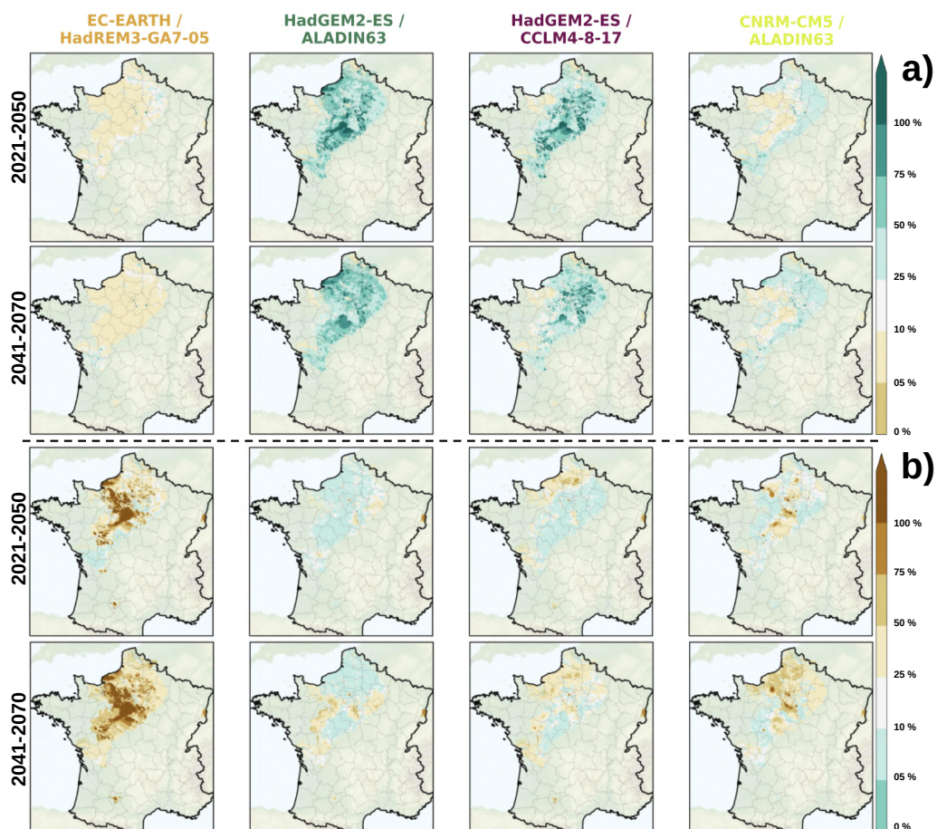
Figure C2. Spatial distribution of the median of the time proportion corresponding to extreme wet events ( SPLI > +1.28 , a)) and extreme dry events ( SPLI < -1.28 , b)) for the short-term and intermediate horizons (in line) for the four storylines (in column).
