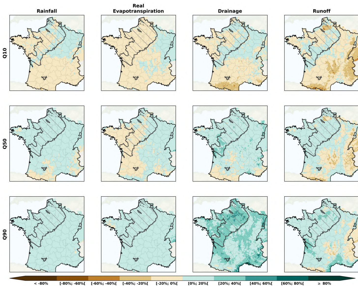
Figure D2. Spatial distribution of the total rainfall (1 st column) from the CPs for the RCP4.5, and of the real evapotranspiration (2 nd column), the drainage (3 rd column) and the runoff (4 th column) simulated by the land surface model SURFEX. The results are represented by the quantiles Q10, Q50 and Q90 from all the CPs over the long-term horizon (2071-2099).
