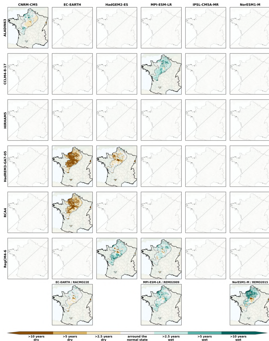
Figure B2. Spatial distribution of the SPLI median over the AquifR domain under the RCP2.6 on the intermediate-term horizon (2041-2070) , following the different GCM (in column) / RCM (in line) combination. The last line corresponds to couples where RCMs are used only once. The missing panels indicate the GCM/RCM couples not included in the EXPLORE2 climate projection dataset.
