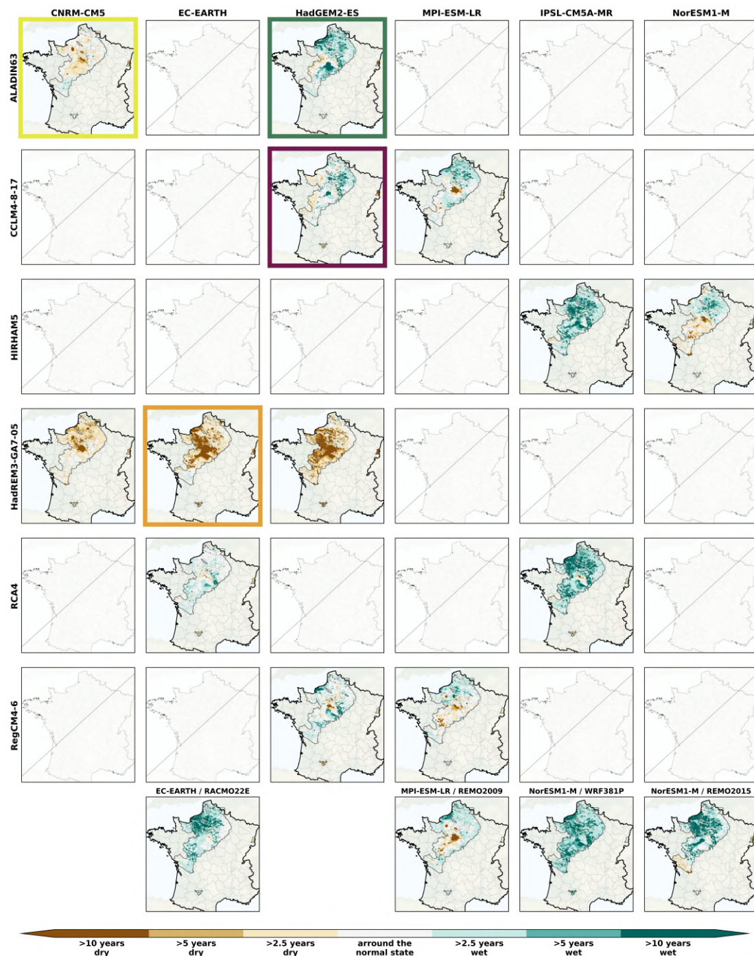
Figure B8. Spatial distribution of the SPLI median over the AquifR domain under the RCP8.5 on the intermediate-term horizon (2041-2070) , following the different GCM (in column) / RCM (in line) combination. The last line corresponds to couples where RCMs are used only once. The colored rectangles indicates the GCM/RCM couples corresponding to the storylines (see section 2.1). The missing panels indicate the GCM/RCM couples not included in the EXPLORE2 climate projection dataset.
