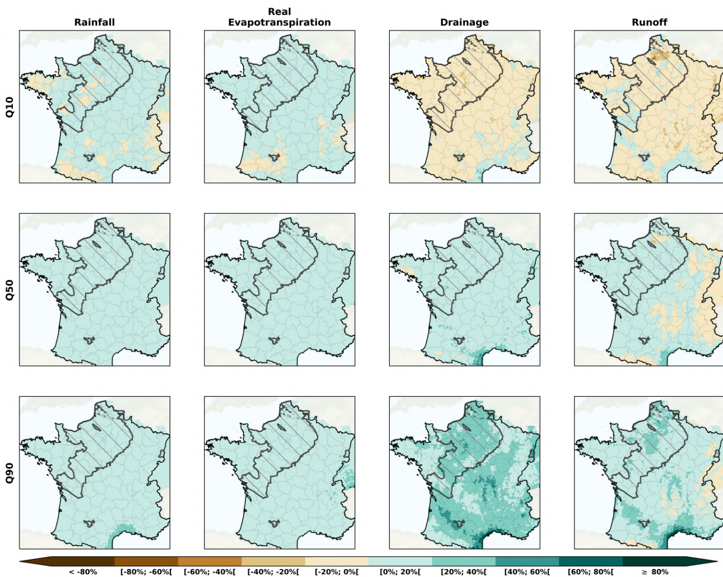
Figure D1. Spatial distribution of the total rainfall (1 st column) from the CPs for the RCP2.6, and of the real evapotranspiration (2 nd column), the drainage (3 rd column) and the runoff (4 th column) simulated by the land surface model SURFEX. The results are represented by the quantiles Q10, Q50 and Q90 from all the CPs over the long-term horizon (2071-2099).
