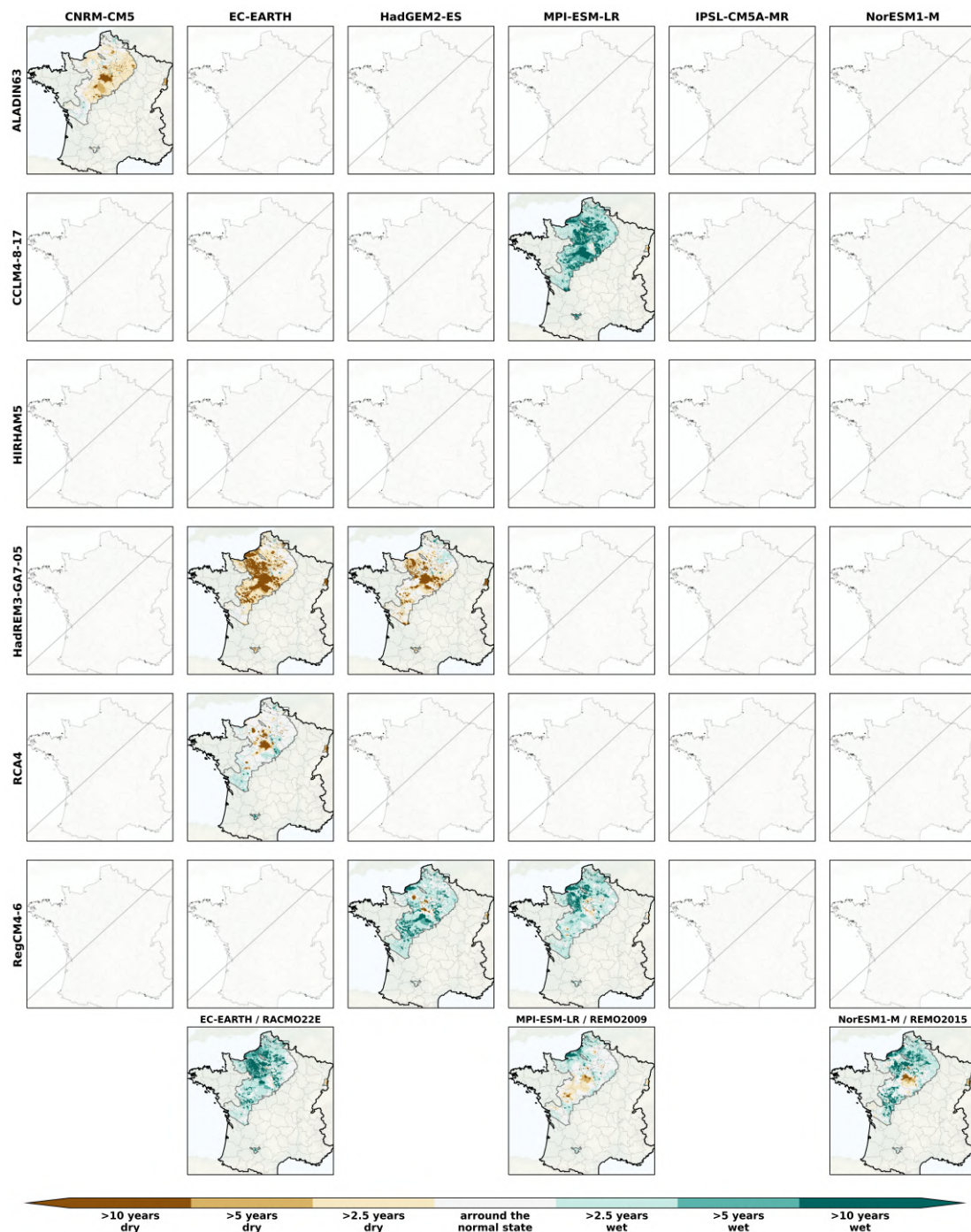
Figure B3. Spatial distribution of the SPLI median over the AquifR domain under the RCP2.6 on the long-term horizon (2071-2099) , following the different GCM (in column) / RCM (in line) combination. The last line corresponds to couples where RCMs are used only once. The missing panels indicate the GCM/RCM couples not included in the EXPLORE2 climate projection dataset.
