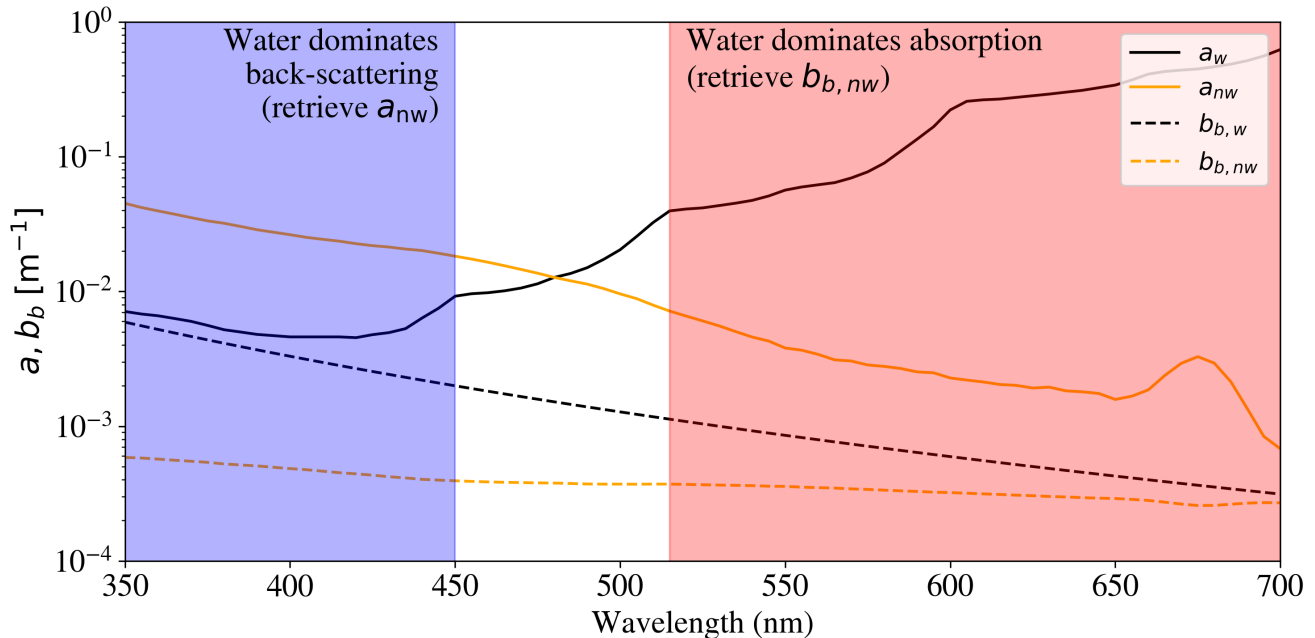
Figure 1. Comparison of the IOP spectra for water ( a_w , b_{b,w} ; black solid and dashed curves) against one example set of non-water spectra ( a_{nw} , b_{b,p} ; orange solid and dashed curves) from L23 (their index=170, an example representative of the open ocean with low Chla concentration). The red region indicates where absorption by water dominates ( a_w > 5a_{nw} ). In this region, reflectance measurements constrain the non-water component of backscattering. Similarly, the blue region is where water dominates backscattering and retrievals may constrain a_{nw} . In turn, for observations with noise, the inversion problem has very limited constraints on the non-water components.
