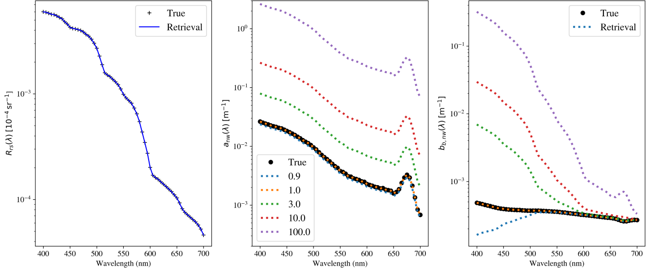
Figure 4. Example of a series of R_{rs}(\lambda) “fits” to an example R_{rs}(\lambda) spectrum (left) for varying a_{nw}(\lambda) (center) and b_{b,p}(\lambda) (right) using the arbitrary IOP model. In this example, we parameterized each with 61 free parameters, one for every wavelength channel. We then altered the non-water absorption spectrum by show a range series of solutions with scaling factors of (0.9, 1., 3., 10., 100.) and derived the spectrum that maintains a perfect solution for relative to the true model for a(\lambda) . Owing to the physical degeneracy in the radiative transfer equation, R_{rs}(\lambda) = F(a/b_b) , there are an infinite number of such solutions yielding an infinite uncertainty in a_{nw}(\lambda) and b_{b,p}(\lambda) .
