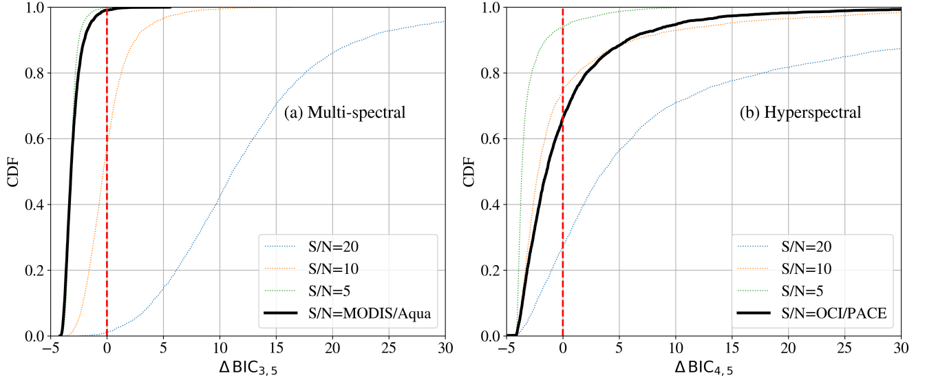
Figure 6. Evaluations of the difference in BIC values \Delta BIC for fits to reflectance data derived from the 3,320 spectra of L23. The curves describe the cumulative distribution function (CDF) of the \Delta BIC values. The left panel is for (a) simulated MODIS observations (8 bands) with a series of signal-to-noise (S/N) assumptions (colored curves) and for retrievals adopting actual MODIS noise estimates from NASA validation Werdell and Bailey (2002). The > 99\% negative \Delta BIC_{3,5} values for the realistic noise case indicates the L23 spectra greatly favor models with only 3 parameters and without phytoplankton. right panel Similar (b) similar analysis but for OCI/PACE-simulated observations with fixed S/N and for a best guess at nominal OCI/PACE performance (Section 2.3). We find even with OCI that only \approx 30\% of the L23 dataset favors the model with phytoplankton.
