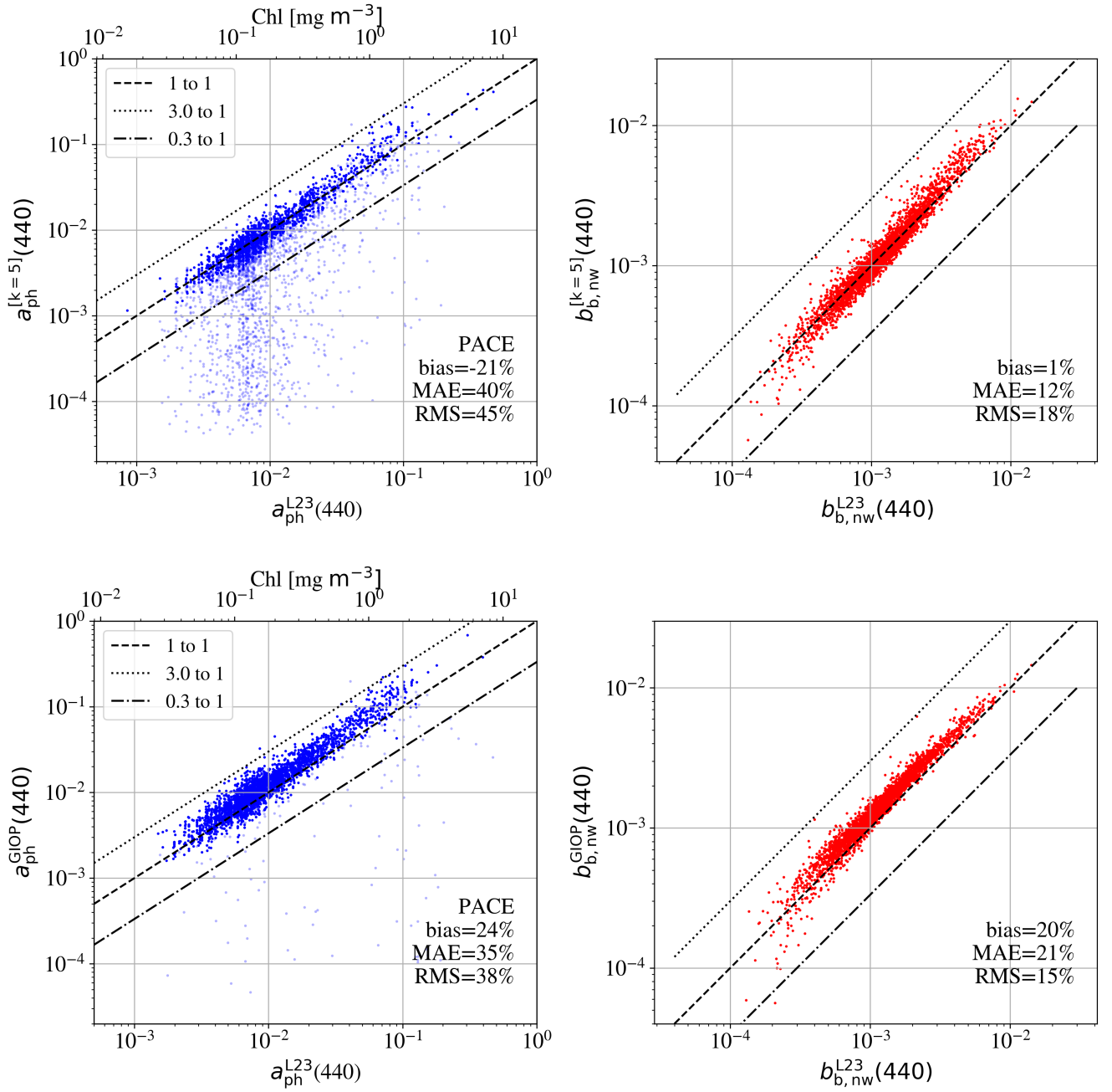
Figure 11. The left panels show the retrievals of a_{ph}(440\text{nm}) for simulated PACE spectra against the true values of for the [k = 5] (top) and GIOP models (bottom) using the BING package. When the error on a_{ph}(440\text{nm}) exceeds three times the best value, we plot the measurement in light blue. The dashed curve is the 1:1 line. The right panels show the retrievals for the particulate backscattering at 440 nm. The bias, median absolute error (MAE), and root mean square (RMS) are indicated in each panel.
