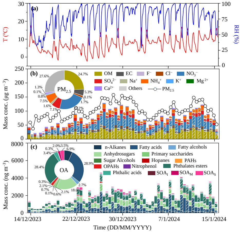
Figure 1: Time series of (a) temperature (T) and relative humidity (RH), (b) concentrations of PM 2.5 , OM, EC, and inorganic ions, and (c) concentrations of OA compounds (SOA 1 : isoprene SOA tracers, SOA M : monoterpene SOA tracers, SOA S : sesquiterpene SOA tracers).
