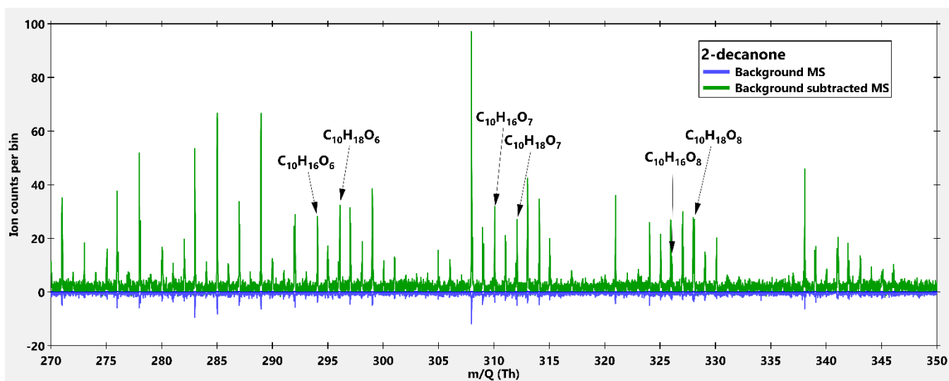
360 Figure A6. High resolution mass spectra (MS) of 2-decanone + OH. Blue MS is the background while the green MS is the background 361 subtracted MS. The background MS is multiplied by a factor of -1 for visualization reasons.
