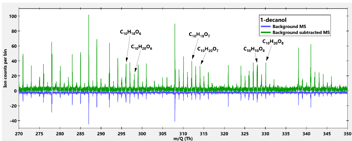
365 Figure A7. High resolution mass spectra (MS) of 1-decanol + OH. Blue MS is the background while the green MS is the background 366 subtracted MS. The background MS is multiplied by a factor of -1 for visualization reasons.
