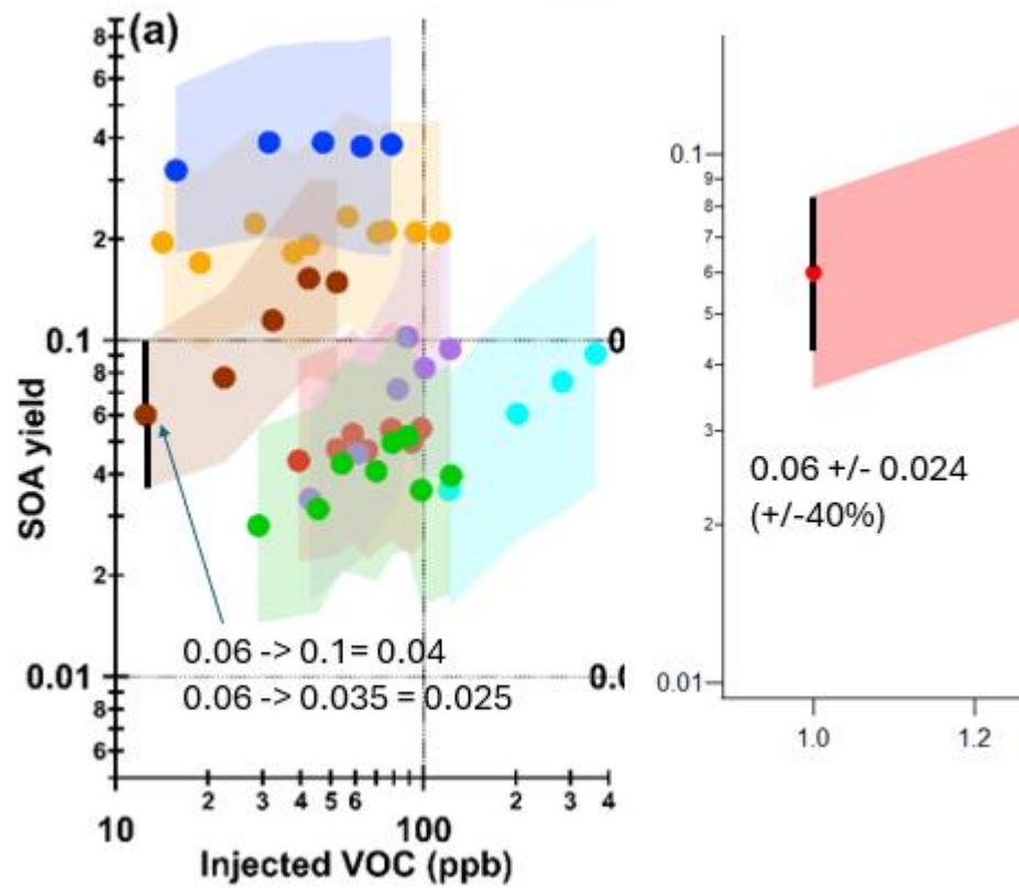
Figure 1: Left: part of Figure 1 with added lines to highlight shape of shaded error area. Right: depiction of a symmetrical error in log space for a similar value.
