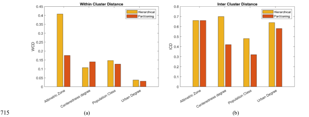
715 Figure 8 – Comparison of clustering algorithms in terms of WCD i (a) and ICD i (b).
