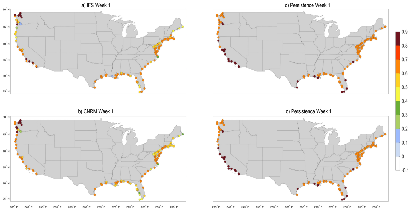
40 Figure S1. Year-round (2000-2017) week 1 anomaly correlation skill between (a) IFS and (b) CNRM hindcast SSH anomalies and NOAA gauge station water level anomalies, and persistence skill for IFS and CNRM hindcast days, (c) and (d), respectively. While the sample years used in the anomaly correlation calculation (2000-2017) are the same, the dates are slightly different because of different initialization dates. All dates are used in both datasets, regardless of whether they overlap with the other dataset, because otherwise there are too few samples. The high similarity between the damped persistence 45 forecasts in panels (c) and (d) suggests that the slightly different sampling days does not strongly affect the assessment of skill for the 2000-2017 period, and thus the IFS and CNRM hindcasts for the 2000-2017 shown here can be fairly compared.
