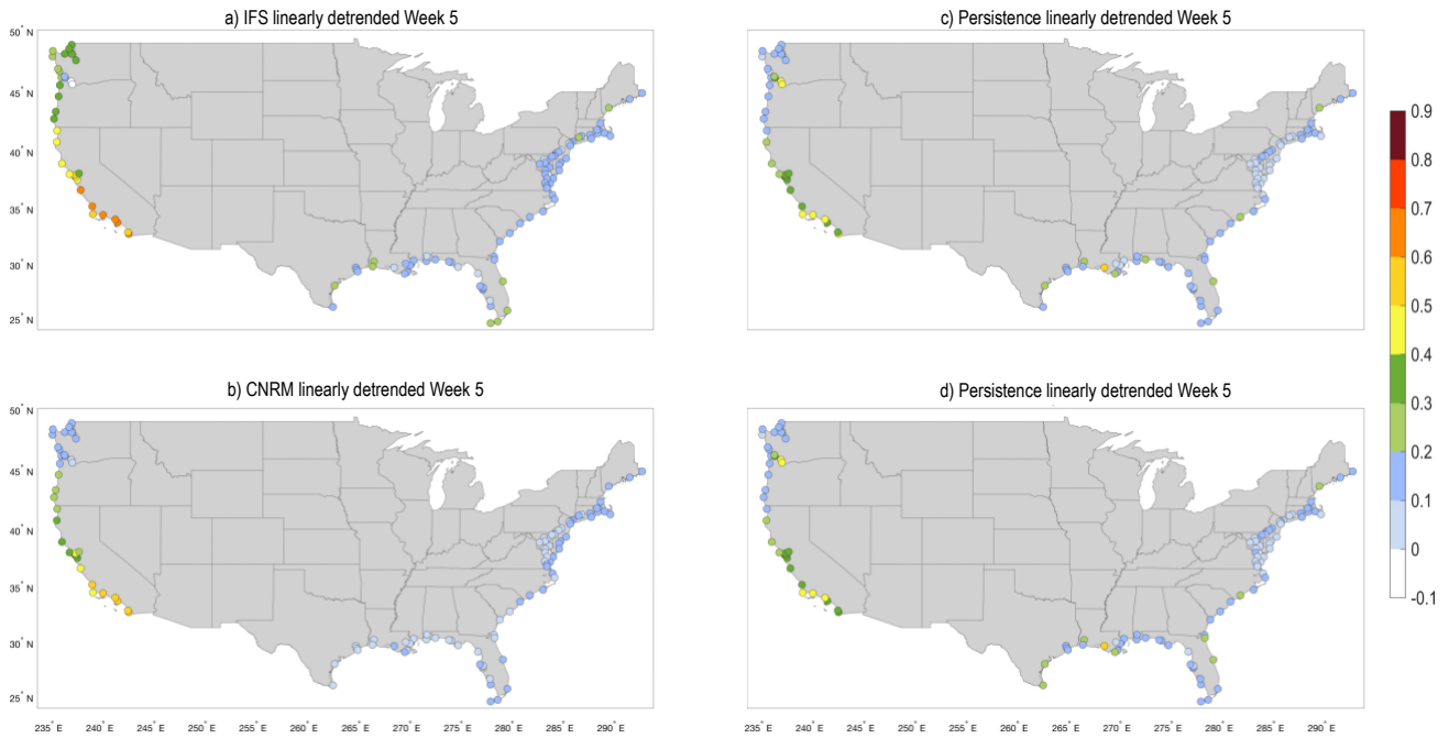
Figure S10. Year-round (2000-2017) week 5 anomaly correlation skill between linearly detrended (a) IFS and (b) CNRM hindcast SSH anomalies and linearly detrended NOAA gauge station water level anomalies, and linearly detrended persistence skill for IFS and CNRM hindcast days, (c) and (d) , respectively. While the sample years used in the anomaly correlation calculation (2000-2017) are the same, the dates are slightly different because of different initialization dates. All dates are used in both datasets, regardless of whether they overlap with the other dataset, because otherwise there are too few samples. The high similarity between the damped persistence forecasts in panels (c) and (d) suggests that the slightly different sampling days does not strongly affect the assessment of skill for the 2000-2017 period, and thus the IFS and CNRM hindcasts for the 2000-2017 shown here can be fairly compared.
