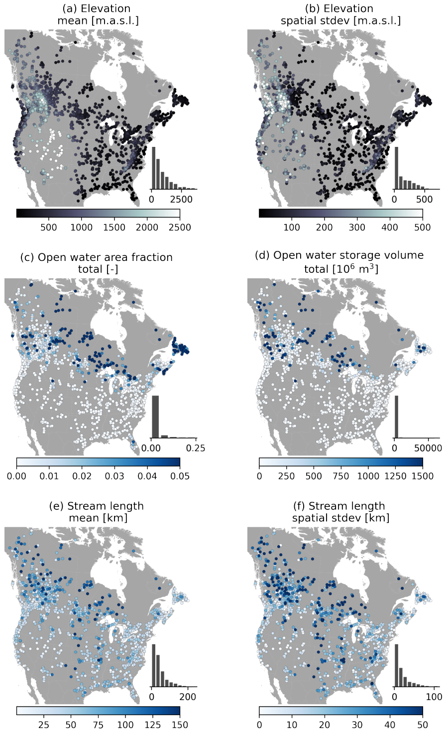
Figure 6. Selection of topographic attributes. Open water (c, d) estimates are obtained from the HydroLAKES database which uses a threshold of 10 ha ( 0.1 \text{ km}^2 ) for lake and reservoir identification. (e, f) Stream length statistics are derived by starting at each headwater sub-basin upstream of a given gauge, and tracing the flow path down until the gauge location is reached. From this ensemble of flow path lengths upstream of a given gauge, the mean and standard deviation of stream lengths are calculated.
