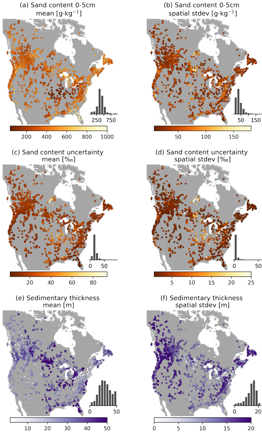
Figure 8. Selection of subsurface attributes. (a-d) Properties derived from the SOILGRIDS 2.0 data set through spatial averaging for each catchment. (a, b) Mean and spatial standard deviation of sand content in the top SOILGRIDS layer. (c, d) Mean and spatial standard deviation of sand content uncertainty, defined as the ratio between the 90-percentile prediction interval and the median prediction \left( \frac{Q_{95} - Q_{05}}{Q_{50}} \right) . (e, f) Mean and spatial standard deviation of sedimentary deposit thickness estimates in the Pelletier data set.
