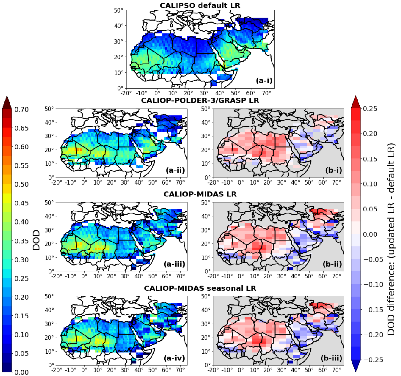
Figure 9: Geographical distributions of the annual Dust Optical Depth (DOD) at 532 nm based on (a-i) the CALIPSO default LR, (a-ii) the LR from the CALIOP-POLDER-3/GRASP synergy and (a-iii, a-iv) the annual and seasonal LR from the CALIOP-MIDAS synergy. The DOD differences between the CALIPSO default product and the DODs derived from the synergies of (b-i) CALIOP-POLDER-3 and (b-ii, b-iii) CALIOP-MIDAS are also presented in the right column.
