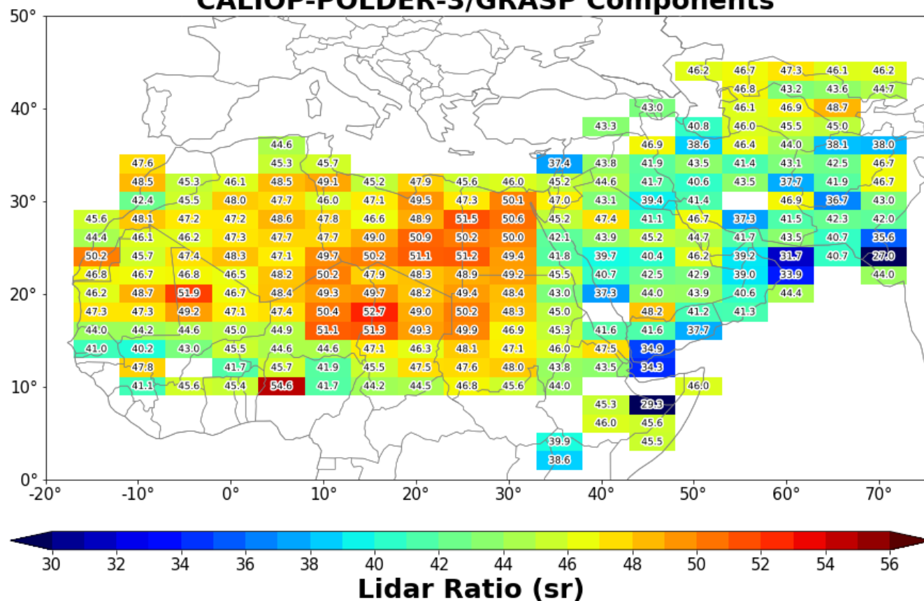
Figure 5: Geographical distribution of dust Lidar Ratio (LR) resulted via the synergy of CALIOP and POLDER-3/GRASP. The values represent the mean LR at each 2°x5° predefined grid.
