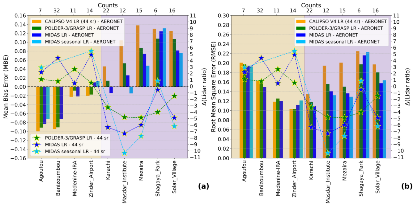
Figure 8: Bar plots of the: (a) Mean Bias Error (MBE) and (b) Root Mean Square Error (RMSE), resulted from the comparisons between AERONET and CALIOP DOD by applying the default CALIPSO dust LR of 44 sr (orange bars), the updated LR from the synergy between CALIOP-POLDER-3/GRASP synergy (green bars), and the updated LR from the annual and seasonal synergy between CALIOP-MIDAS synergy (blue bars and cyan bars, respectively) on CALIOP's backscatter retrievals. On the bottom x-axis the AERONET stations used in the evaluation are presented, while on the top x-axis are shown the counts of the dust cases used for the derivation of the metrics per station. The right y-axis represents the LR_{diff} between the CALIOP default dust LR (44 sr) versus the dust LR from the synergies of CALIOP-POLDER-3/GRASP (green stars) and CALIOP-MIDAS (blue stars for annual; cyan stars for seasonal), respectively.
