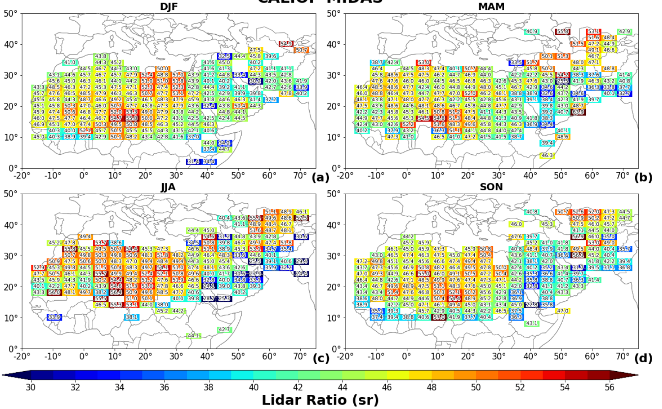
Figure 7: Seasonal geographical distributions of dust Lidar Ratio (LR) for (a) DJF, (b) MAM, (c) JJA and (d) SON resulted via the synergy of CALIOP and MIDAS. The values represent the mean LR at each 2°x5° predefined grid.
