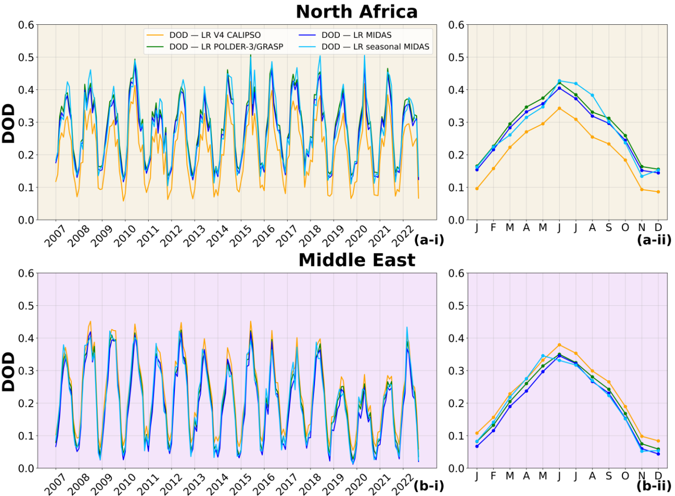
660 Figure 11: Interannual (i) and intra-annual (ii) variability of Dust Optical Depth (DOD) at 532 nm, representative for the period 2007–2022, regionally averaged over (a) North Africa and (b) Middle East. The orange color represents the DOD computed with the CALIPSO default LR, while green, blue and cyan colors correspond to the updated LR values based on CALIOP-POLDER-3/GRASP and CALIOP-MIDAS annual and seasonal synergies, respectively.
