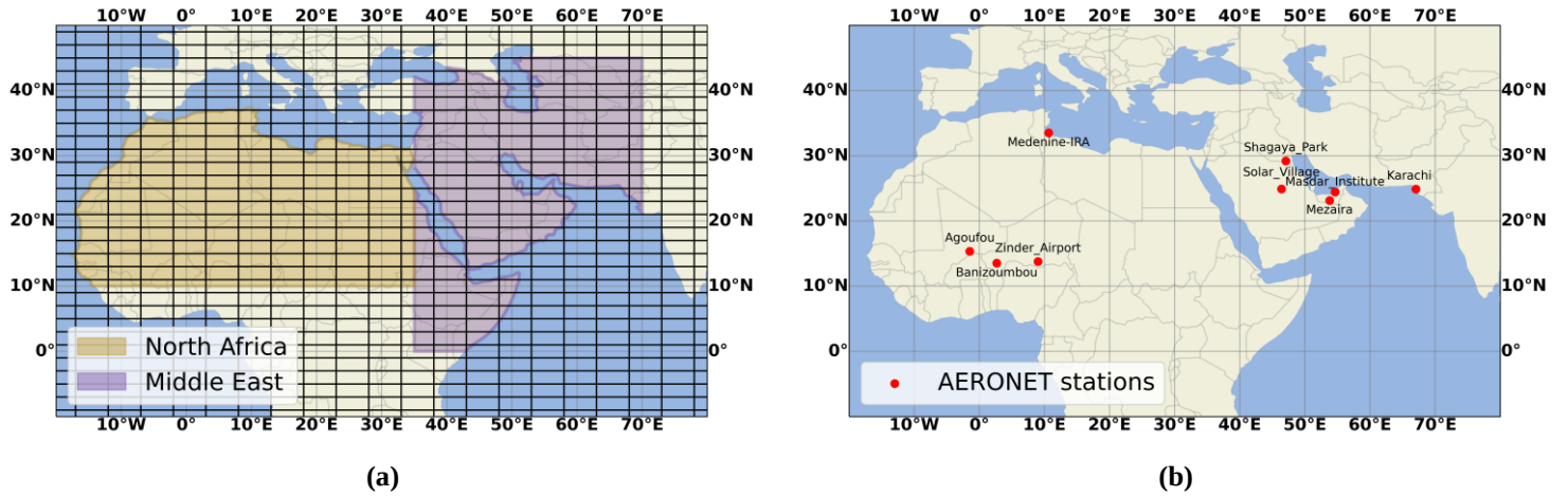
Figure 1: (a) The North Africa (yellow-shaded area) and Middle East (purple-shaded area) desert regions as defined based on Ginoux et al. (2012). The domain is divided into grids with 2°x5° spatial resolution grids based on Winker et al. (2013) in order to minimize the signal error in CALIPSO mean profiles, and (b) the AERONET stations over North Africa and Middle East used for evaluating CALIOP DODs.
