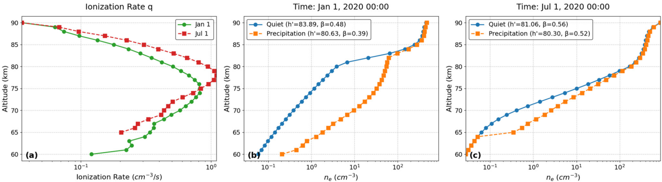
440 Figure 7: Illustration of seasonal variations in electron density and reflection height at latitude 52.5° N, longitude -90° E ( L \approx 5 ). (a) Ionization rate at 00:00 LT on January 1 and July 1, 2020. (b, c) Electron density profiles during quiet conditions and after same stable particle precipitation on January 1 and July 1, 2020, respectively.
