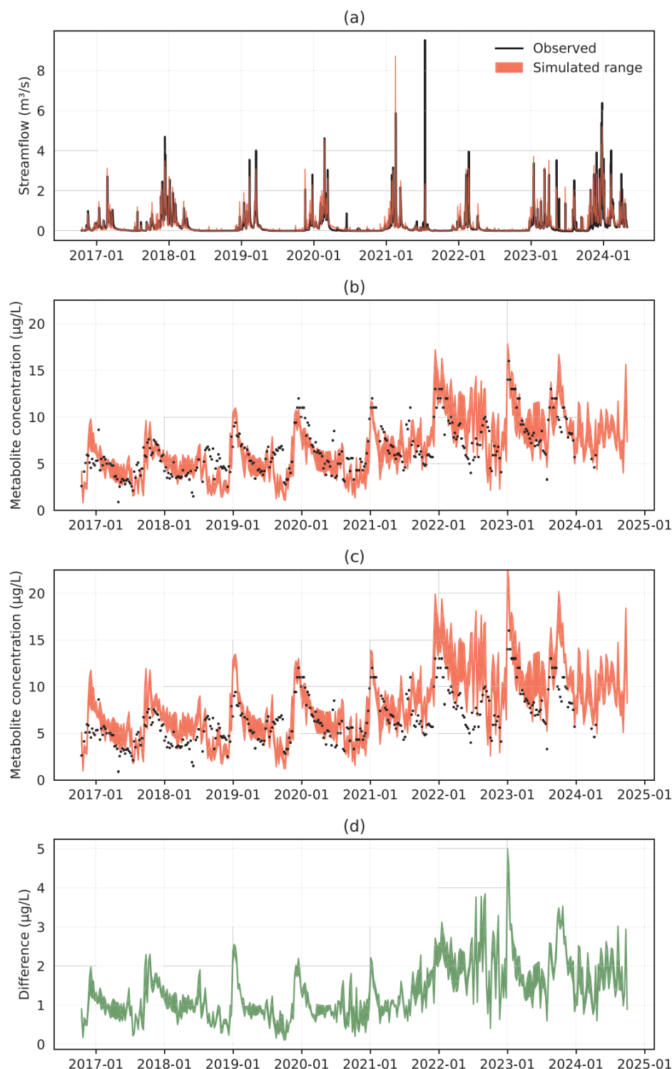
345 Figure 2: Catchment 1 (C1) time series (Jun 2016 – Oct 2024) for observed and simulated discharge (a), metabolite concentration with plant uptake (b), metabolite concentration without plant uptake (c), and the difference between (c) and (b)
