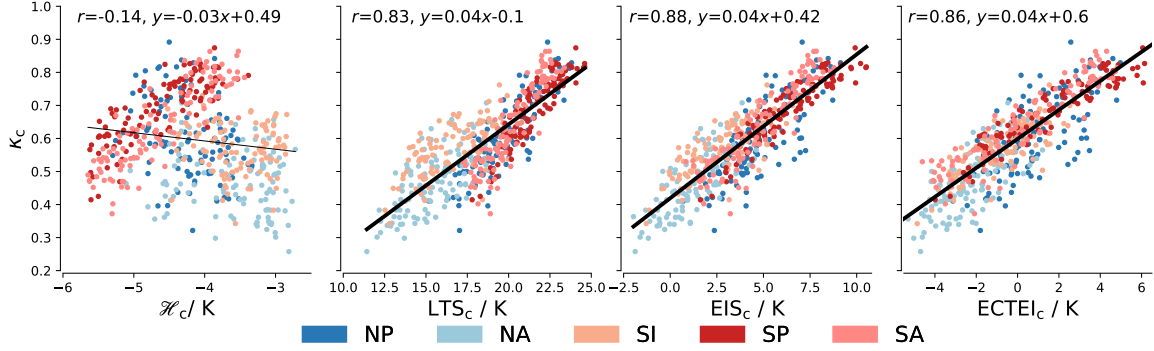
Figure 2. Scatter plots of different cloud controlling factors and low cloud fraction ( \kappa ) from 2003 to 20112014. Each scatter point represents a monthly mean, and the plots include 9 years of data, covering all 12 months per year. From left to right, the cloud controlling factors are \mathcal{H} , LTS, EIS, ECTEI, analyzed over the cloud (c) areas, as denoted by subscript. All subplots share the same y-axis, which represents \kappa , with each plot displaying data points colored by different regions. Regression lines are presented for p-values \leq 0.05 , and thickened when r^2 \geq 0.25 .
