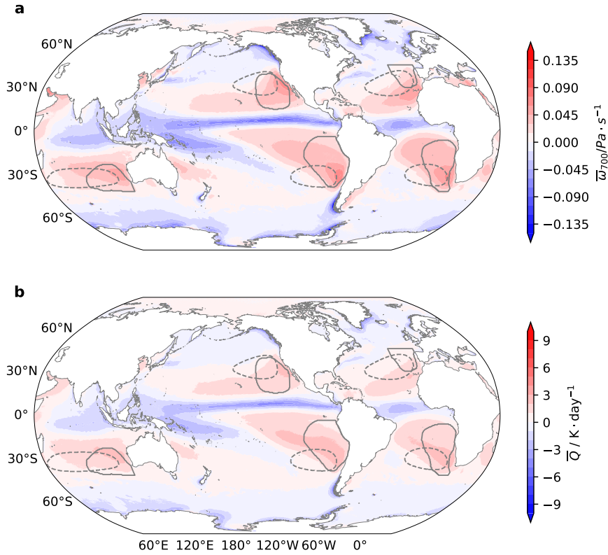
Figure 4. Map of 1985–2014 climatological mean \omega_{700} (topleft) and \bar{Q} (bottomright). Subtropical high areasStratocumulus regions are shown by dashed lines and cloud-regions are outlined by solid lines.
