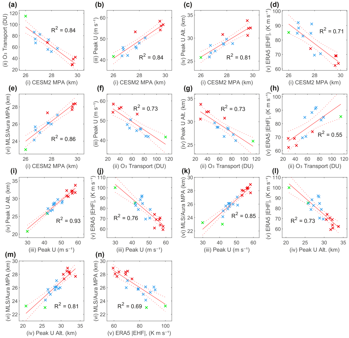
Figure A4. The relationship between dynamical proxies and ozone ( O_3 ) transport. Linear fits are performed between (i) CESM2 MPA (km) for 2005–2018, (ii) CESM2 horizontal O_3 transport between 70^\circ S – 90^\circ S from 17–27 km (DU) for 2005–2018, (iii) the average Sept.–Oct. strength of the peak 45^\circ S – 75^\circ S MERRA-2 zonal wind (U) ( m s^{-1} ) for 2004–2024, (iv) the average Sept.–Oct. altitude of the peak 45^\circ S – 75^\circ S MERRA-2 zonal wind (U) (km) for 2004–2024, (v) the magnitude of the Mar.–Oct. accumulated ERA5 eddy heat flux ( |EHF| ) ( K m s^{-1} ) for 2004–2023, and (vi) observed MLS/Aura MPA (km) for 2004–2024. Red lines show the result from each fit and its 95% confidence bounds. The corresponding R^2 value is given. Years are colour-coded according to the categories in Table 1: Green = Minor, Blue = Moderate, and Red = Major ozone holes.
