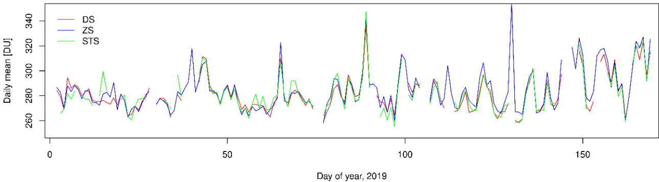
Figure 3: Series of daily mean. Both the ZS and STS TOC measurements correlate well with the DS reference measurements. It is worth noticing that on days with missing reference data the ZS measurements are usually higher than the mean value from the DS measured before and after the days of missing values. This is clearly seen around day 40, 112, and 130.
