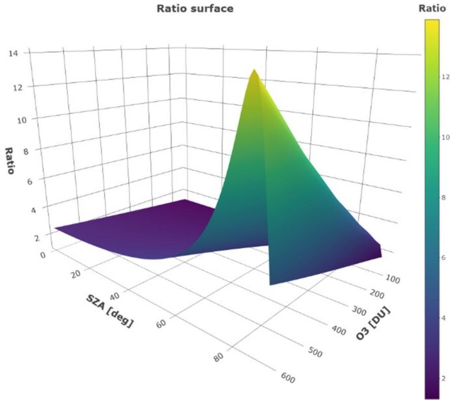
170 Figure 1: The resulting surface from the linearly interpolated LUT values.
