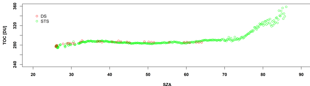
Figure 7: When the SZA approaches 70°, the detection level is almost reached, and the model predicts this as a false increase in TOC as the 312.2 nm intensity disappears earlier than expected.
