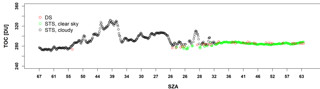
250 Figure 5: This shows a typical plot with cloudy conditions before noon where the STS TOC measurements are increased and highly varying. During afternoon the variation is reduced, resulting in better agreement with the Brewer DS measurements.
