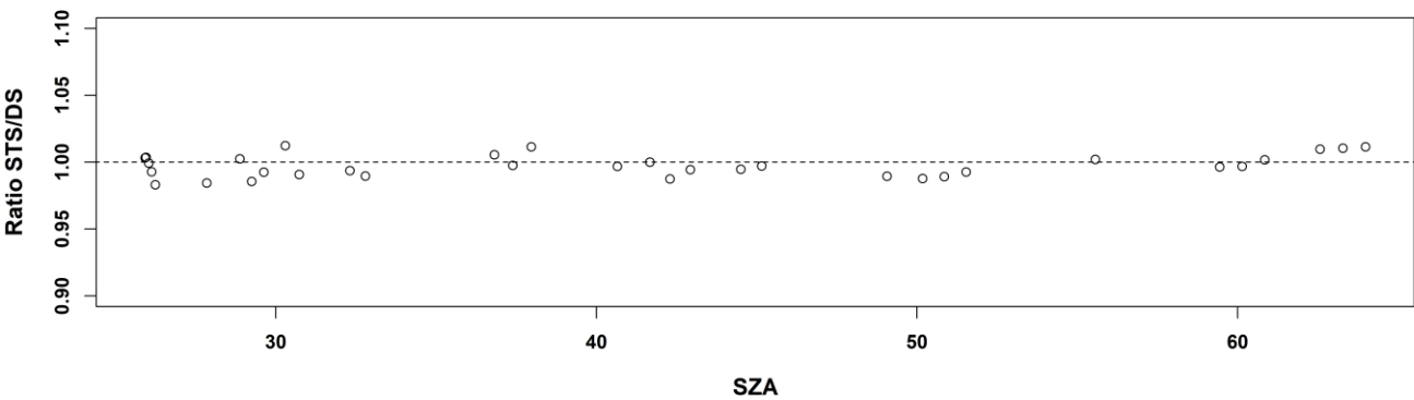
305 Figure 8: The circles indicate the ratio between the STS TOC and DS measurements during day 49 from noon and on. The maximum deviation is 1.7 % and the standard deviation is 0.8 %.
