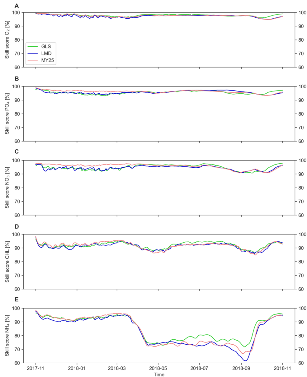
Fig. S3: Time series of skill scores (SSs) [%] for key biogeochemical tracers for the x10 time-step simulation, comparing offline and online runs using the Generic Length Scale (GLS), Mellor–Yamada 2.5 (MY25), and Large–McWilliams–Doney (LMD) mixing schemes. Panels show (A) dissolved oxygen (O 2 ), (B) phosphate (PO 4 ), (C) nitrate (NO 3 ), (D) chlorophyll (CHL), and (E) ammonium (NH 4 ). Green, blue, and coral lines correspond to GLS, LMD, and MY25 simulations, respectively.
