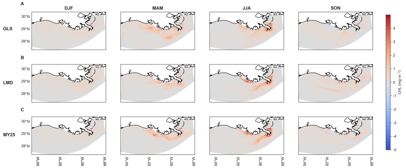
Fig. S5: Mean seasonal differences in chlorophyll concentrations (CHL) at the surface layer. The panels illustrate the differences between offline (x5 DT) and online simulations for each mixing scheme: (A) Generic Length Scale (GLS), (B) Mellor–Yamada 2.5 (MY25), and (C) Large–McWilliams–Doney (LMD). The coolwarm color scale on the right indicates the magnitude of the differences. Seasonal designations are as follows: DJF (December-January-February, winter), MAM (March-April-May, spring), JJA (June-July-August, summer), and SON (September-October-November, fall). This figure highlights the variability in CHL concentrations across different mixing schemes and seasons, providing insight into the performance of the offline simulations relative to the online model.
