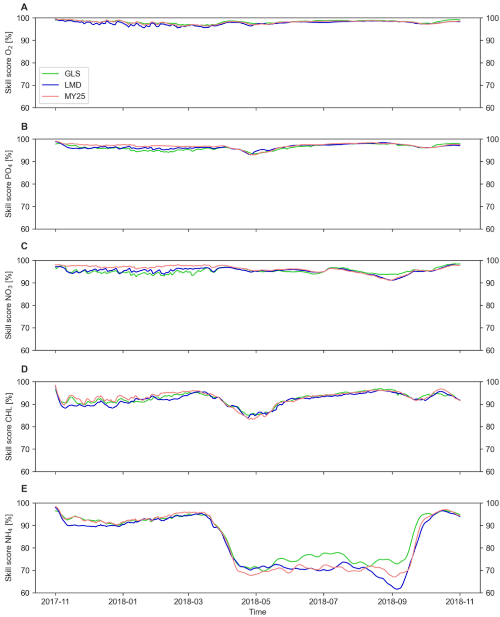
30 Fig. S2: Time series of skill scores (SSs) [%] for key biogeochemical tracers for the x3 time-step simulation, comparing offline and online runs using the Generic Length Scale (GLS), Mellor–Yamada 2.5 (MY25), and Large–McWilliams–Doney (LMD) mixing schemes. Panels show (A) dissolved oxygen ( O_2 ), (B) phosphate ( PO_4 ), (C) nitrate ( NO_3 ), (D) chlorophyll (CHL), and (E) ammonium ( NH_4 ). Green, blue, and coral lines correspond to GLS, LMD, and MY25 simulations, respectively.
