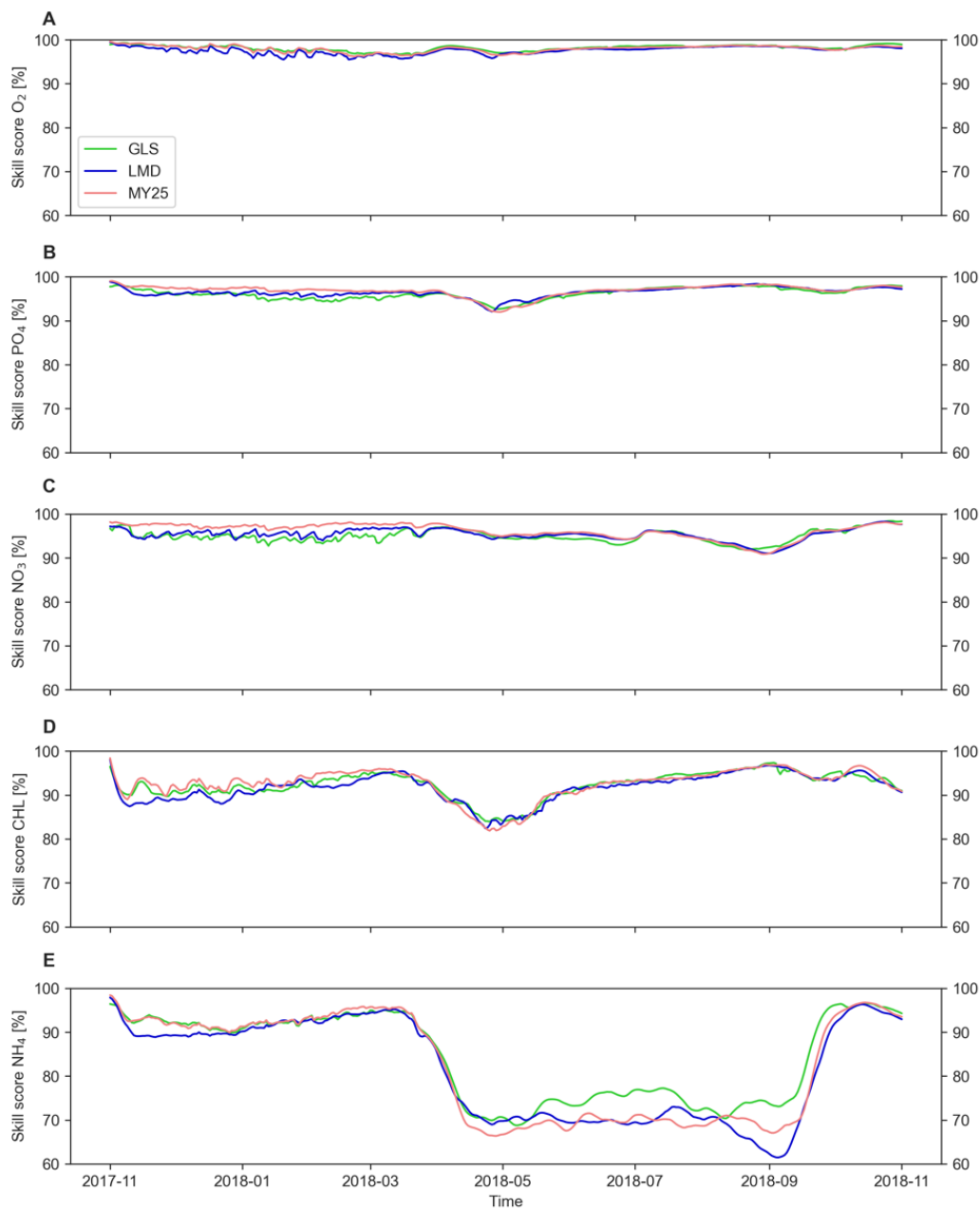
Fig. S1: Time series of skill scores (SSs) [%] for key biogeochemical tracers for the x1 time-step simulation, comparing offline and online runs using the Generic Length Scale (GLS), Mellor–Yamada 2.5 (MY25), and Large–McWilliams–Doney (LMD) mixing schemes. Panels show (A) dissolved oxygen ( O_2 ), (B) phosphate ( PO_4 ), (C) nitrate ( NO_3 ), (D) chlorophyll (CHL), and (E) ammonium ( NH_4 ). Green, blue, and coral lines correspond to GLS, LMD, and MY25 simulations, respectively.
