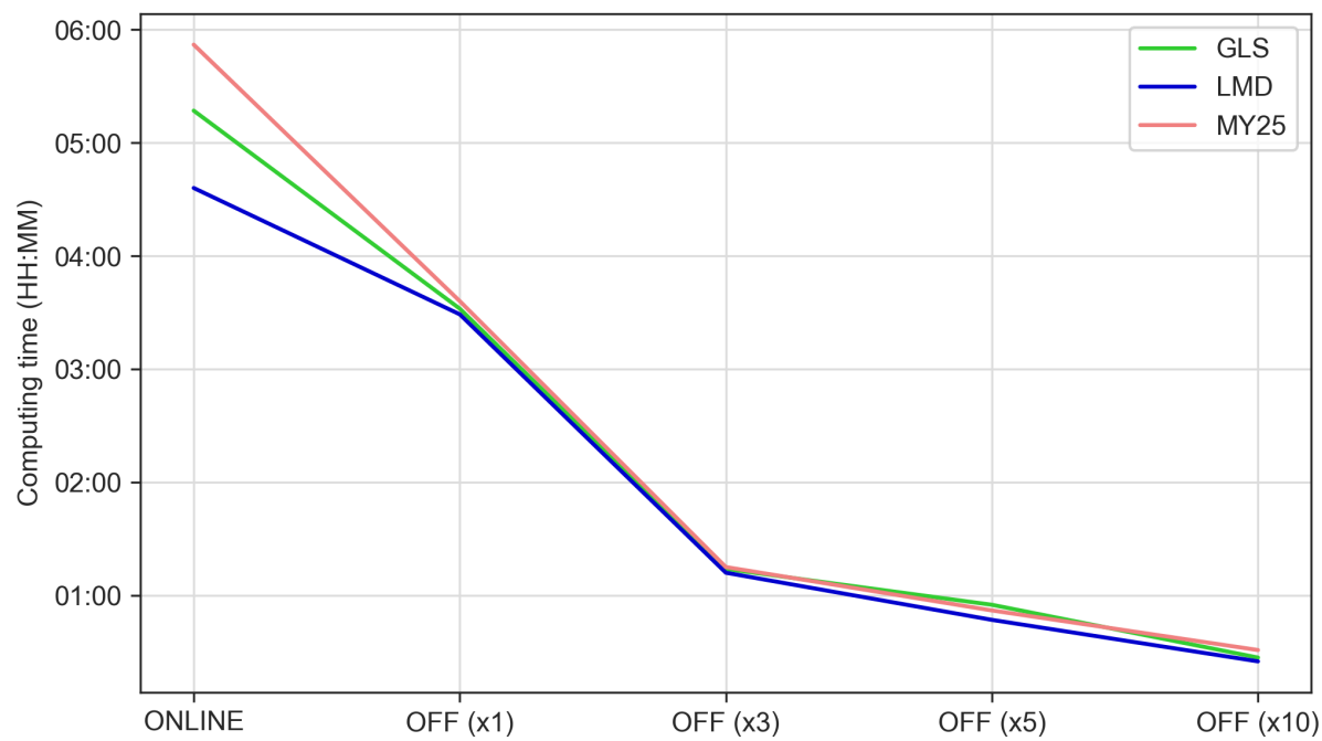
485 Figure 11: Computing time (hh:mm) for online and offline simulations across each configuration, considering the three mixing schemes. The color coding corresponds to the mixing schemes: green for Generic Length Scale (GLS), blue for Large-McWilliams-Doney (LMD), and red for Mellor-Yamada 2.5 (MY25). The label ONLINE refers to the coupled simulation, while the labels "OFF (x1)", "OFF (x3)", "OFF (x5)", and "OFF (x10)" indicate the respective offline simulations with the time steps multiples used.
