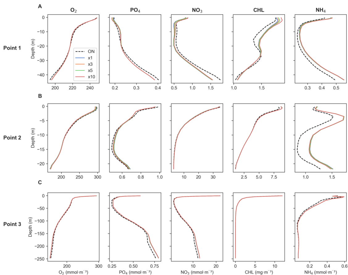
Figure 8: Time-averaged profiles of key biogeochemical tracers' concentrations for Generic Length Scale (GLS) mixing simulations.
