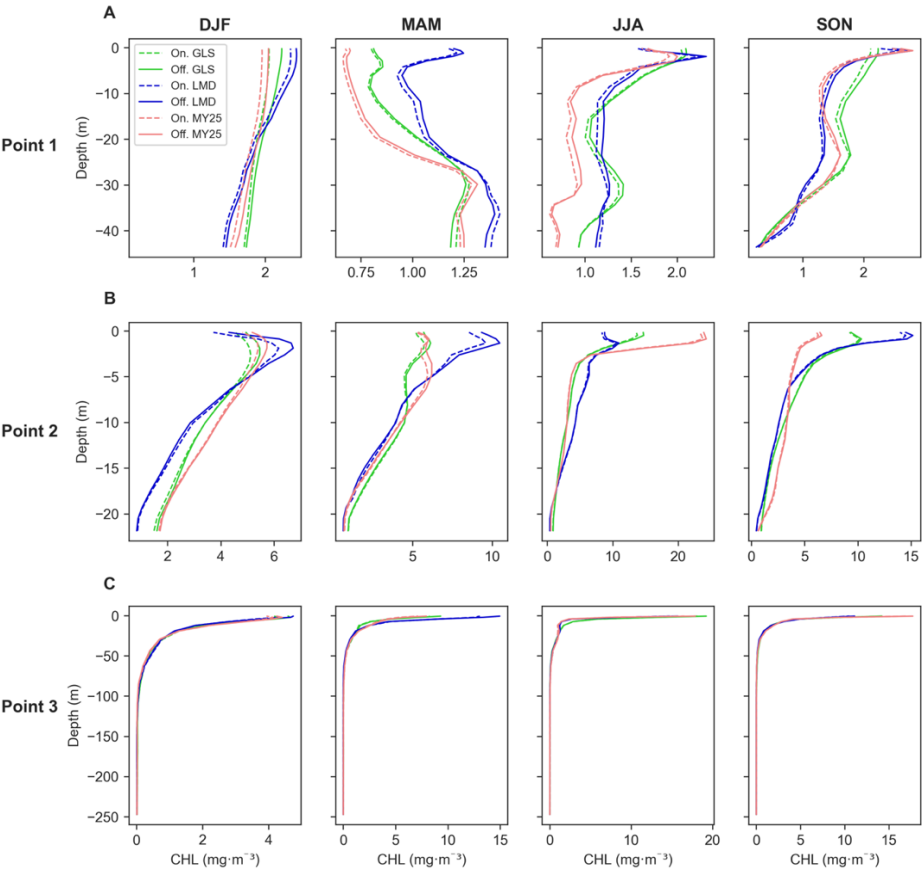
465 Figure 10: Seasonal-averaged chlorophyll concentration (CHL) profiles for offline (x5 time step, solid line, Off.) and online simulations (dashed line, On.) across different mixing schemes. Panels display data for: (A) Point 1, located offshore in the western part of the study area; (B) Point 2, situated near the mouth of the Atchafalaya River; and (C) Point 3, located near the mouth of the Mississippi River. Refer to Figure 1 for specific point locations. The green, blue, and red lines represent the Generic Length Scale (GLS), Large-McWilliams–Doney (LMD), and Mellor-Yamada 2.5 (MY25) mixing schemes, respectively. Seasonal designations are as follows: DJF 470
