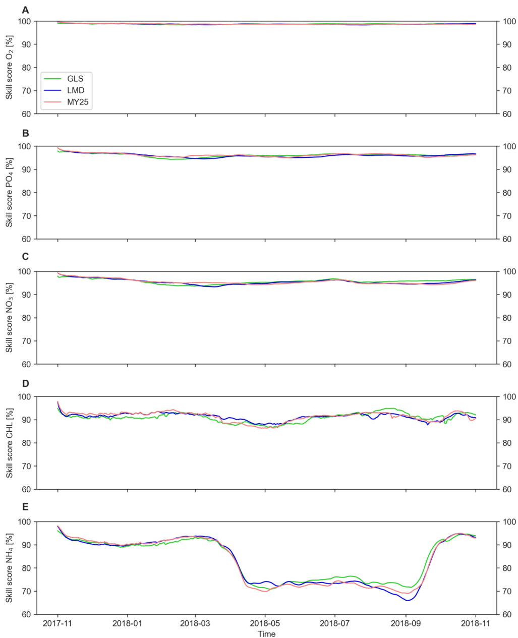
Figure 3: Time series of volume-weighted skill scores (SSs) [%] for key biogeochemical tracers during the x5 time-step simulation.
