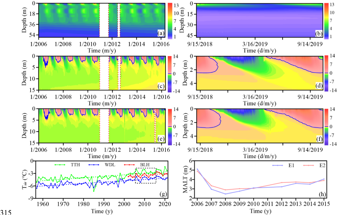
Figure 9: Contour maps of the ground temperature in borehole L A (a), E 1 (c), E 2 (e), L B (b), S 1 (d), and S 2 (f), respectively; (g) air temperature in BLH (built in 2002), WDL, and TTH meteorological stations; (h) variation in MALT at E 1 and E 2 , respectively; the areas marked by the red dashed lines (a, c, and e), black dashed line (g) and blue line (c–f) represent missing data, air temperature during 2006–2015, and temperatures equal to 0°C, respectively.
