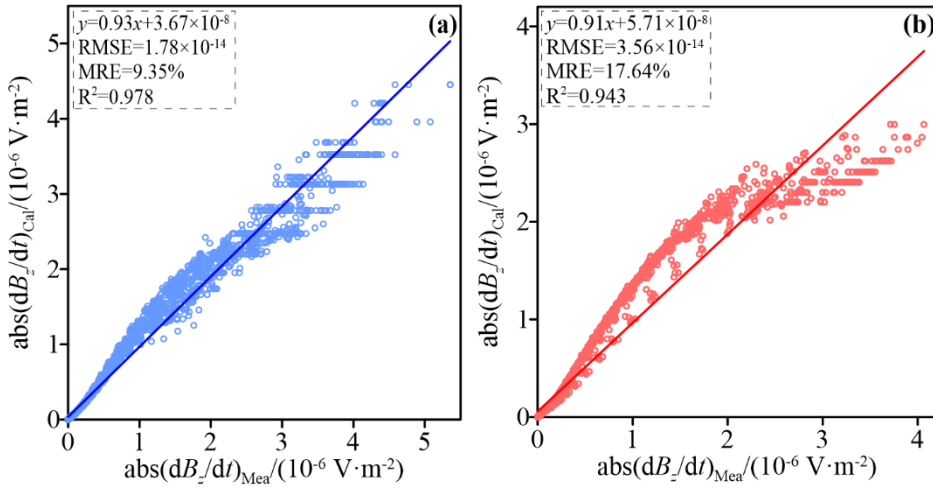
290 Figure 5: Comparison between calculated ((dBz/dt)Cal) and measured ((dBz/dt)Mea) induced electromotive forces for TE1 (a) and TE2 (b) transects, where the blue and red lines represent the fitting lines.
