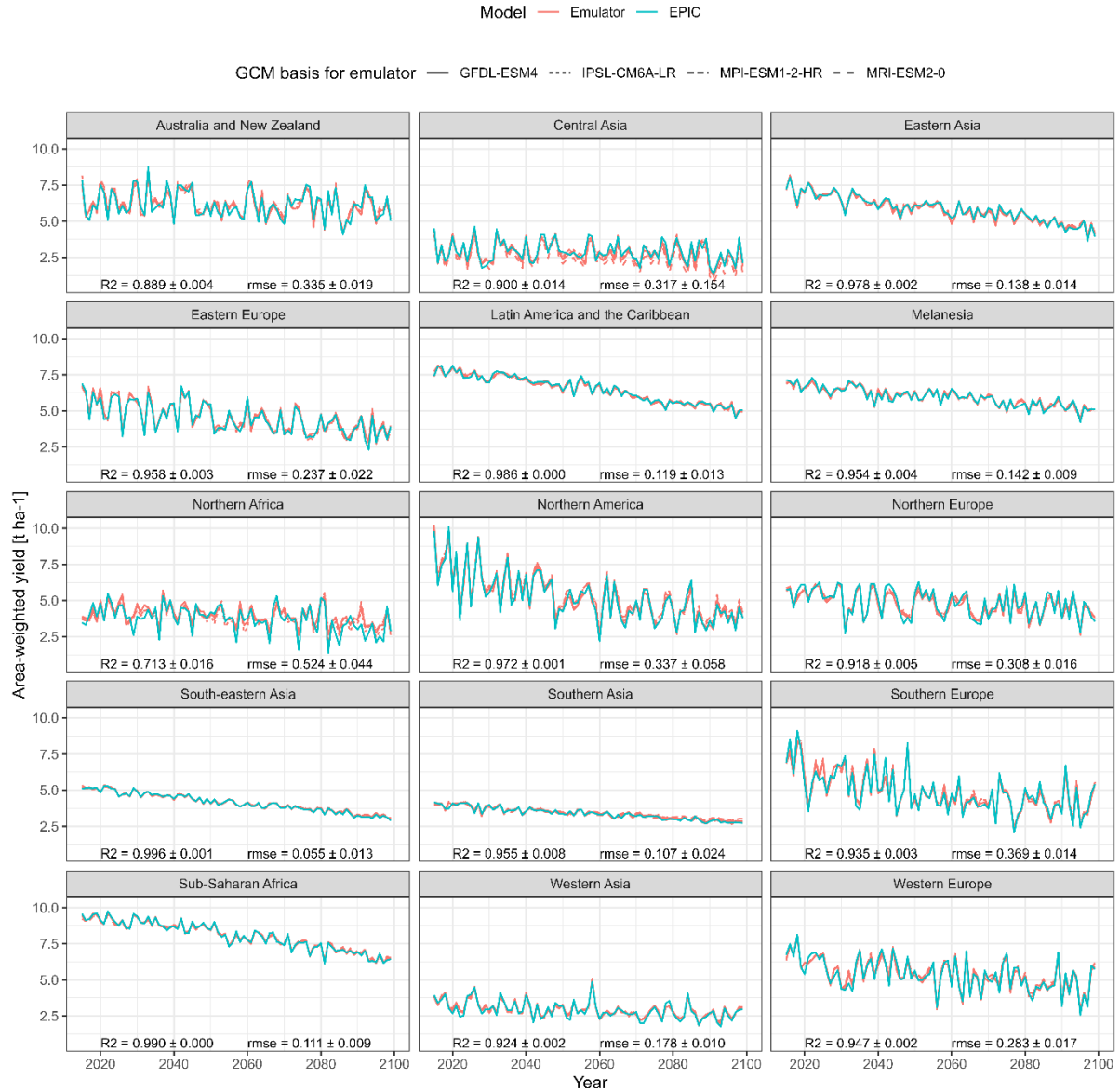
Figure 5. Same as Figure 4 but for 15 macro regions and target climate dataset UKESM1-0-LL x SSP585 only.
