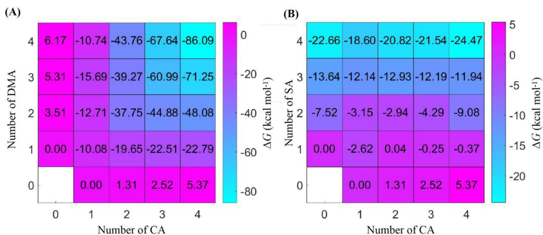
Figure 2. The formation free energy ( \Delta G ) (in \text{kcal mol}^{-1} ) of (A) (CA) 1-4 (DMA) 1-4 and (B) (CA) 1-4 (SA) 1-4 clusters at the DLPNO-CCSD(T)/aug-cc-pVTZ// \omega B97X-D/6-31++G(d,p) level of theory. The calculations are performed at 278 K and 1 atm.
