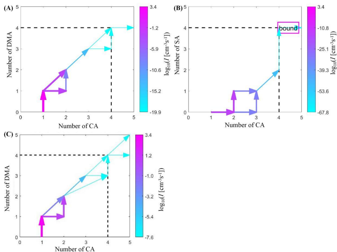
Figure 6. (A) Main clustering pathways of (CA) 1-4 (DMA) 1-4 clusters at 278 K, [CA] = 10^6 \text{ cm}^{-3} , and [DMA] = 5 ppt. (B) Main clustering pathways of (CA) 1-4 (SA) 1-4 clusters at 278 K, [CA] = 10^6 \text{ cm}^{-3} , and [SA] = 10^6 \text{ cm}^{-3} . (C) Main clustering pathways of (CA) 1-4 (DMA) 1-4 clusters at 238 K, [CA] = 10^6 \text{ cm}^{-3} , and [DMA] = 5 ppt.
