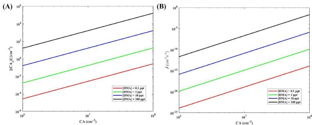
Figure 4. Simulated steady-state CA dimer concentration \sum[(\text{CA})_2] (\text{cm}^{-3}) (A) and the cluster formation rates J (\text{cm}^{-3} \text{s}^{-1}) out of the simulation systems (B) as a function of [\text{CA}] at 278 K.
