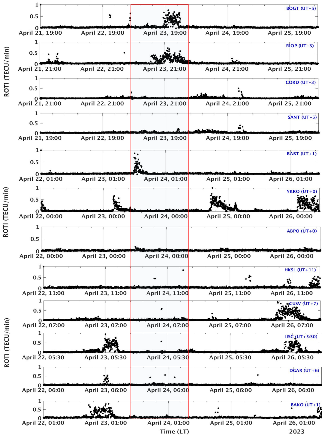
Figure 8. Local time variation of ionospheric ROTI during April 22-25, 2023 storm.
