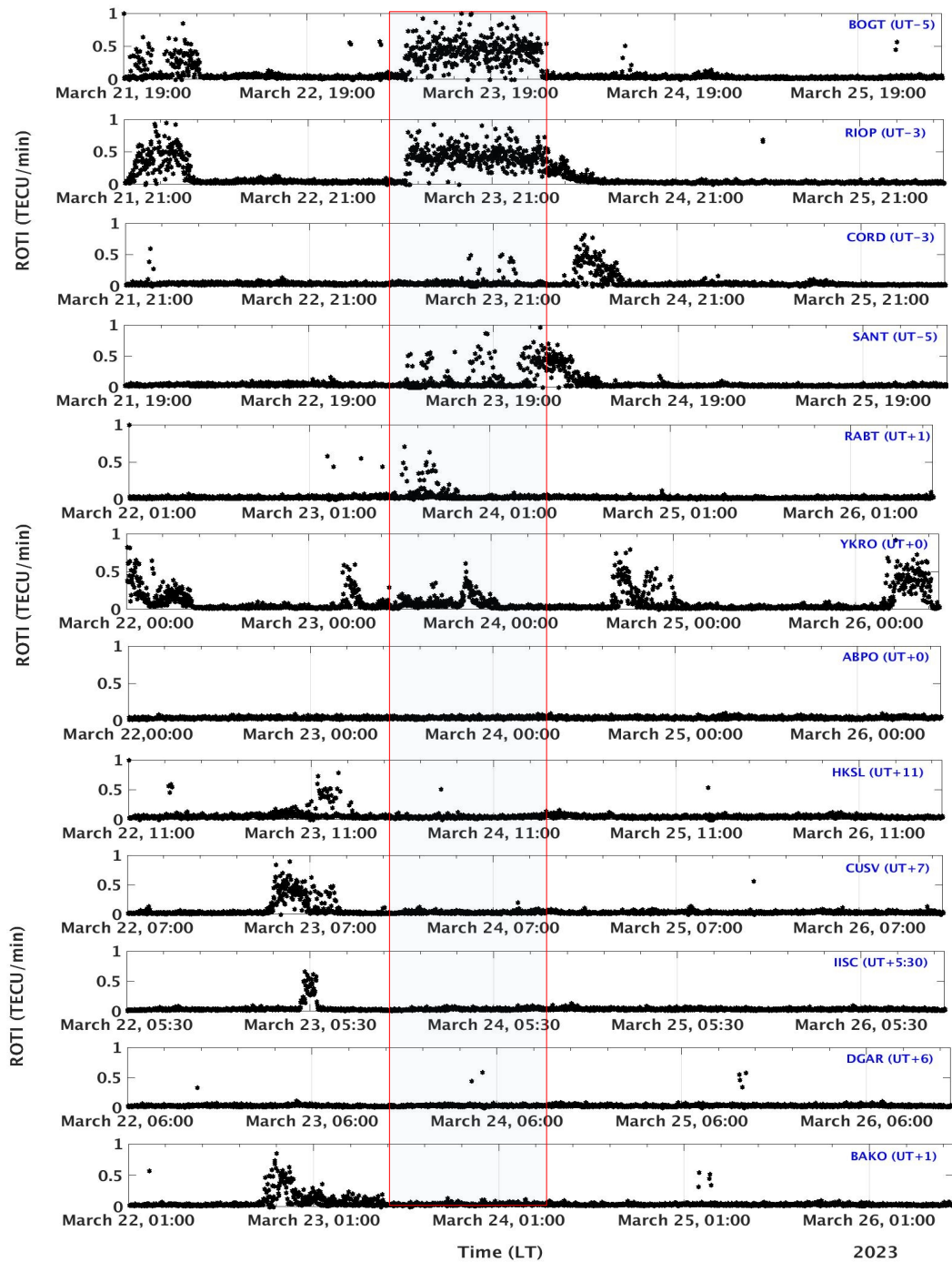
Figure 7. Local time variation of ionospheric ROTI during March 22-25, 2023 storm.
