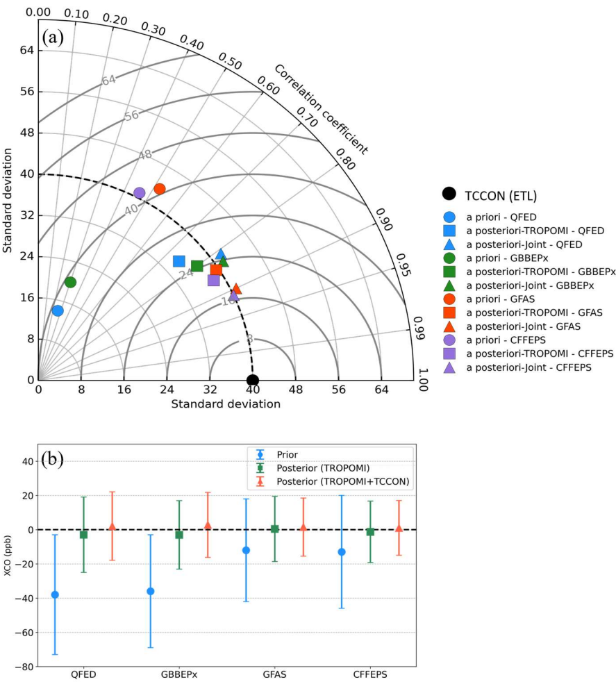
760 Figure 11: Taylor diagram for evaluation of the assimilation and a priori model using four different biomass burning inventories against TCCON XCO measurements at East Trout Lake (ETL) between May and September 2023. (a) Assimilation is performed using TROPOMI-only (square) and joint TROPOMI and TCCON (triangle) data, while their correlations and standard deviations are compared with the model a priori (coloured circles) and XCO measurements (black circle). (b) Evaluation of the mean bias and error of the priors (blue), assimilation using TROPOMI-only (green), and assimilation using a joint TROPOMI and TCCON (red).
