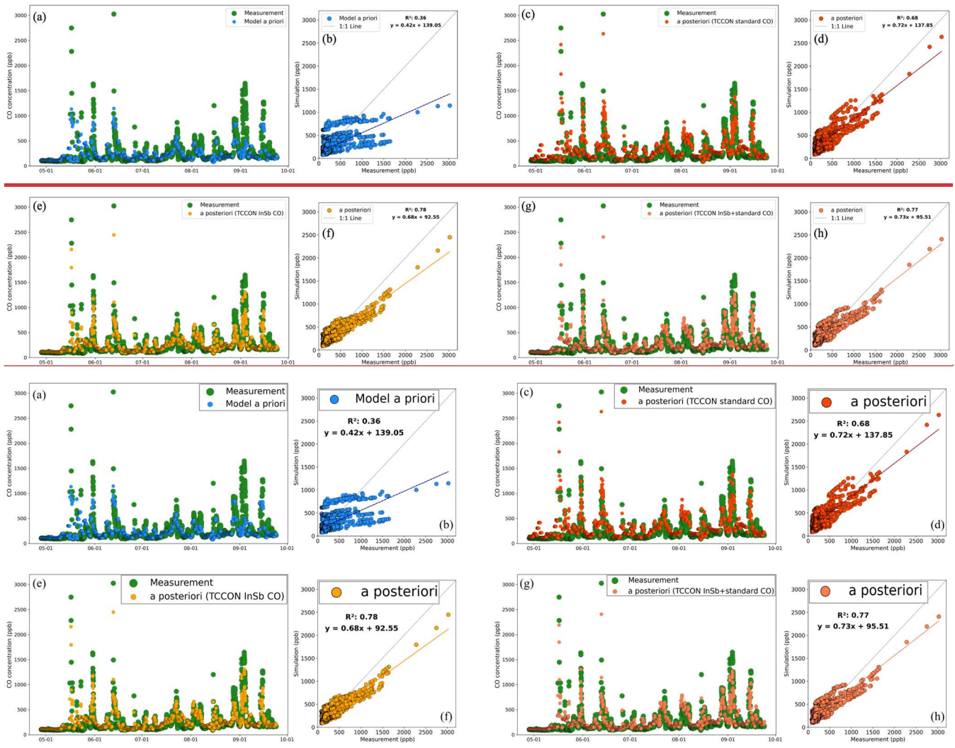
Figure 12: Evaluation of the assimilation and a priori model using CFEPS biomass burning inventory against tall tower measurements at ~60 m above sea level at East Trout Lake (ETL). (a-b) a priori model (blue), (c-d) assimilation using joint TROPOMI and TCCON standard XCO TCCON data (red), (e-f) assimilation using joint TROPOMI and InSb XCO TCCON data (yellow), and (g-h) assimilation using joint TROPOMI and the standard and InSb TCCON data (orange) are compared with tall tower measurements (green).
