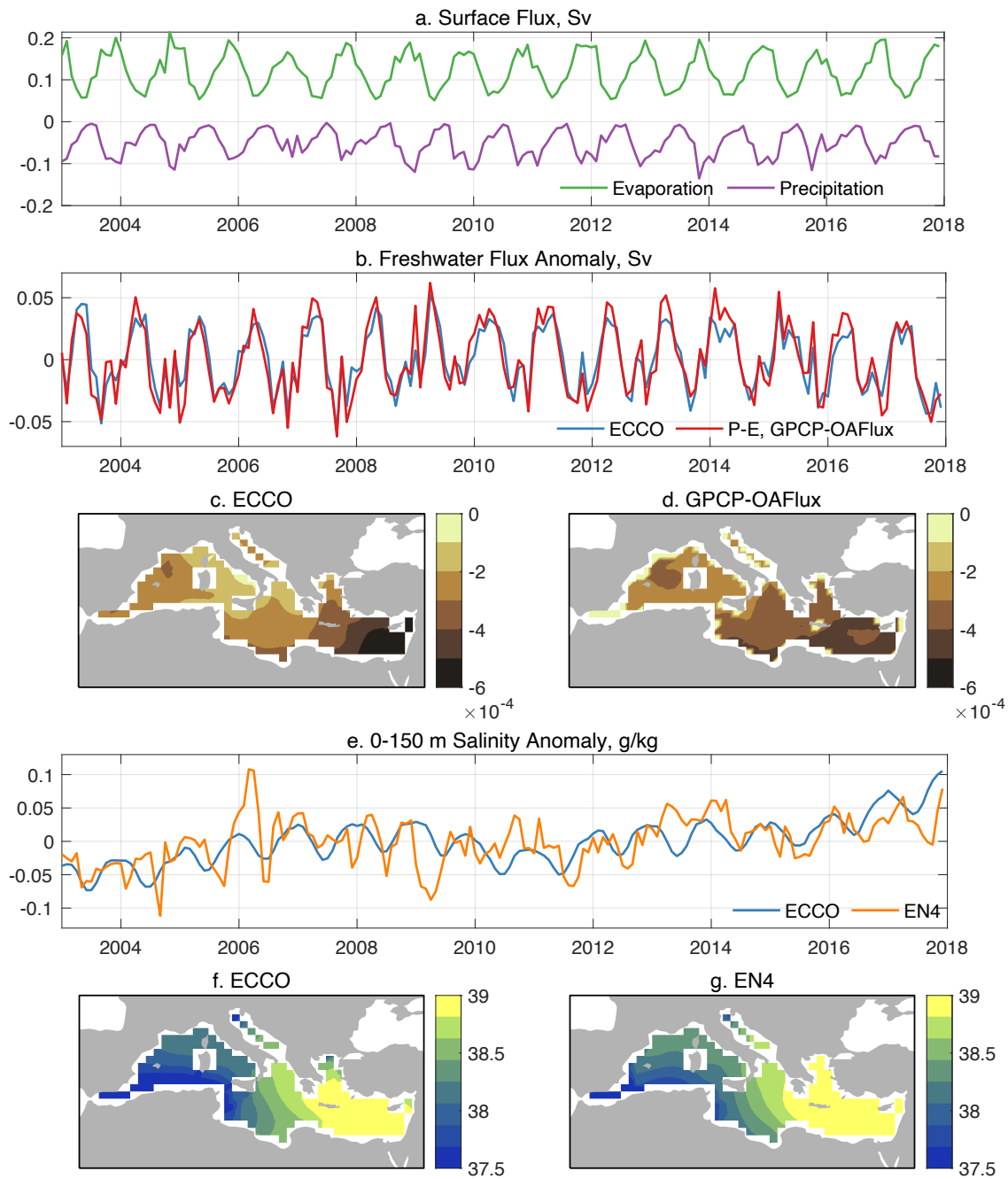
110 Figure 2 Timeseries and time-mean spatial patterns of freshwater flux and mean salinity (0–150 m) in the Mediterranean Sea, comparing ECCO outputs with other datasets. (a) timeseries of total evaporation and precipitation from ECCO; (b) timeseries of freshwater flux anomaly from ECCO and the reference flux derived from GPCP and OAFlux; (c&d) spatial patterns of surface freshwater flux; (e) timeseries of salinity anomaly from ECCO and EN4; (f&g) spatial patterns of salinity. All data are interpolated onto the ECCO grid.
