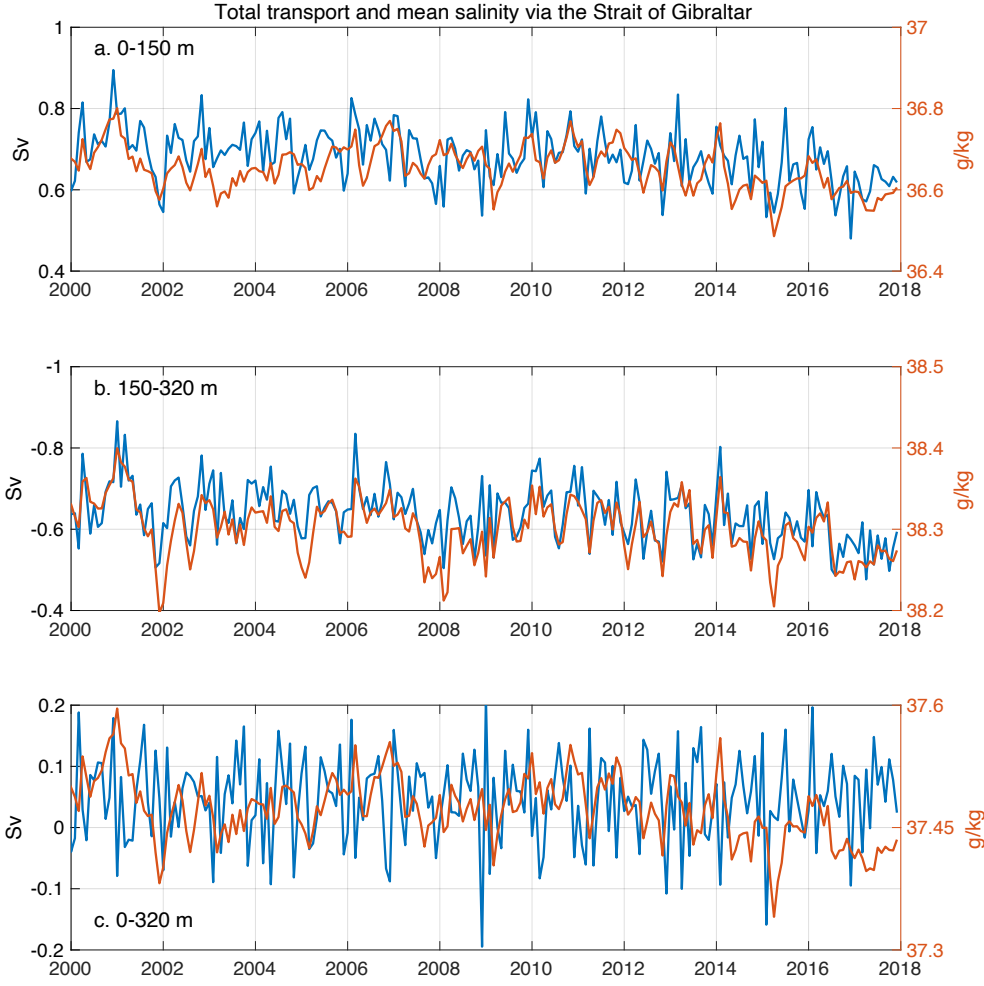
160 Figure 3 Net flux (blue, left axis) and mean salinity (red, right axis) at the Strait of Gibraltar. positive transport means eastward transport into the Mediterranean Sea. Notice the y-axis in panel (b) is inverted.
